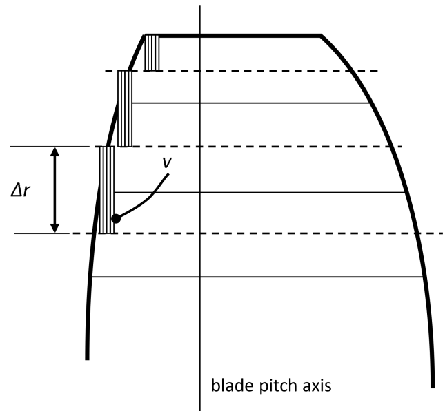
Figure 6. A sketch illustrating the parameters used to evaluate the eroded volume of a generic span-wise element. \Delta r represents the span-wise dimension of a generic element, and v denotes the eroded volume from that element.
