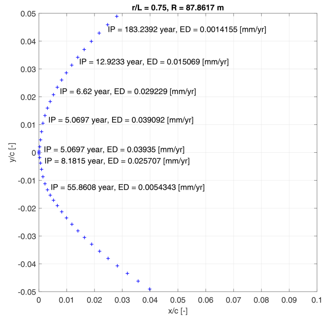
Figure 8. The figure illustrates the discretization of chord-wise elements of a blade profile located at 75 % blade length from the blade root. For certain elements, the incubation period, IP, and the yearly accumulated erosion depth, ED, are shown. r/L represents the relative position of the profile along the blade length, while R denotes the radial distance of the airfoil from the blade root. x/c and y/c are the airfoil coordinates, non-dimensional using the local chord length.
