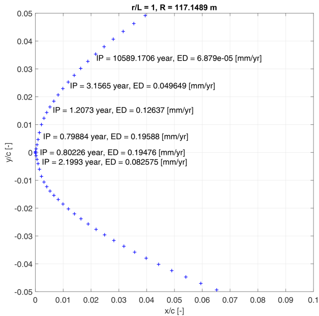
Figure 7. The figure illustrates the discretization of chord-wise elements of the tip airfoil. For certain elements, the incubation period, IP, and the yearly accumulated erosion depth, ED, are shown. r/L represents the relative position of the profile along the blade length, while R denotes the radial distance of the airfoil from the blade root. x/c and y/c are the airfoil coordinates, non-dimensional using the local chord length.
