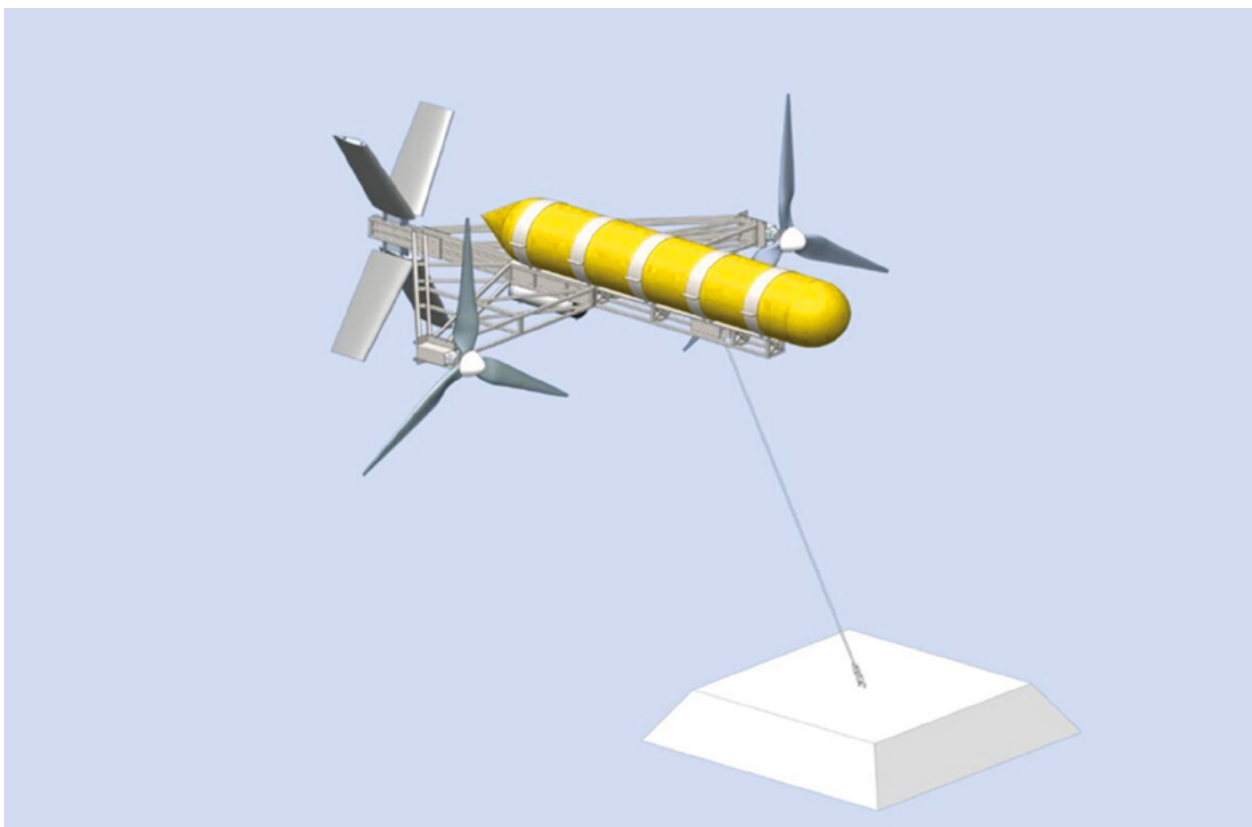
The functioning of the Multi Energy Compensator System
