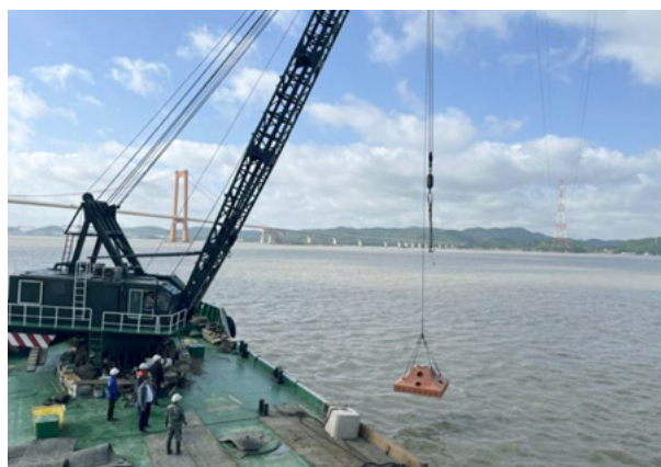
Deployment of test equipment in Zhoushan test site
