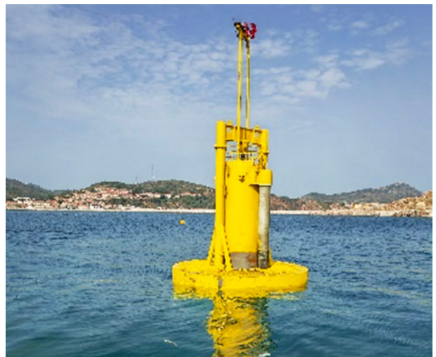
Shandong University wave energy device in sea trial
