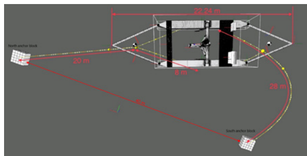
Figure 2: Blind Channel Tidal berth design
