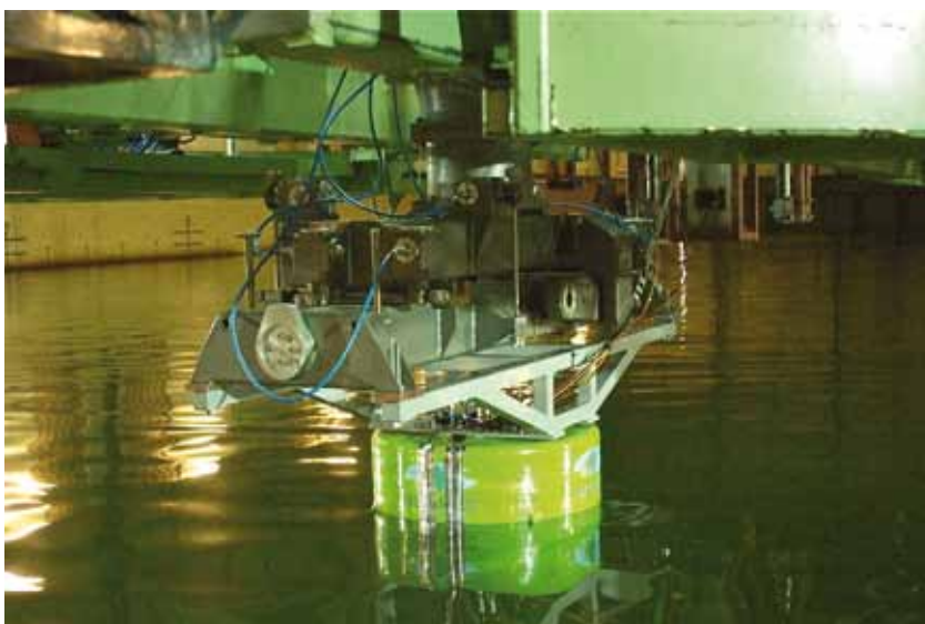
▲ Tank testing of OCEANTEC wave energy device
