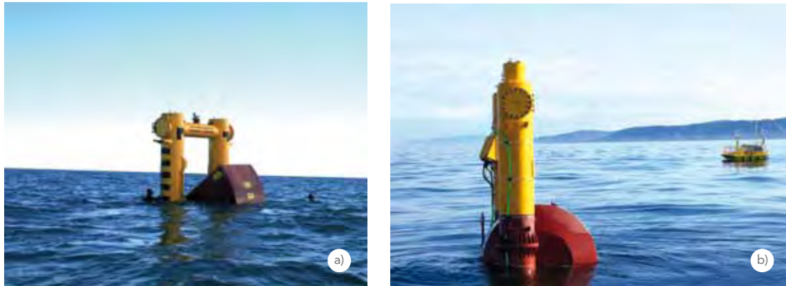
FIGURE 1: a) WET-NZ's MEDF device off Akaroa Heads (2011) and b) its US device at the NNMREC test site, Oregon (August 2012)
