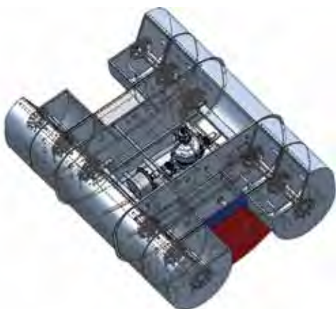
▲ ISWEC drawing and scaled prototype in testing site
