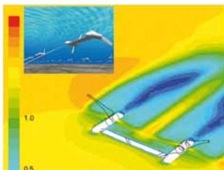
◀ Simulation of the ocean current power generation (IHI, Toshiba, Mitsui Global Strategic Studies Institute, University of Tokyo)
