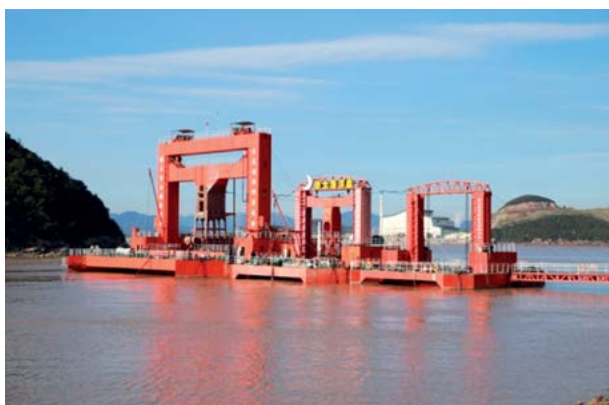
ZJU Tidal Current Energy Demonstration Platform
