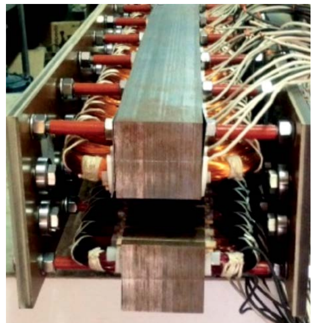
The IMPETUS prototype
