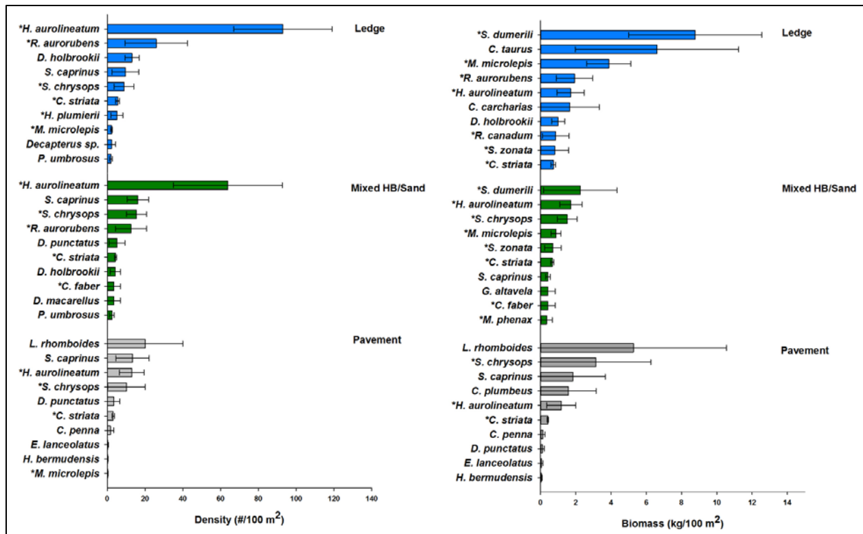
Figure 3-60. The top ten species of the conspicuous community's mean density ( \#/100\text{ m}^2 ) and mean biomass ( \text{kg}/100\text{ m}^2 ) by natural hardbottom type: Ledge, Mixed HB/Sand, and Pavement. The asterisk (*) denotes a member of the Snapper Grouper Management Complex managed by the SAFMC.
