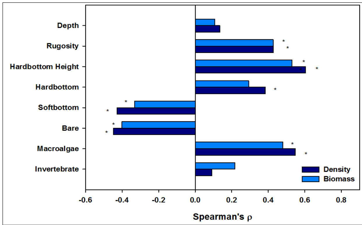
Figure 3-72. Large Fish (50 cm TL) mean site density and biomass Spearman rank correlations by depth (m), multi-beam derived rugosity, hardbottom height (cm), and percent cover: hardbottom, softbottom, macroalgae, and invertebrates. * indicates significance probability where \alpha < 0.05 .
