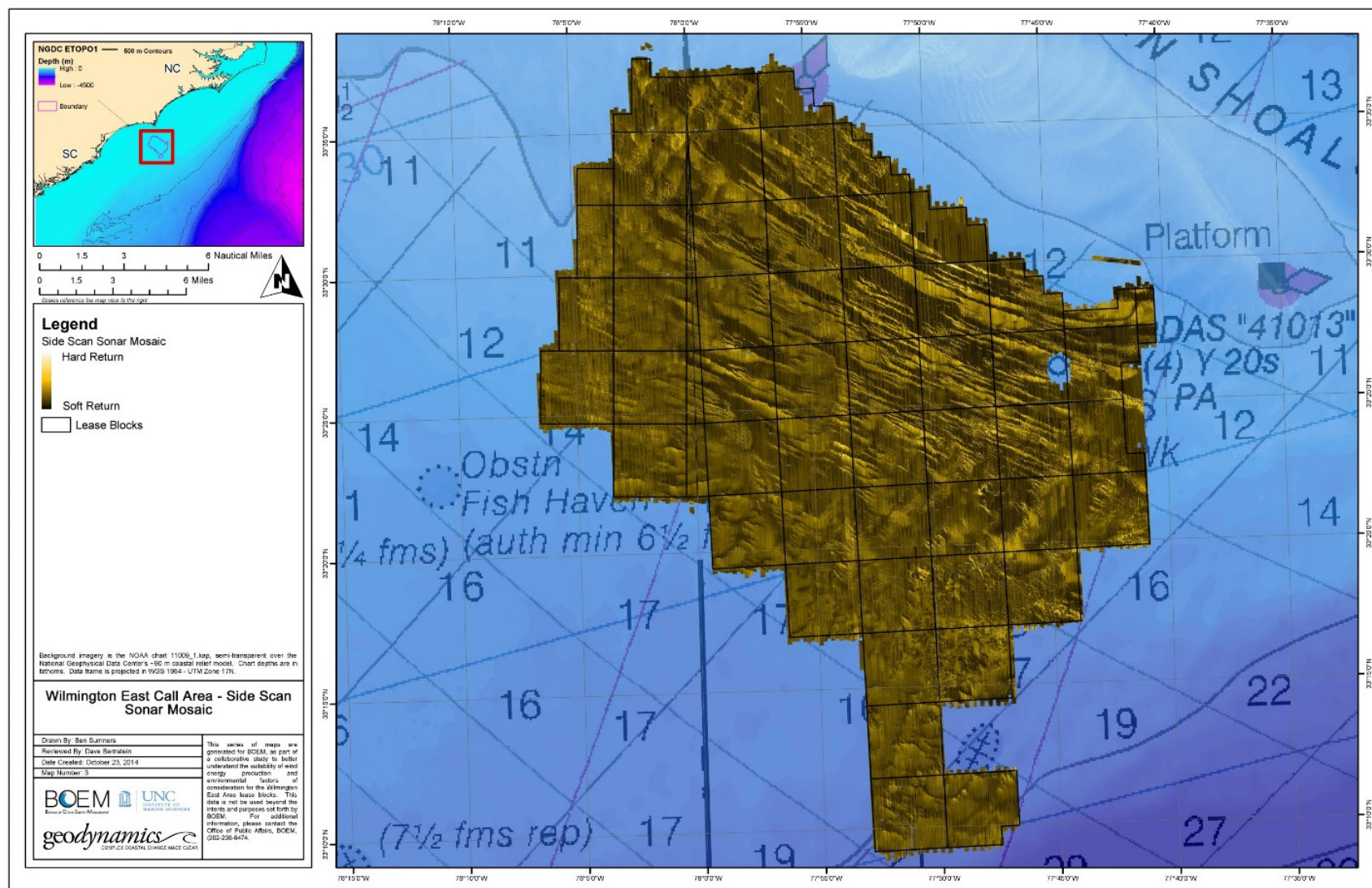
Figure 3-3. Results of the sidescan sonar mosaic, overlaid by OCS lease blocks.
