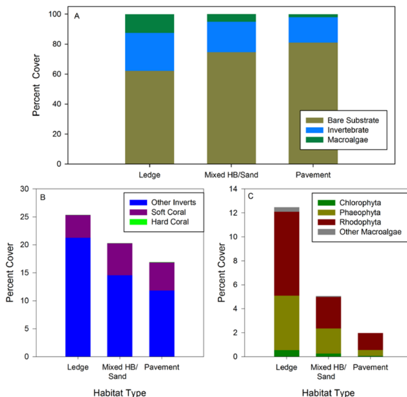
Figure 3-56. Percent cover for broad taxonomic groups (A), invertebrates only (B), and macroalgae only (C) by habitat type.
