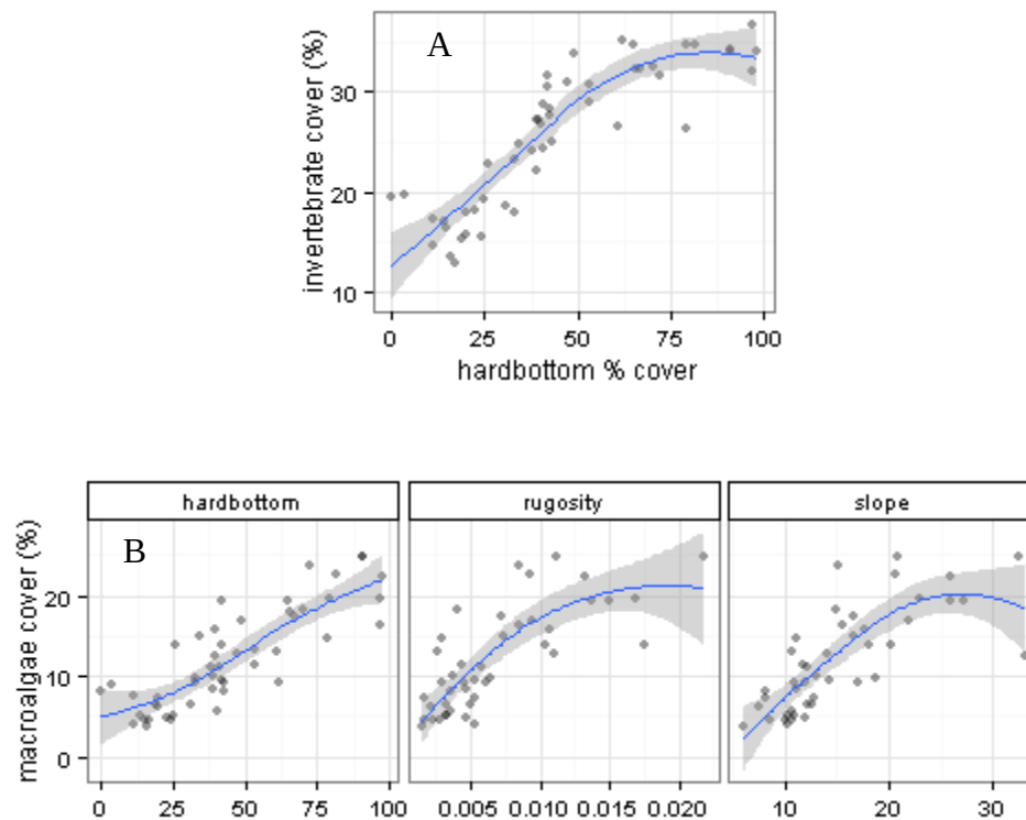
Figure 3-51. A. Partial dependence plot showing cover of invertebrates, including hard corals, soft corals, and sponges, as related to hardbottom cover (%). B. Partial dependence plots showing cover of macroalgae as related to hardbottom cover (%), multibeam derived rugosity (5 cell resolution), and slope (m). Line indicates smoothed fit, gray is confidence band.
