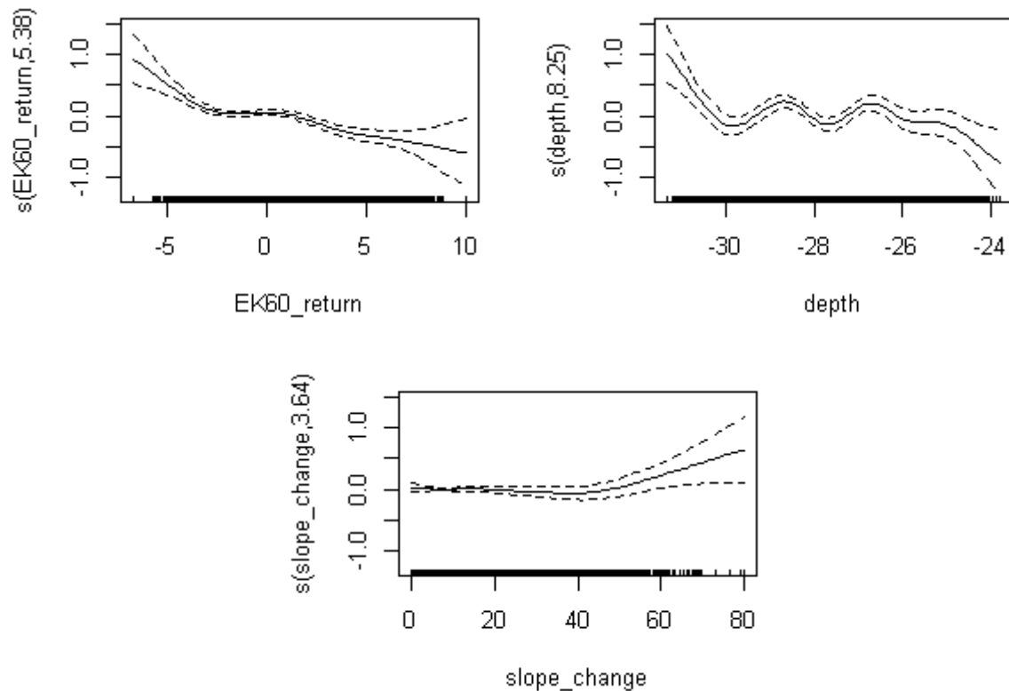
Figure 3-41. Smoothed relationships (y-axis) between SBES fish in the medium size class with environmental variables for the combined North and South survey areas.
