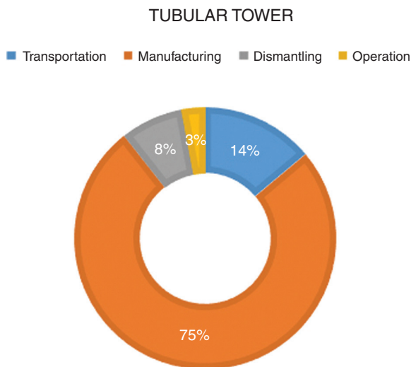
Fig. 5 Distribution of CO 2 emissions per life stage for the lattice tower
