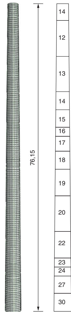
Fig. 1 Tubular-tower shell-thickness distribution
