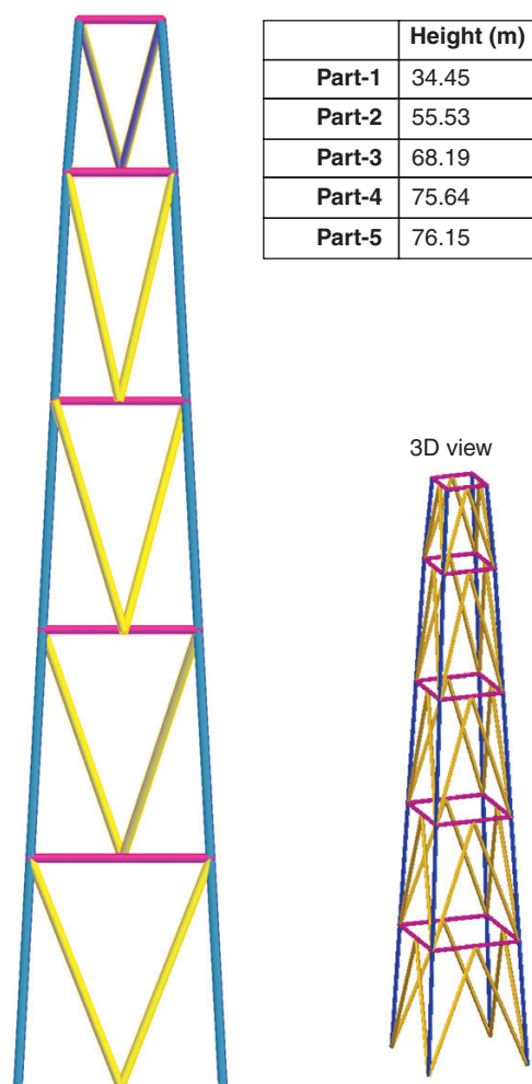
Fig. 2 Lattice-tower configuration
