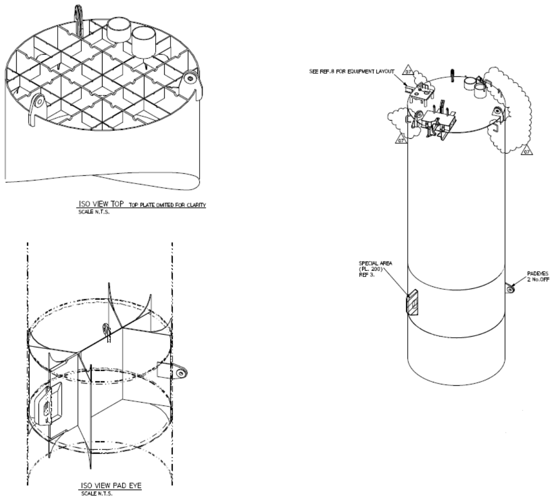
Figure 4-2: ISO view of suction anchors, including stiffeners
