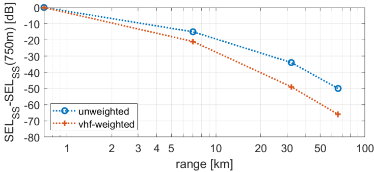
Figure 6 Decay of unweighted and weighted broadband SEL_{SS} (with varying frequency bandwidth, see Figure 5) with range as measured during piling for the Gemini wind farm (pile U8), relative to the values measured at 0.7 km.
