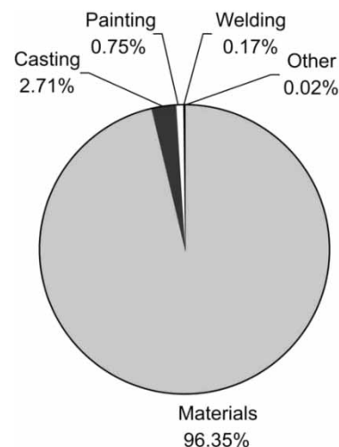
Fig. 8 Breakdown of embodied energy in structural manufacture
