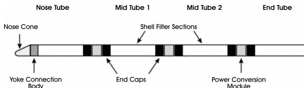
Fig. 5 Structural elements of the Pelamis
