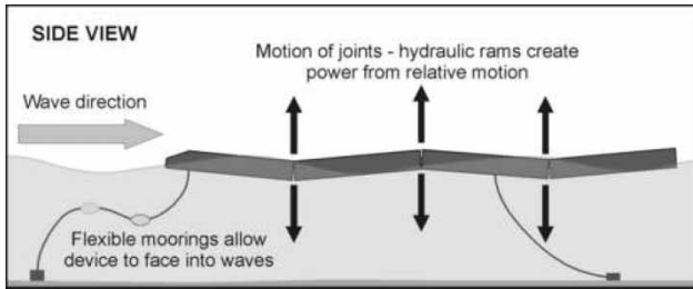
Fig. 3 Side view of the Pelamis (adapted from reference [16])
