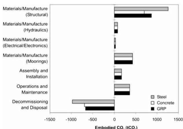
Fig. 12 Comparison of embodied CO 2 with alternative materials
