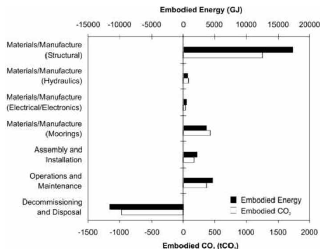
Fig. 9 Embodied energy by life cycle stage
