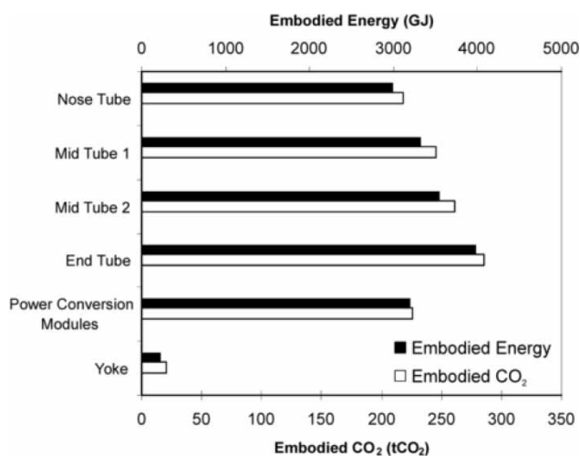
Fig. 7 Structural embodied energy and CO 2
