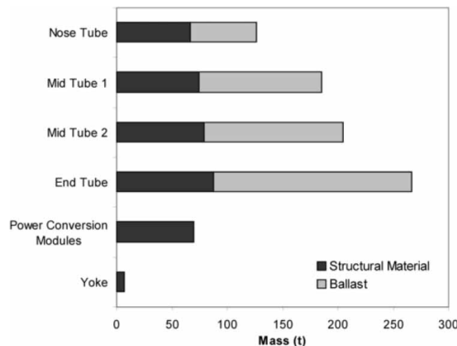
Fig. 6 Mass of structural elements
