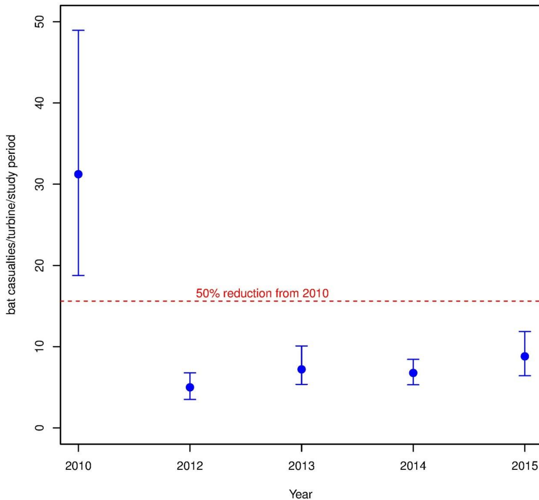
Figure 7. A comparison of estimate bat casualty rates and 90% confidence intervals for Fowler Ridge Wind Farm. The 2010 estimate represents turbine operating at manufacturer cut-in speeds. The 2012, 2013, 2014, and 2015 estimates represent data collected at turbines that were feathered below 5.0 m/s. The red dotted line represents a 50% reduction in bat casualty rates compared to the 2010 point estimate.
