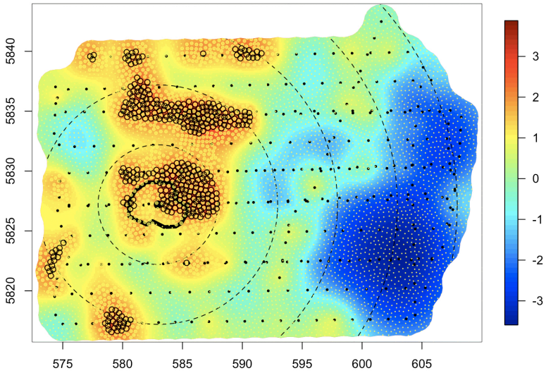
Figure 12. As Figure 9. Black dots refer to the exclusion set for the positive values. At these locations the joint probability that the w_j values are positive and important is at least 0.90.
