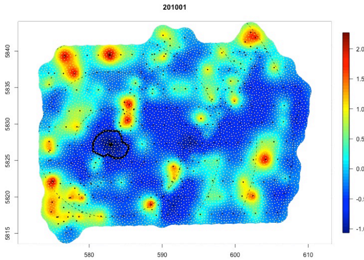
Figure 22. Results for the January 2010 survey.
