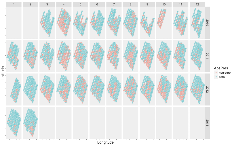
Figure 33. Spatial position of sampling locations by year and month for the Robin Rigg wind farm. A green dot means that zero birds were observed whereas a red dot indicates that the count was larger than 0.
