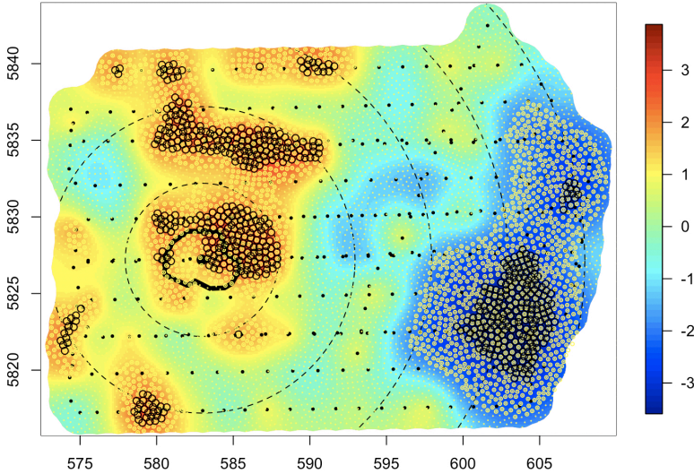
Figure 13. As Figure 9 to Figure 12. The yellow dots within the blue areas refer to points where we have an important reduction of the spatial random field. The black dots within the blue areas form the exclusion set for the negative values.
