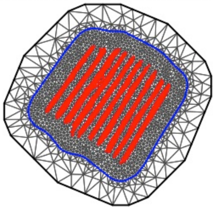
Figure 34. The mesh used by the spatial ZIP model. The mesh has 2023 vertices. The mesh has an inner part (with a finer resolution) and also an outer part to avoid numerical problems due to the boundary.
