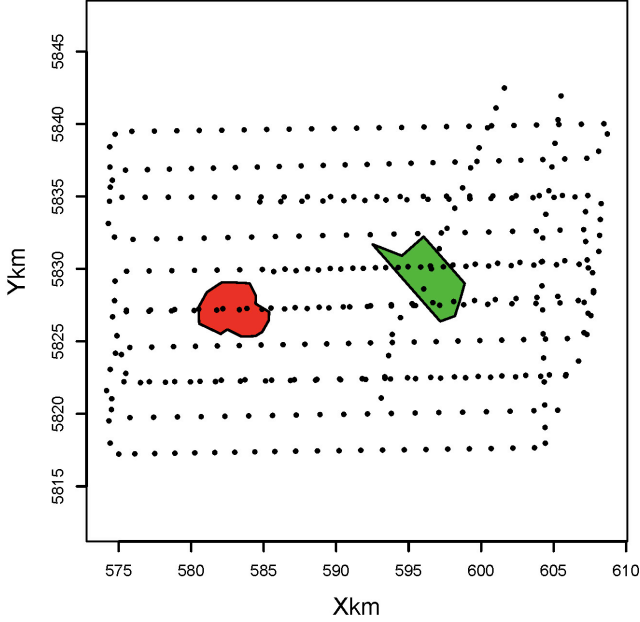
Figure 3. Sampling locations for the survey made in November 2003. The area covered by the PAWP wind park is plotted as a red polygon and the green area is the OWEZ wind park.
