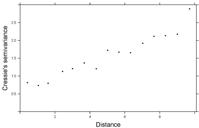
Figure 6. Variogram of Pearson residuals obtained by the Poisson GLM in Equation (3.1).
