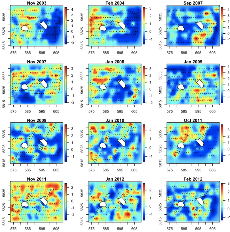
Figure 5. Spatial random fields obtained by the Poisson GLM with spatial-temporal correlation applied on the combined data of the OWEZ and PAWP wind parks. Red values correspond to areas with higher abundances and blue values to areas with lower abundances.
