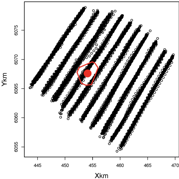
Figure 31. Spatial position of sampling locations for the Robin Rigg wind farm. The red lines represents the outer turbines.
