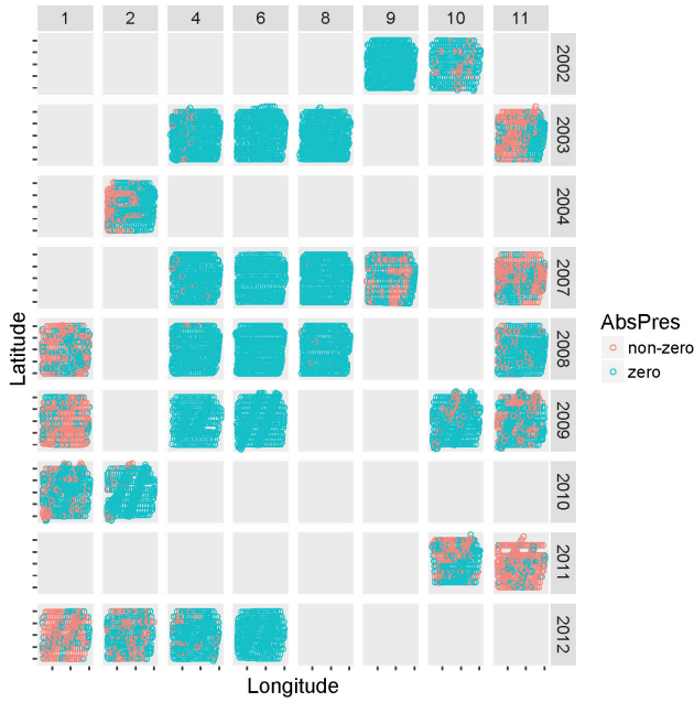
Figure 2. Spatial position of sampling locations by year and month for PAWP and OWEZ. A green dot means that zero birds were observed whereas a red dot indicates that the count was larger than 0.
