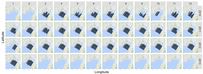
Figure 32. Spatial position of sampling locations by year and month for the Robin Rigg wind farm.
