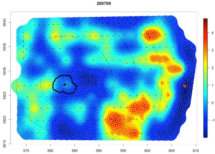
Figure 17. Results for the September 2007 survey.
