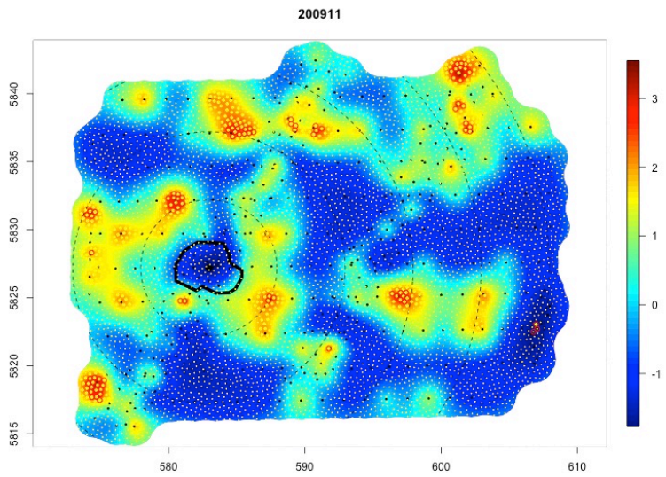
Figure 21. Results for the November 2009 survey.
