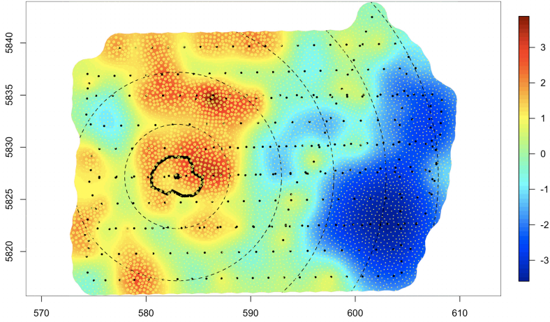
Figure 11. As Figure 9. Yellow dots within the red areas refer to locations where the w_j is positive and important.
