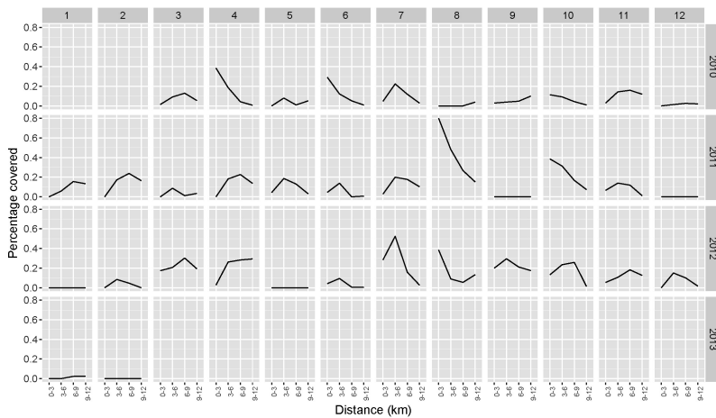
Figure 36. Percentage of coverage of positive (and important) values of the spatial random field per distance band for the marginal probabilities for Robin Rigg for each month and year. Results are obtained with a ZIP GLM with spatial correlation.
