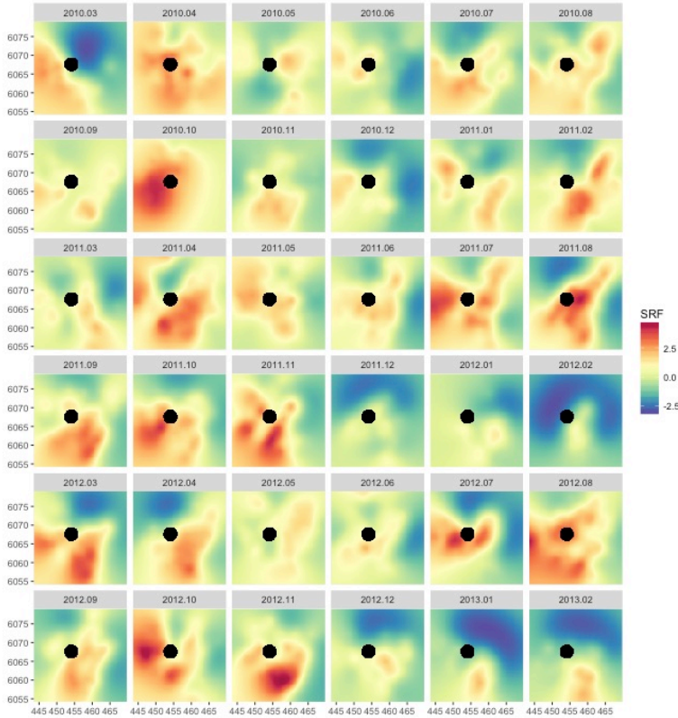
Figure 35. Spatial random fields obtained by the NB GLMM with spatial-temporal replicate correlation applied on Robin Rigg data. Red values correspond to areas with higher abundances and blue values to areas with lower abundances. To obtain the fitted values of the model we have to (i) add the intercept, sampling area effect, random effect survey and the spatial random fields, and then (ii) the exponential function has to be applied. This model does not use time knots.
