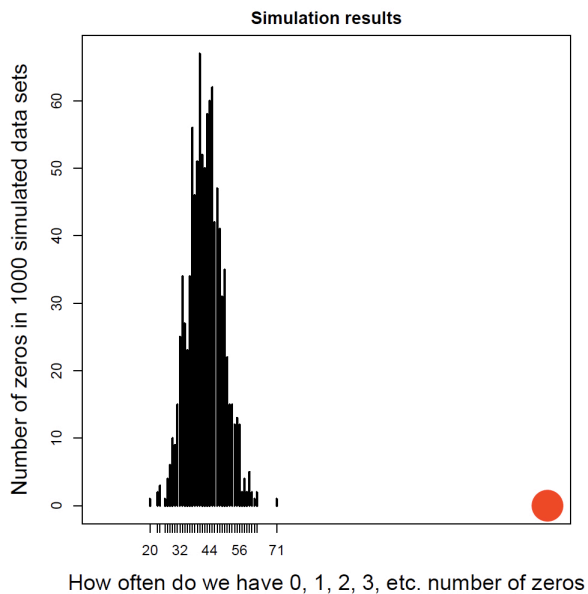
Figure 7. Results of simulation study. The red dot represents the number of zeros in the observed data in survey from November 2003. The frequency plot (black lines) are based on the number of zeros in 1,000 simulated data sets.
