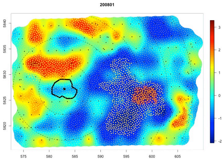
Figure 19. Results for the January 2008 survey.
