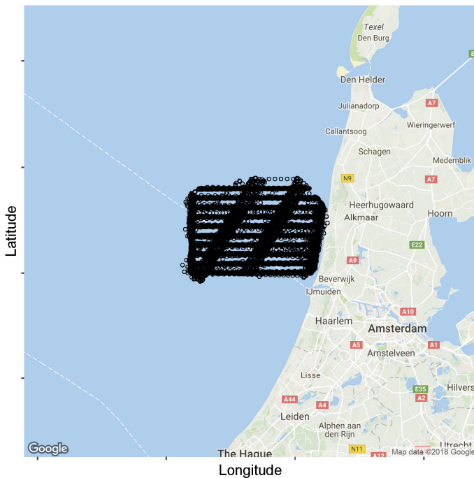
Figure 1. Spatial position of sampling locations for the offshore PAWP and OWEZ wind farms.
