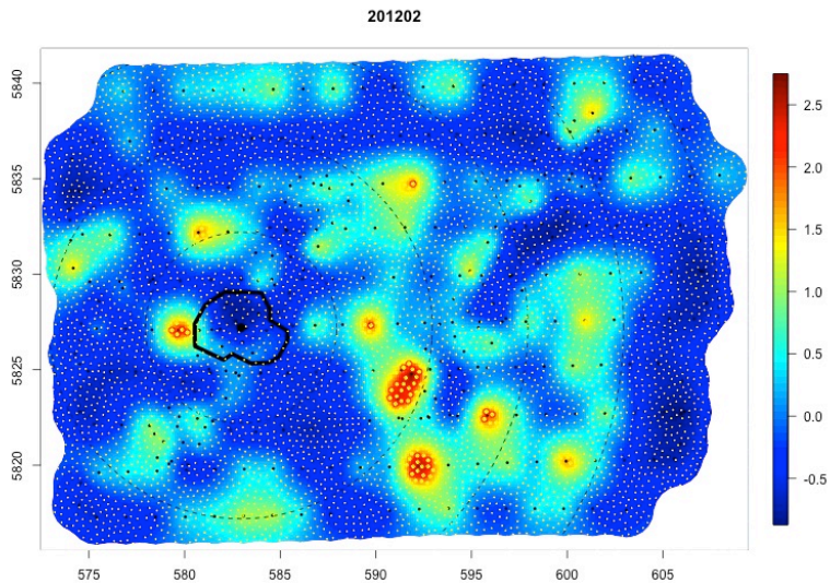
Figure 26. Results for the February 2012 survey.
