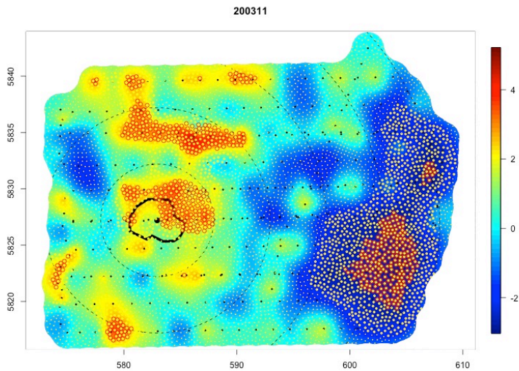
Figure 15. Results for the November 2003 survey.
