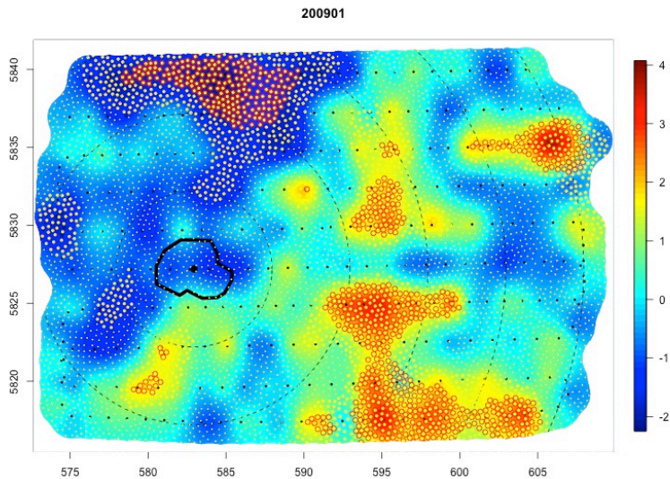
Figure 20. Results for the January 2009 survey.
