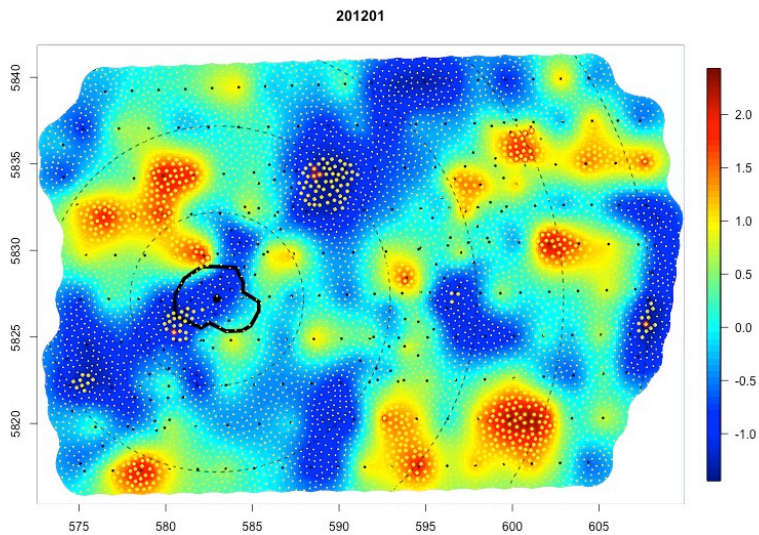
Figure 25. Results for the January 2012 survey.
