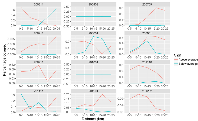
Figure 28. Percentage of coverage per distance band for the marginal probabilities for PAWP.
