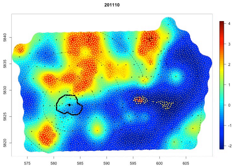
Figure 23. Results for the October 2011 survey.
