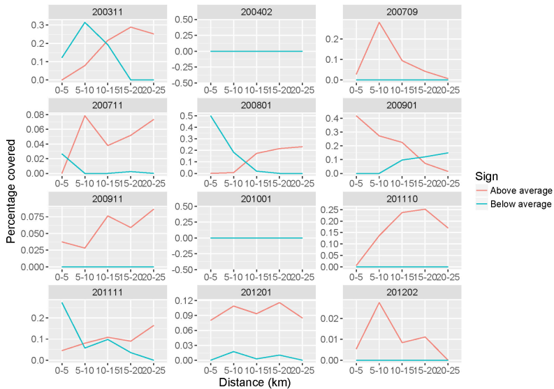
Figure 29. Percentage of coverage per distance band for the marginal probabilities for OWEZ.
