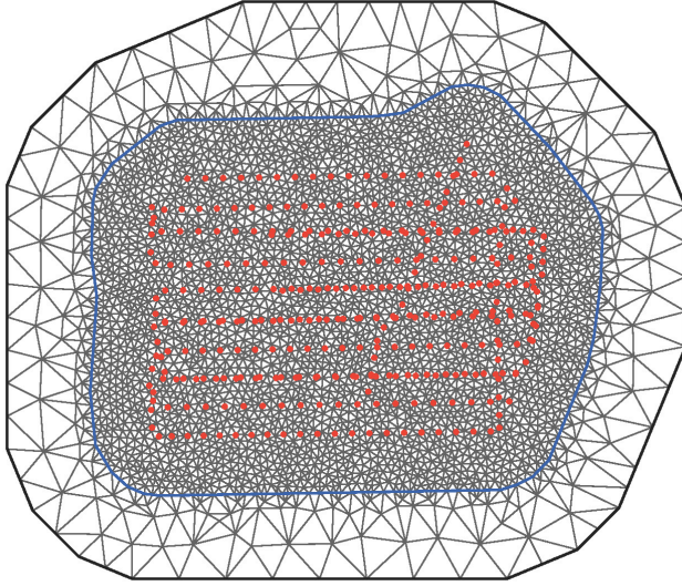
Figure 4. The mesh used by the spatial ZIP model. The mesh has 3715 vertices. The mesh has an inner part (fine mesh) and also an outer part to avoid numerical problems due to the boundary.
