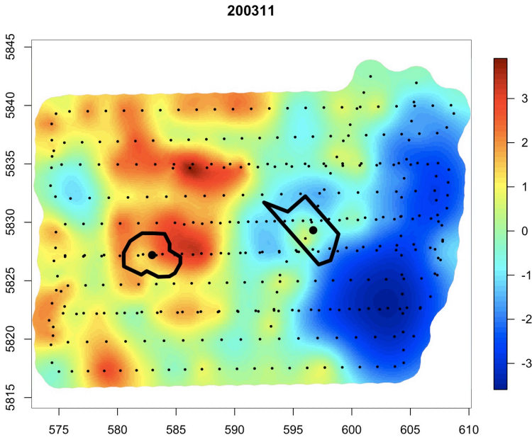
Figure 8. Spatial random field obtained by the spatial ZIP model applied on the survey data from November 2003. The coordinates are UTM coordinates.
