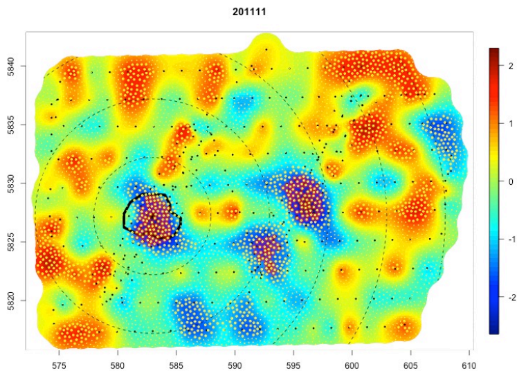
Figure 24. Results for the November 2011 survey.
