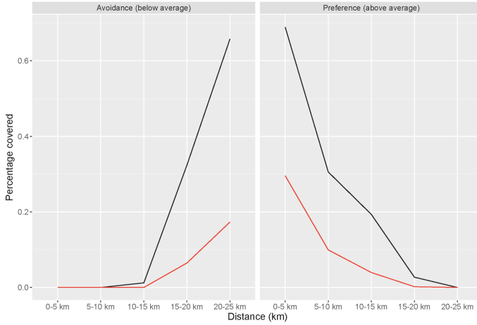
Figure 14. Percentages of important nodes in each distance band for PAWP. The black lines are for the marginal probabilities and the red lines are for the joint probabilities. The left panel is for the negative values (blue areas in Figure 9) and the right panel is for the positive values (red areas in Figure 9).
