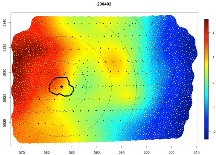
Figure 16. Results for the February 2004 survey.
