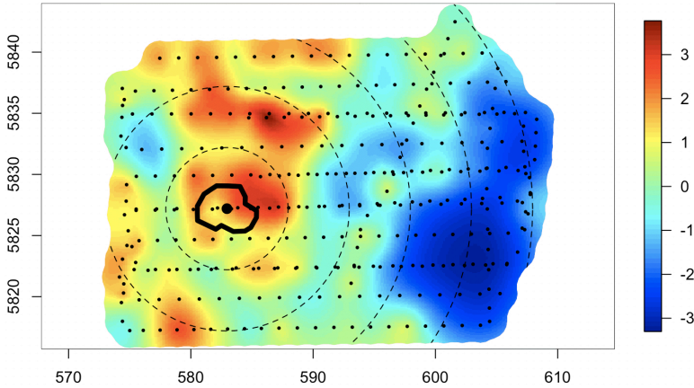
Figure 9. Spatial random field obtained by the spatial ZIP model. Circles with a radius of 5 km, 10 km, 15 km, etc. around the centre of PAWP have been added.
