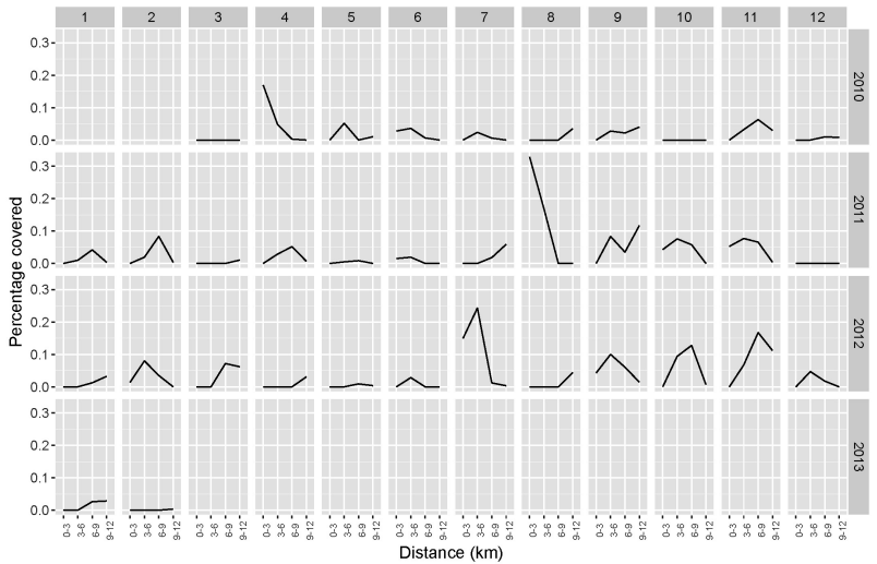
Figure 37. Percentage of coverage per distance band for the marginal probabilities for Robin Rigg. Results are obtained with a NB GLM with spatial correlation.
