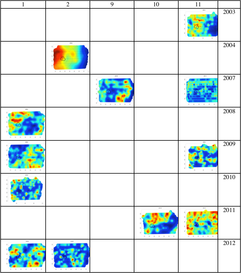
Figure 27. Results for all surveys. The colour red corresponds to above average values and blue to below average values.
