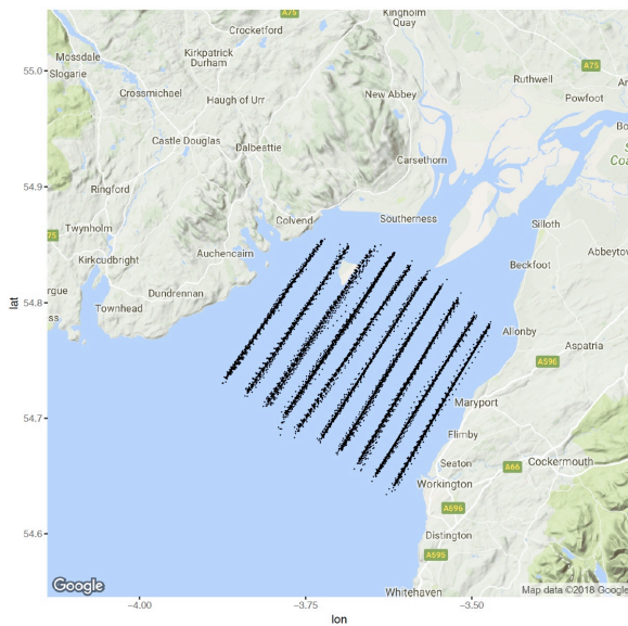
Figure 30. Spatial position of sampling locations for the Robin Rigg wind farm.
