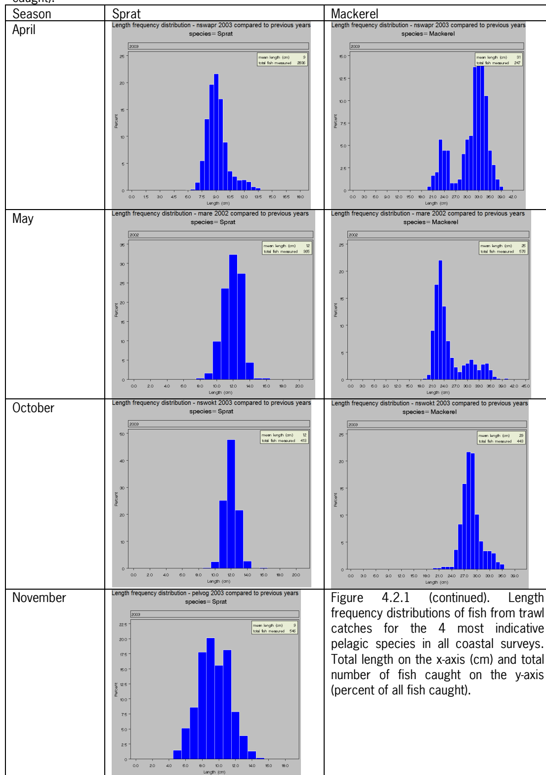
Figure 4.2.1. Length frequency distributions of fish from trawl catches for the 4 most indicative pelagic species in all coastal surveys. Total length on the x-axis (cm) and total number of fish caught on the y-axis (percent of all fish caught).
