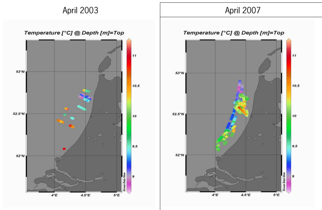
Figure 3.3.1. Temperature distributions in April 2003 (left panel) and April 2007 (right panel). High temporal variation can be observed in the raw data points particularly around the windfarm in April 2007
