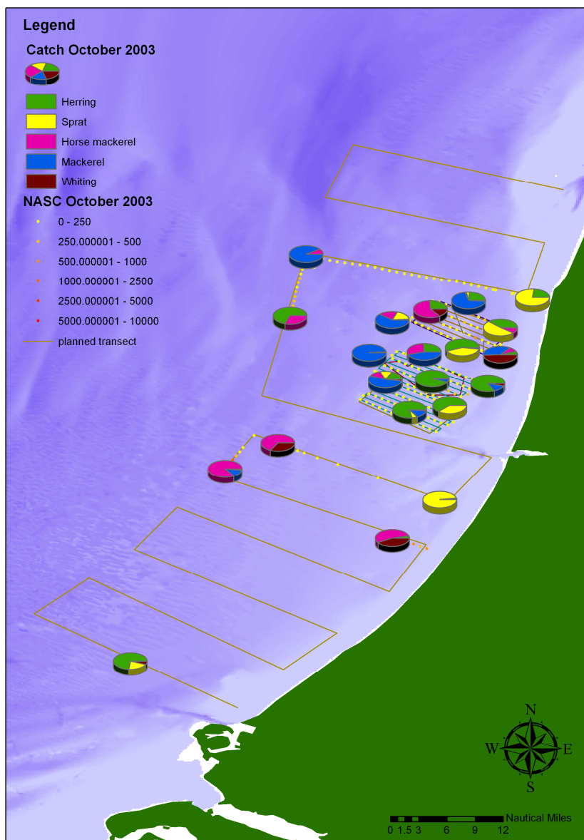
Figure 2.1.1. Catch composition of pelagic fish in the T0-October survey showing a high species diversity but low acoustic abundances of the main species: herring and sprat.
