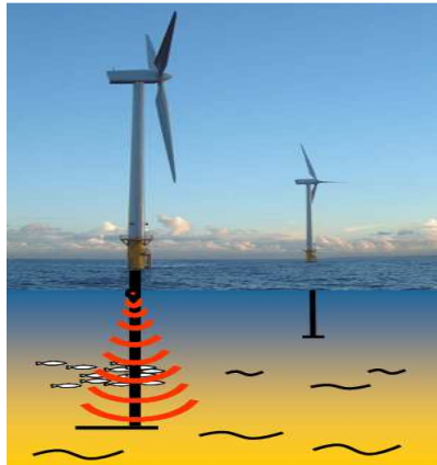
Figure 2.2. A schematic presentation of increased fish concentrations near individual turbines and how a high resolution setup can reveal pelagic fish schools near a wind turbine
