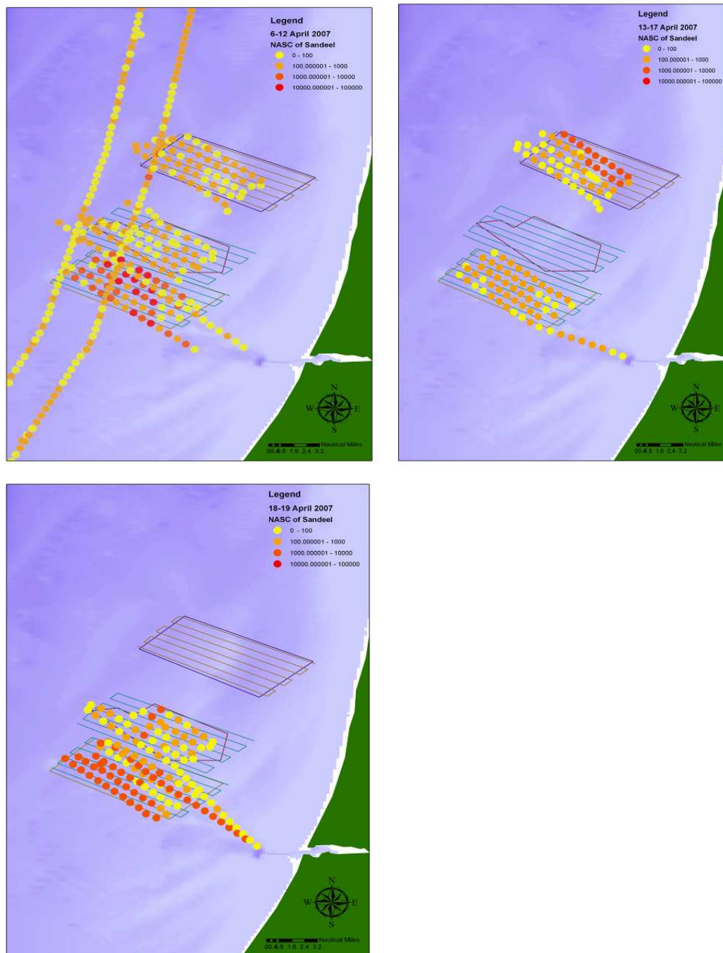
Figure 3.2.4. Weekly acoustic densities on the cruise track of sandeel species in the T1 survey indicating high temporal variations in abundance. Note: acoustic positions show a small deviation which needs to be corrected.
