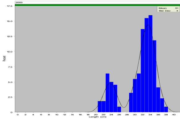
Figure 4.1.2. Length frequency distributions of fish from trawl catches for the 7 most common pelagic species in both T0 and T1 surveys. Total length on the x-axis (cm) and total number of fish caught on the y-axis (percent of all fish caught). The green bar indicated the relative amount of fish used for a frequency distribution.
