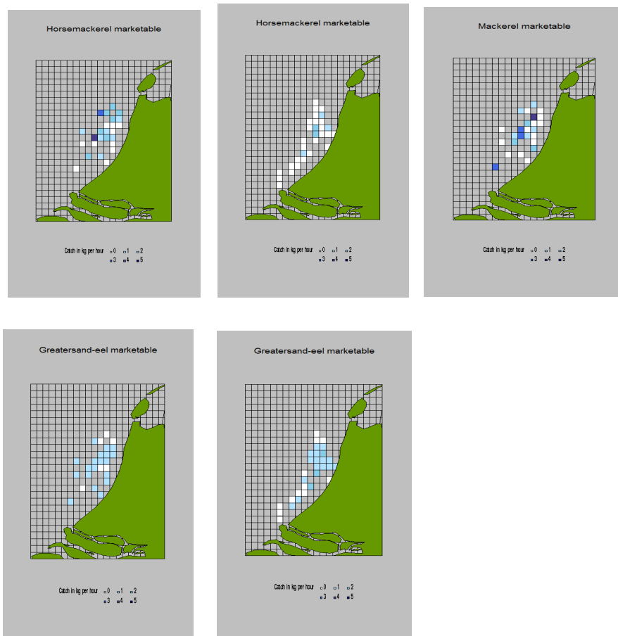
Figure 4.2.2. Spatial distribution of the most common pelagic species based on trawl catches in 10log (kg/hour) fishing.
