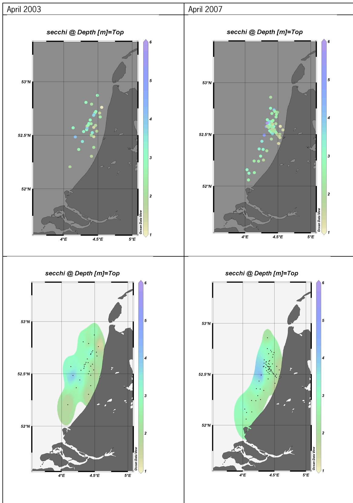
Figure 3.3.3. Comparison between water clarity distribution as recorded by Secchi observations in April 2003 (left panel) and April 2007 (right panel).
