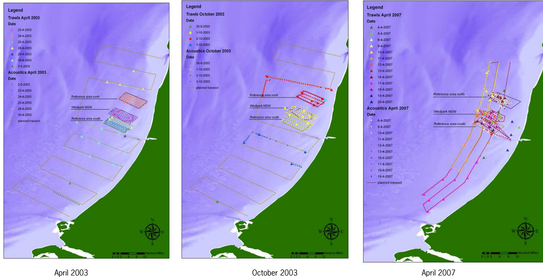
Figure 2.1: Temporal progression of both T0 and T1 surveys based on trawl catches and acoustic samples. The OWEZ area (middle rectangle) and neighbouring reference areas are indicated.
