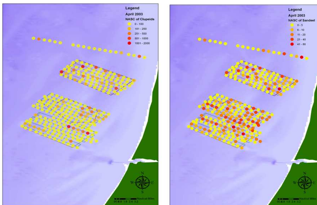
Figure 3.2.3. Mean acoustic densities on the cruise track of both clupeids and sandeel species in the T0 survey indicating high local variation.
