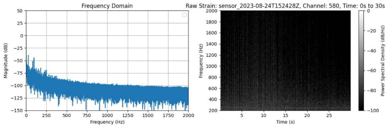
(2) Boat stationed at dock, engine on; cable in spool inside boat.
