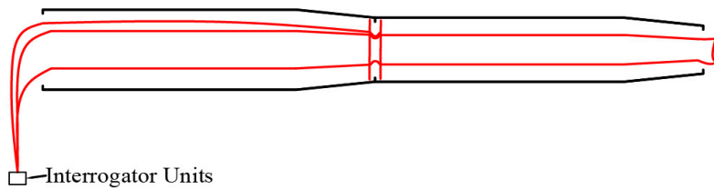
Figure 1: Fiber-Optic Installation Layout (in Red) for the 4-Point Bend Test (Side View)
