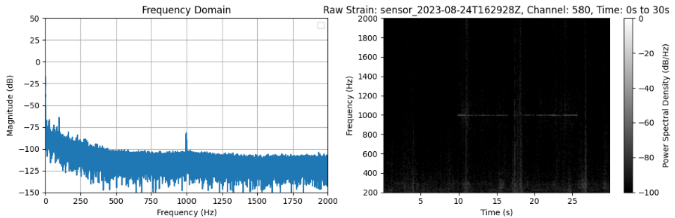
(3) Boat at destination point, engine on; cable in spool inside boat; speaking playing 1,000 Hz near cable.
