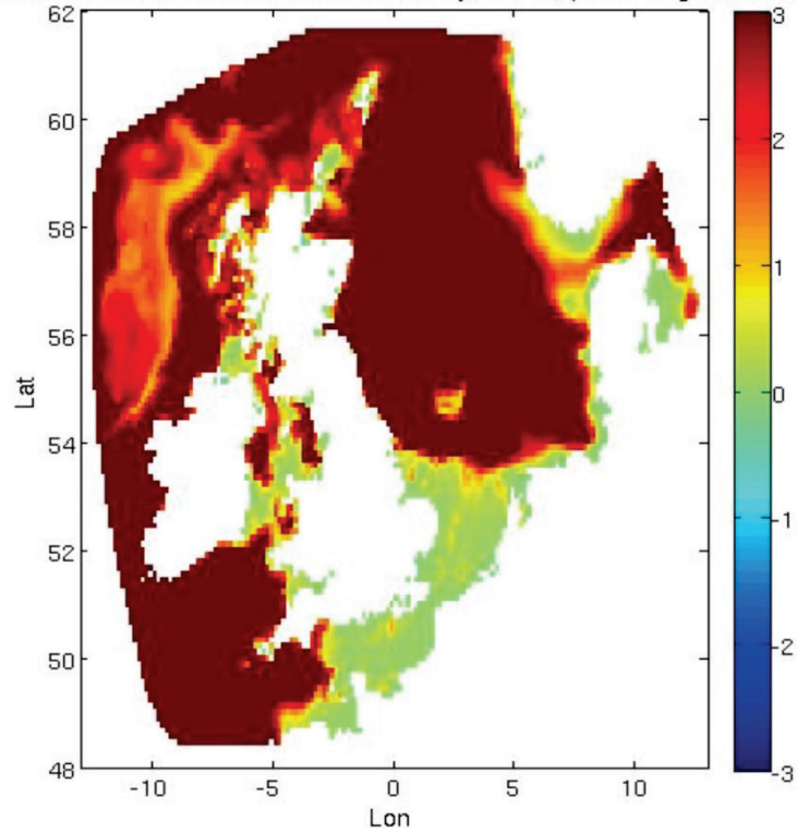
FVCOM surface T minus FVCOM bottom T at june15th, (Units: Degrees Celcius)
