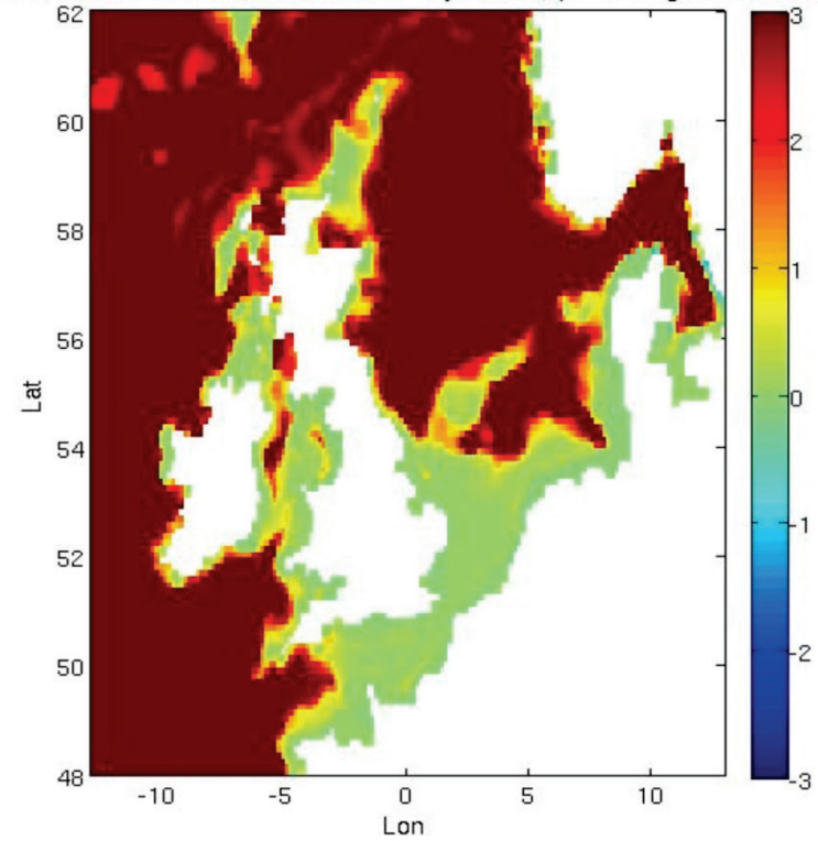
AMM surface T minus AMM bottom T at june15th, (Units: Degrees Celcius)
