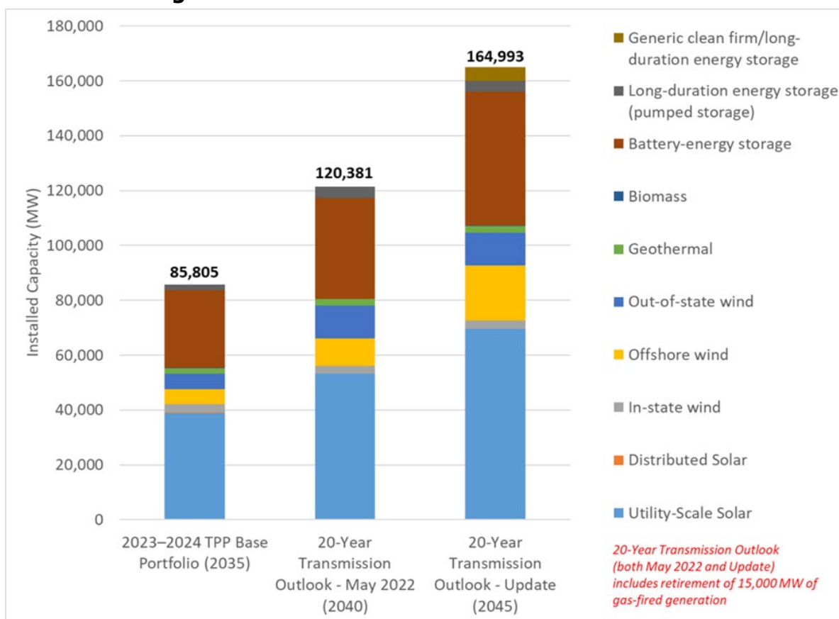
Figure 1-1: Resource Portfolios for 2035 to 2045
