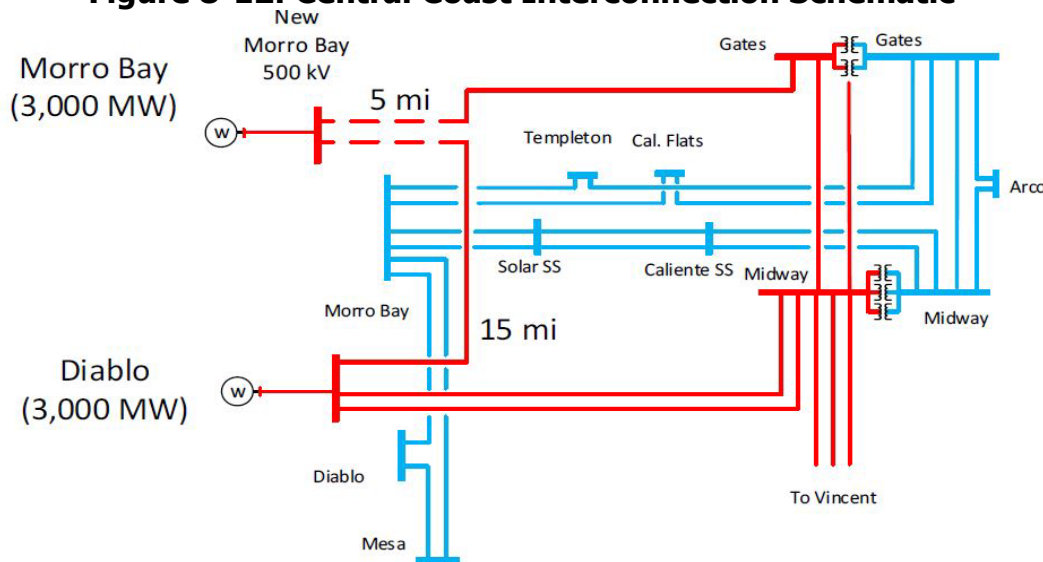
Figure 8-12: Central Coast Interconnection Schematic
