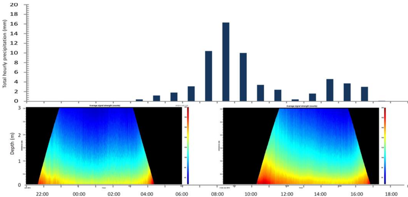
Figure 32 : Influence of precipitation on suspended sediment concentration (represented as backscatter intensity from the ADCP) from 21:00 June 7 to 19:00 June 8th during Post-tropical storm Andrea.
