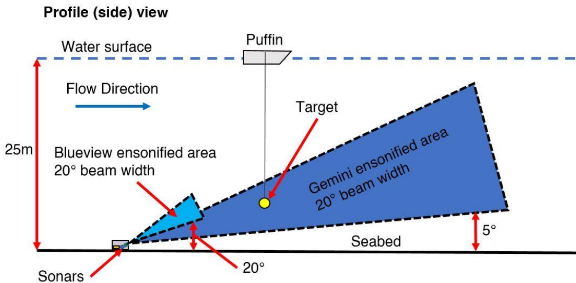
Figure 2.1.4: Grand Passage experiment schematic - profile view - Deployment 1
