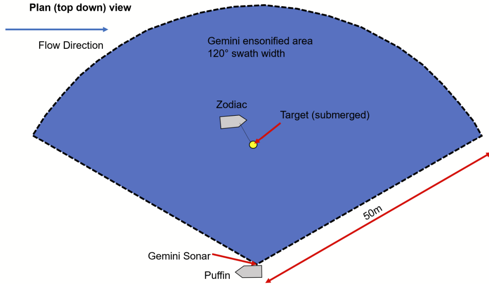
Figure 2.1.12: Minas Passage experiment schematic - plan view
