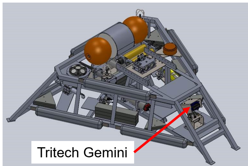
Figure 4.2: Pathway Monitoring Platform with Tritech Gemini mounted in the pan and tilt module on the bottom right.
