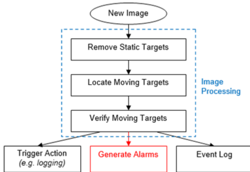
Figure 2.3.1: SeaTec image processing flow.
