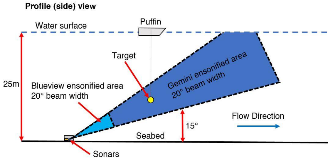
Figure 2.1.5: Grand Passage experiment schematic - profile view - Deployment 2
