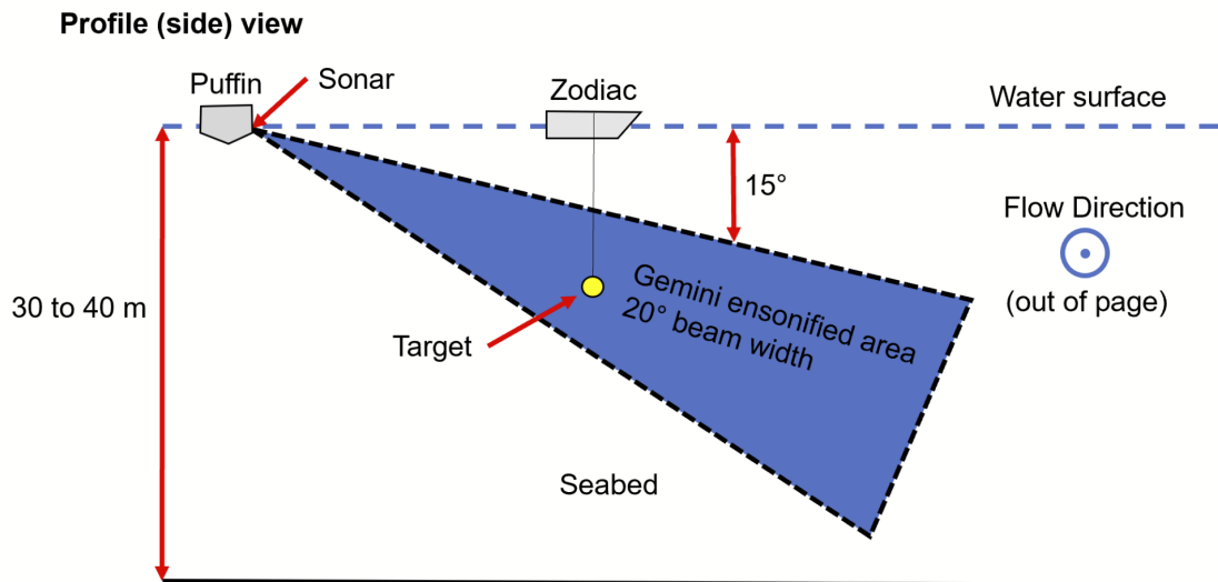
Figure 2.1.13: Minas Passage experiment schematic - profile view
