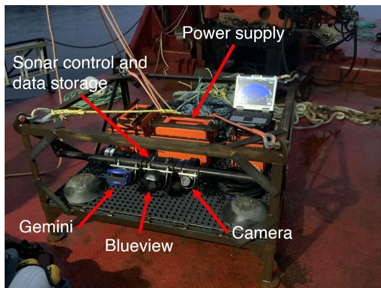
Figure 2.1.1: Autonomous Multibeam Imaging Sonar (AMIS) monitoring system
