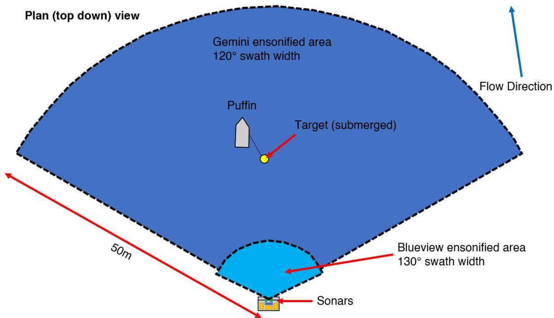
Figure 2.1.3: Grand Passage experiment schematic - plan view
