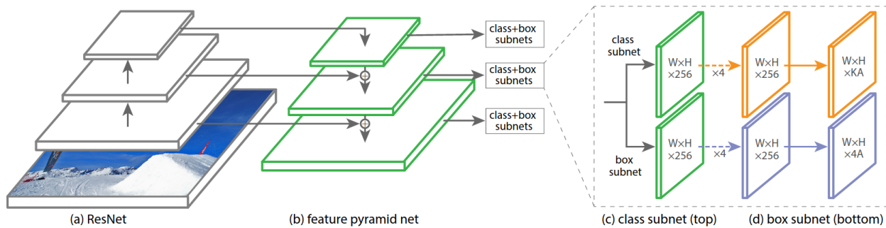
Fig 2.3.2: RetinaNet architecture, presented by (Lin 2017a). Original text: The one-stage RetinaNet network architecture uses a Feature Pyramid Network (FPN) (Lin 2017b) backbone on top of a feedforward ResNet architecture (Huang 2017)(a) to generate a rich, multi-scale convolutional feature pyramid (b). To this backbone RetinaNet attaches two subnetworks, one for classifying anchor boxes (c) and one for regressing from anchor boxes to ground-truth object boxes (d). The network design is intentionally simple, which enables this work to focus on a novel focal loss function that eliminates the accuracy gap between our one-stage detector and state-of-the-art two-stage detectors like Faster R-CNN with FPN (Lin 2017b) while running at faster speeds.
