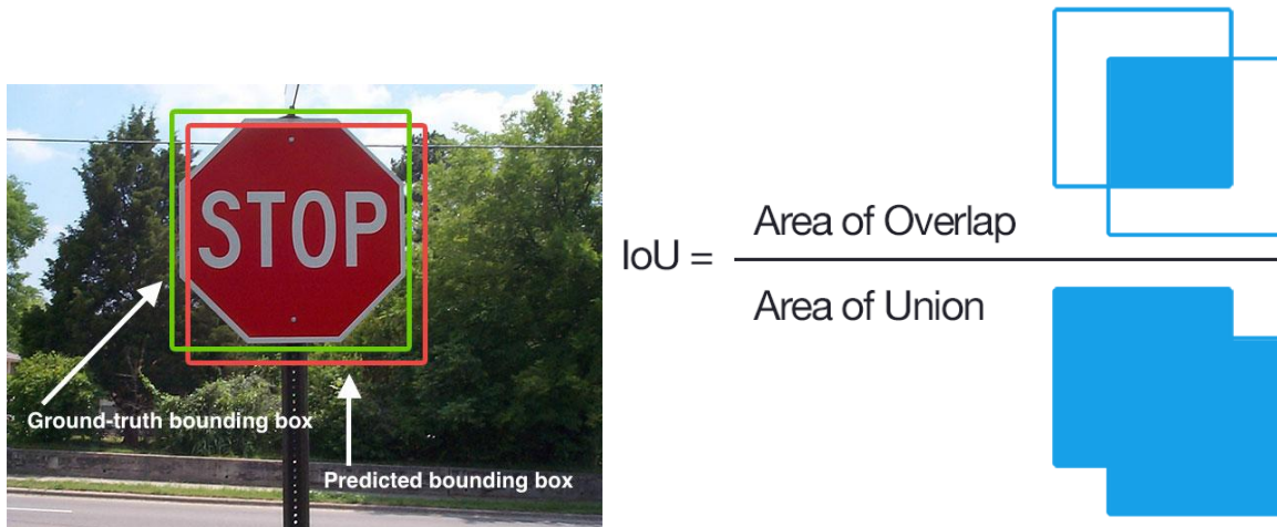
Fig 2.3.5: Intersection over Union (IoU) example. In this case, the ground truth bounding box (green square) is compared to a predicted bounding box (red square), and IoU is the ratio of the area of overlap over the area of union. Photo credit: Adrian Rosebrock, Wikipedia Commons (Rosebrock 2016a, Rosebrock 2016b)
