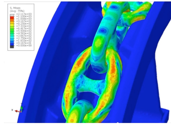
Figure 18. Out-of-Plane Bending
