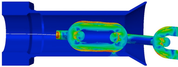
Figure 17. In-Plane Bending
