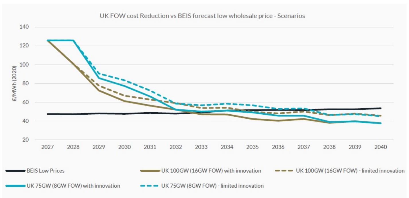
Figure 8. UK Floating Offshore Wind Cost Reduction vs BEIS Forecast Wholesale Electricity Price. Source: ORE Catapult, Floating Offshore Wind Centre of Excellence 10
