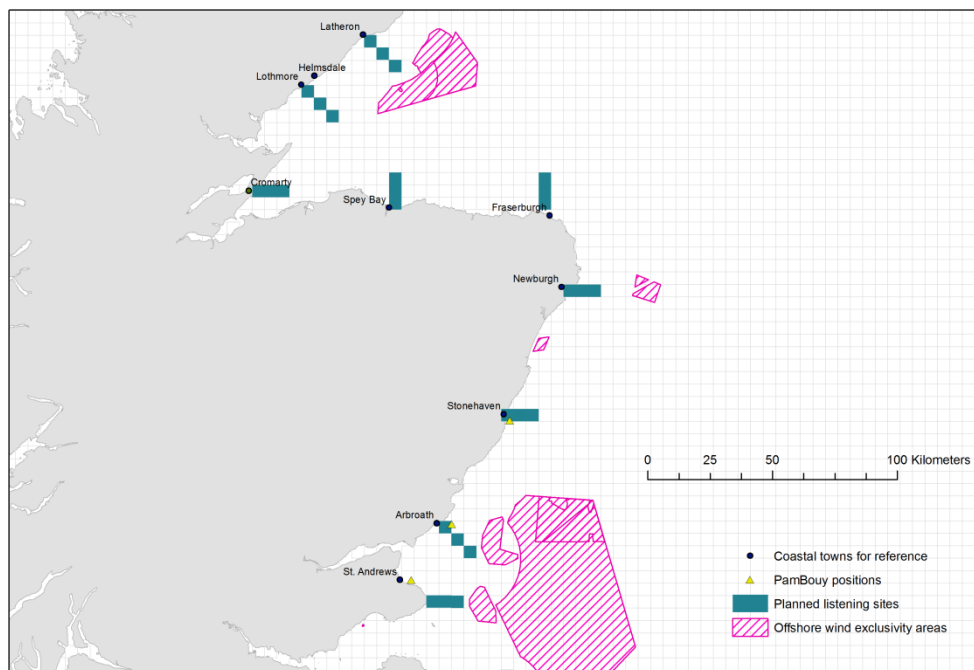
Figure 2. Draft locations for the different passive acoustic devices forming the proposed East Coast PAM network (courtesy of Marine Scotland)
