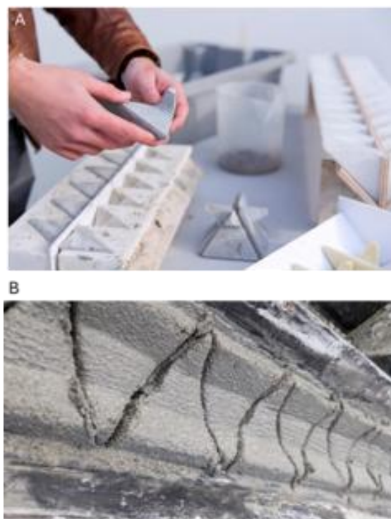
FIGURE 18. PICTURES OF THE PRODUCTION PROCESS OF THE DIFFERENT REEFBOOSTER DESIGNS. A SHOWS DESIGN A, AND B SHOWS DESIGN B.
