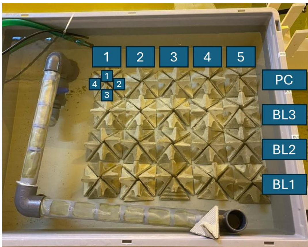
FIGURE 6. SETUP OF EXPERIMENT S1 AND S2 WITH THE REEFBOOSTERS OF DIFFERENT MATERIAL COMPOSITIONS IN THE CRATES ON TOP OF A TO CULTIVATION SYSTEM.
