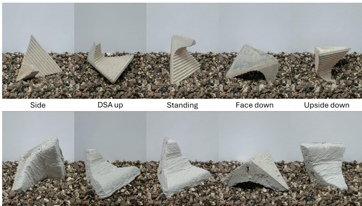
FIGURE 35. LANDING POSITIONS OF REEFBOOSTER DESIGN A (UPPER ROW PICTURES) AND REEFBOOSTER DESIGN B (LOWER ROW PICTURES) ON A COARSE SEDIMENT SURFACE WITH THE DEFINITIONS (SIDE, DSA UP, STANDING, FACE DOWN, UPSIDE DOWN).
