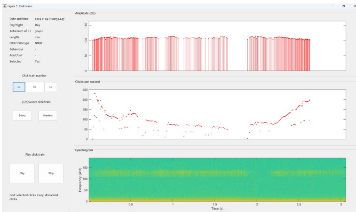
Figure 3-3-8: A screenshot from DPorCCA showing a high quality classified click train from hydrophone 8731.
