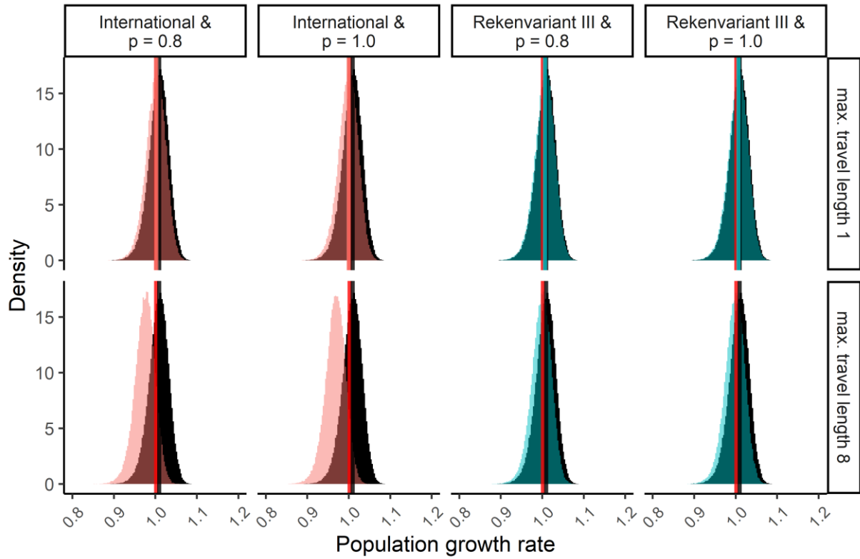
Figure 5. Distribution of population growth rates of the northern gannet for the different scenarios. Vertical lines indicate the median population growth rates of the ALI threshold (red), the null scenario (black) and each OWF-scenario (colours). Estimates of mortality rates are derived from IBM simulations.
