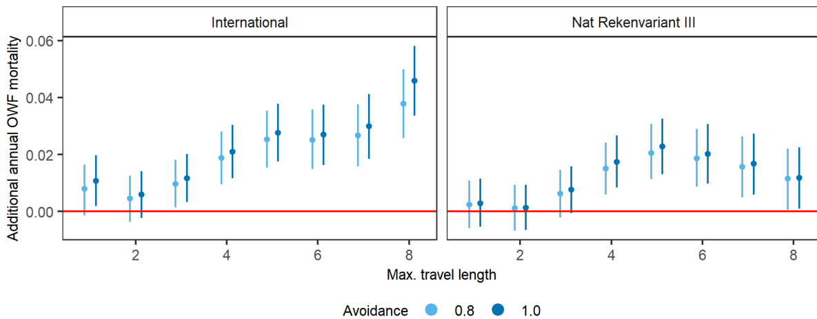
Figure 4. Annual mortality values from OWF-induced habitat loss as estimated by the northern gannet (IBM). Blue points show median mortality values and line ranges extend towards the 5 th and 95 th percentiles. The same data are shown in Table 34.
