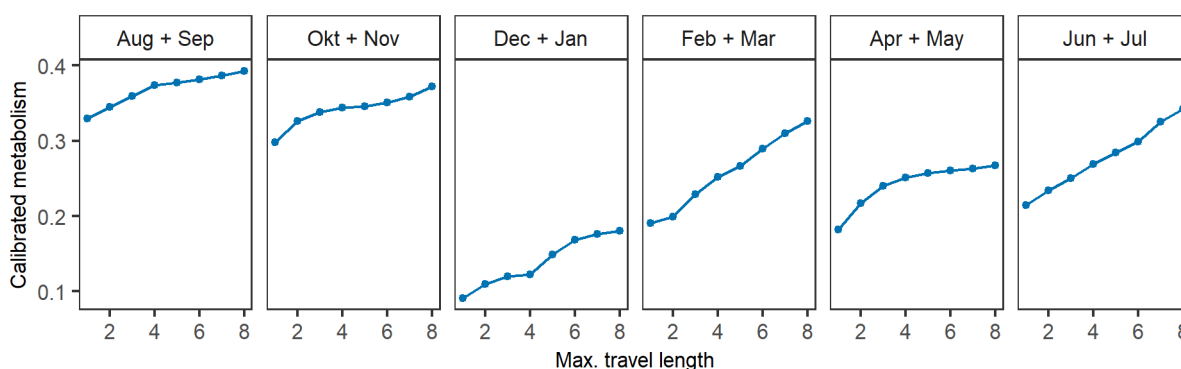
Figure 1. Calibrated metabolism per maximum travel length and bimonthly period.
