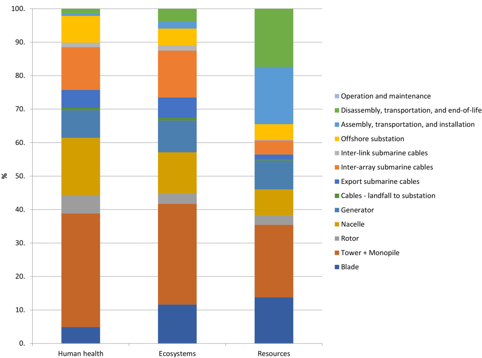
Figure 5. Life cycle impact assessment – endpoint results.
