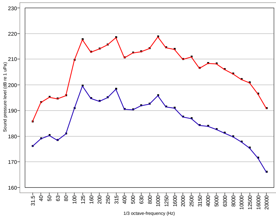
Figure 3.15. Frequency spectrum (Third octave band sound pressure level) of ramming pulses (FINO 1-platform) back-calculated to 1 m (red = \text{dB}_{0-p} re 1 \mu\text{Pa} , blue = \text{dB}_E re 1 \mu\text{Pa} from ITAP, 2005).
