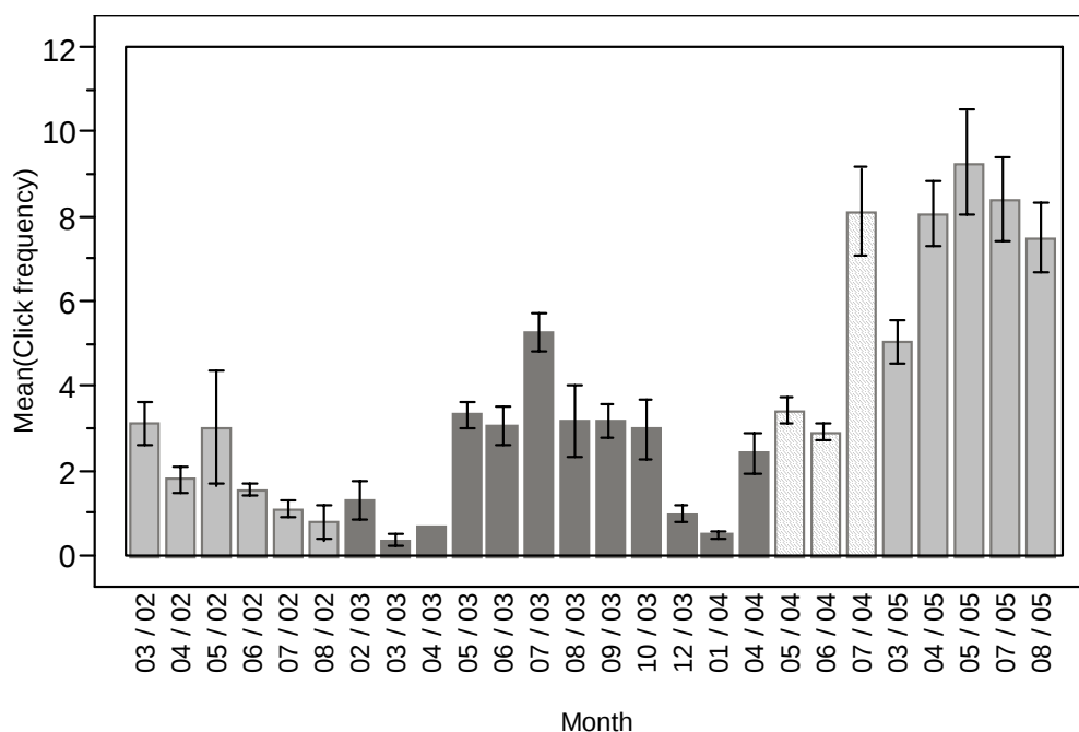
Figure 4.11. Mean click frequency per month in station 7 (+/-SE; light grey = V1, medium grey = V3, dark grey = V4, patterned = V1/V3).
