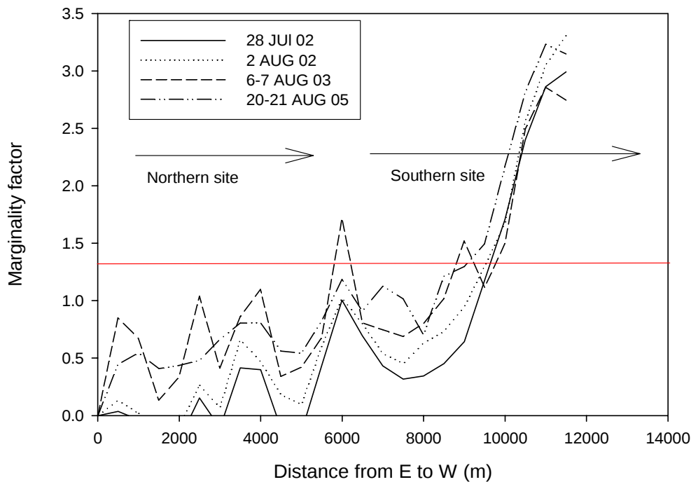
Figure 4.21. Variation in ecological marginality factor for harbour porpoise during north-flowing tidal currents on the four selected surveys along an east-west profile passing through the centre of both the northern and the southern wind farm sites. The red line marks the threshold for significance (mean value plus one standard deviation).
