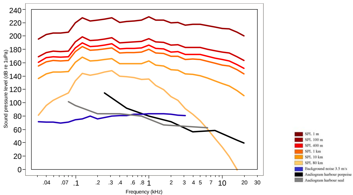
Figure 6.2. Pile-driving noise and background noise (see Figure. 6) compared to the audiogram of harbour porpoises and harbour seals (audiogram values as dB_{rms} re 1 \mu Pa ; after Kastelein et al., 2002 and Kastak & Schusterman, 1998).
