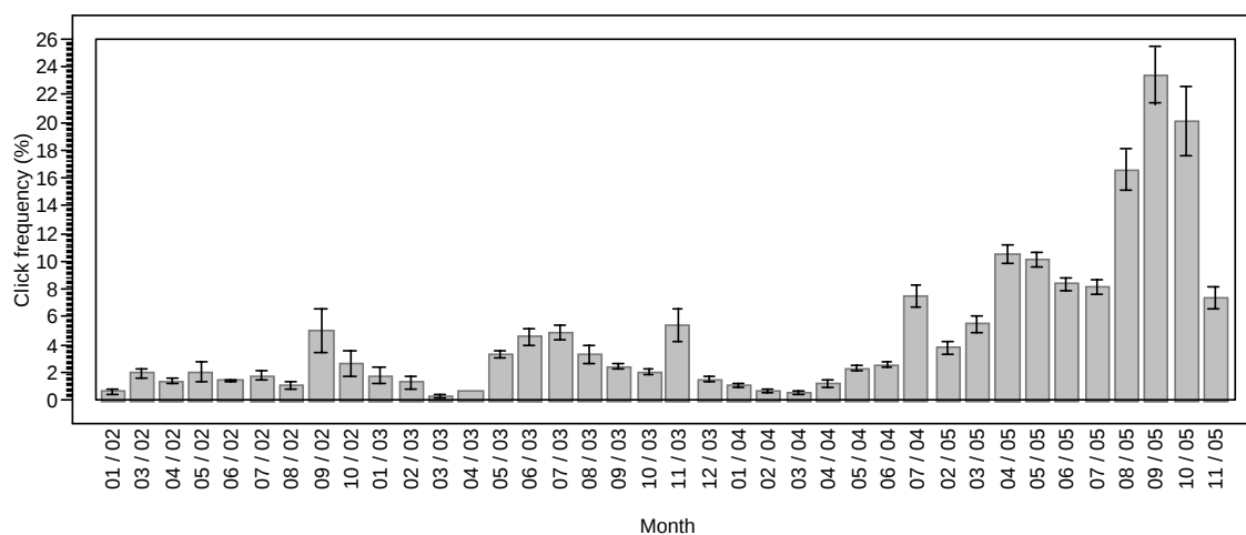
Figure 4.4. Mean click frequency by month (all data; error bars = SE).
