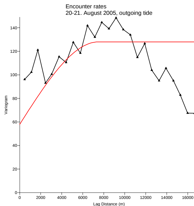
Figure 4.24. Empirical and experimental variograms of encounter rates of harbour porpoises during August 20-21, 2005.
