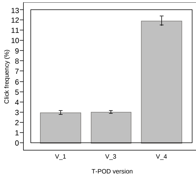
Figure 4.5. Mean click frequency by T-POD version (all data; error bars = SE).
