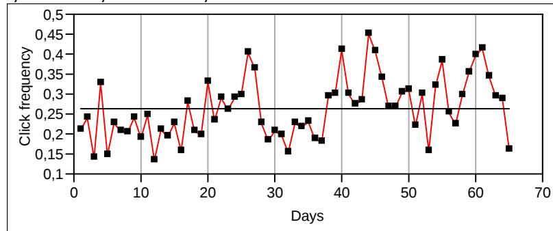
Time Series B Station 7, T-POD 282, 10.03 – 13.05.05 - residuals
