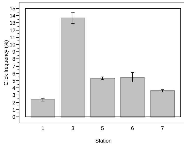
Figure 4.1. Mean click frequency by station (all data; error bars = SE).
