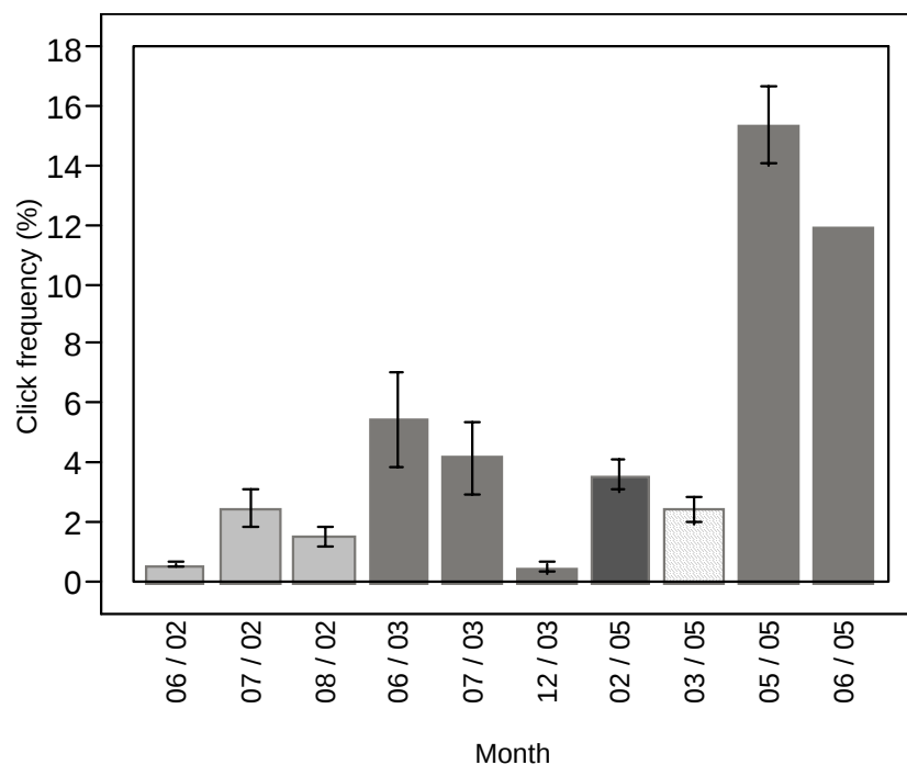
Figure 4.10. Mean click frequency per month in station 6 (+/-SE; light grey = V1, medium grey = V3, dark grey = V4, patterned = V3/V4).
