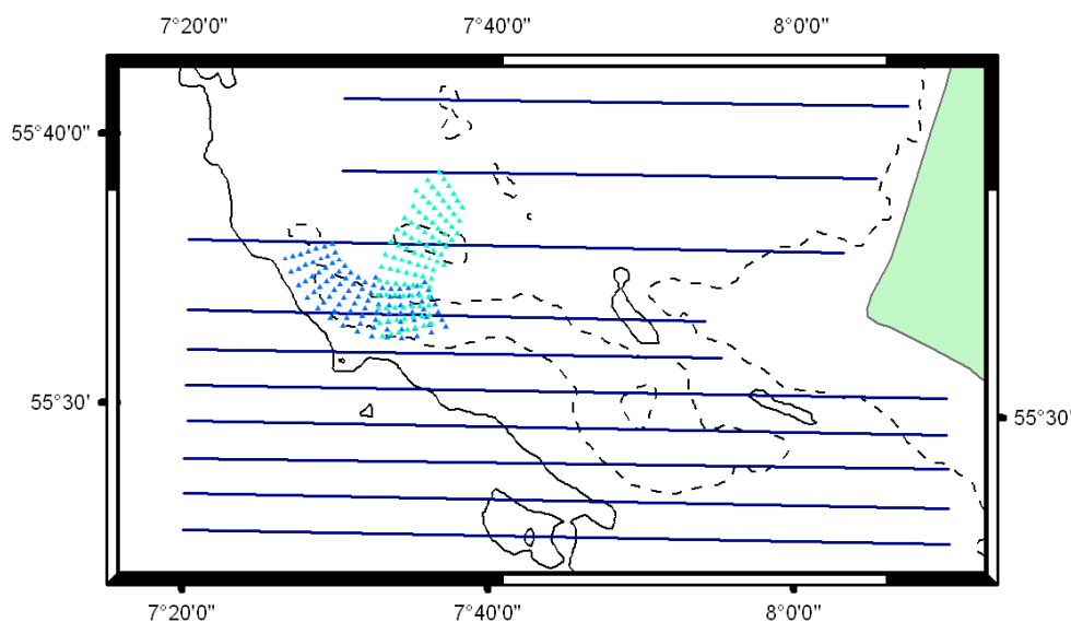
Figure 3.4. Survey design for the dedicated ship-based surveys of harbour porpoises associated with the Horns Rev 1 Offshore Windfarm (minimum number of lines covered).
