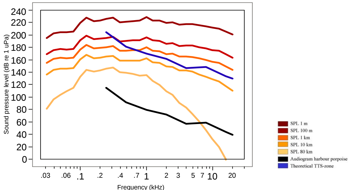
Figure 6.4. Attenuation of impact pile-driving noise at different distances from the source compared with the audiogram and a theoretical threshold shift zone of 90 dB above audiogram.
