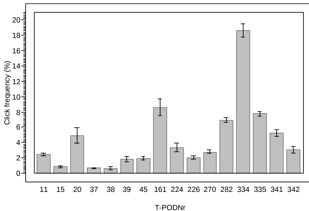
Figure 4.6. Mean click frequency by T-POD number (all data; error bars = SE).
