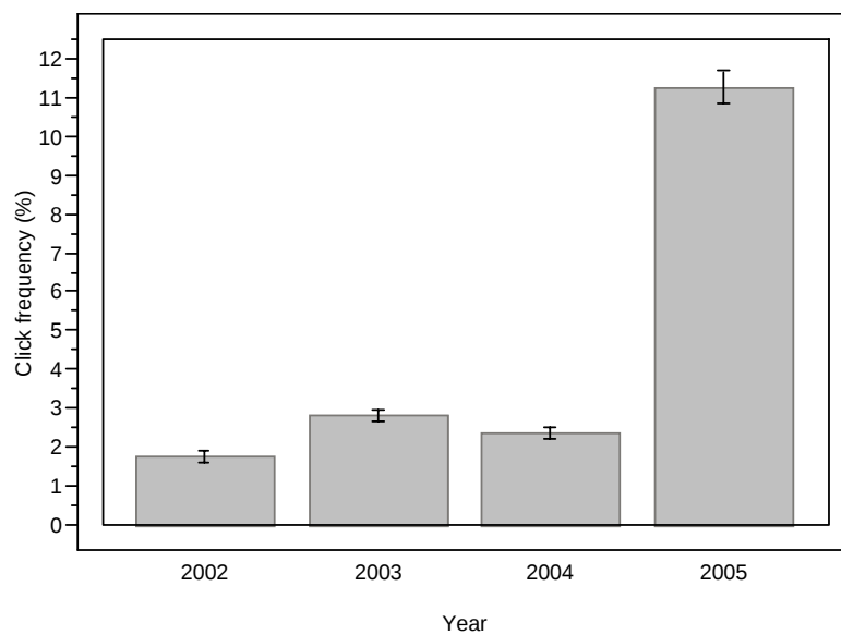
Figure 4.2. Mean click frequency by year (all data; error bars = SE).
