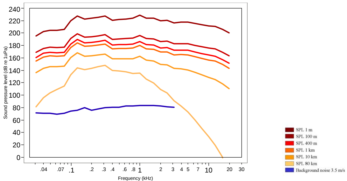
Figure 6.1. Attenuation of pile-driving noise at different distances from the source and background noise levels at moderate wind-speeds (Pile-driving noise after ITAP (2005) and Betke, pers. Comm; values as dB_{0-p} re 1 \mu Pa in 1/3 octave-bands; TL-calculations after Thiele (2002); background noise levels as 1/3 octave-bands in dB_{Leq} re 1 \mu Pa after Betke et al., 2004).
