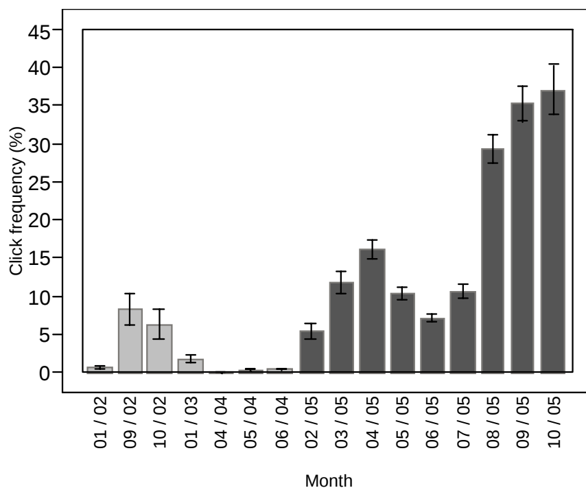
Figure 4.8. Mean click frequency per month in station 3 (+/-SE; light grey = V1, medium grey = V3, dark grey = V4).
