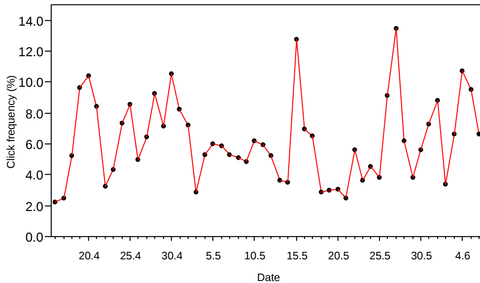
Figure 4.12. Daily click frequency from 16.04.05 – 06.06.05 recorded at station 1.
