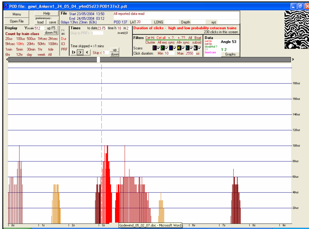
Figure 3.2. Example diagram from the T-POD software showing clicks and trains of different probability (x-axis = time (s); y-axis = duration ( \mu s); red = CET-HI clicks, brown / yellow = CET-LO clicks).
