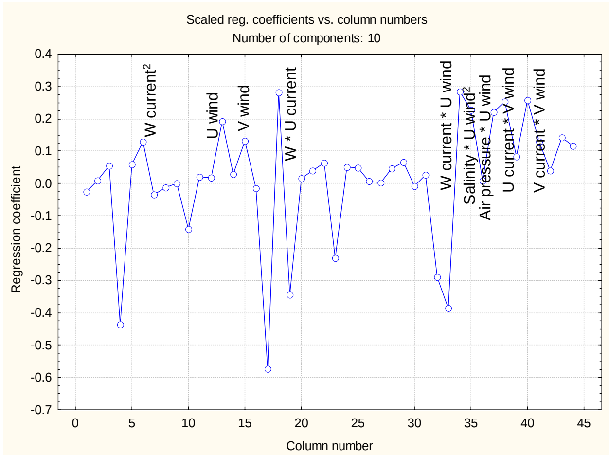
Figure 4.15. Results of the PLS regression showing regression coefficients vs environmental variables for daily click frequency at station HR 1.
