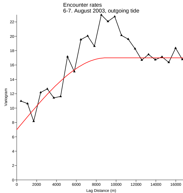
Figure 4.23. Empirical and experimental variograms of encounter rates of harbour porpoises during August 6-7, 2003.
