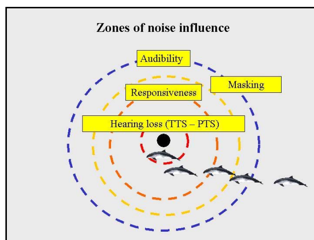
Figure 3.13. Zones of noise influence (after Richardson et al., 1995).
