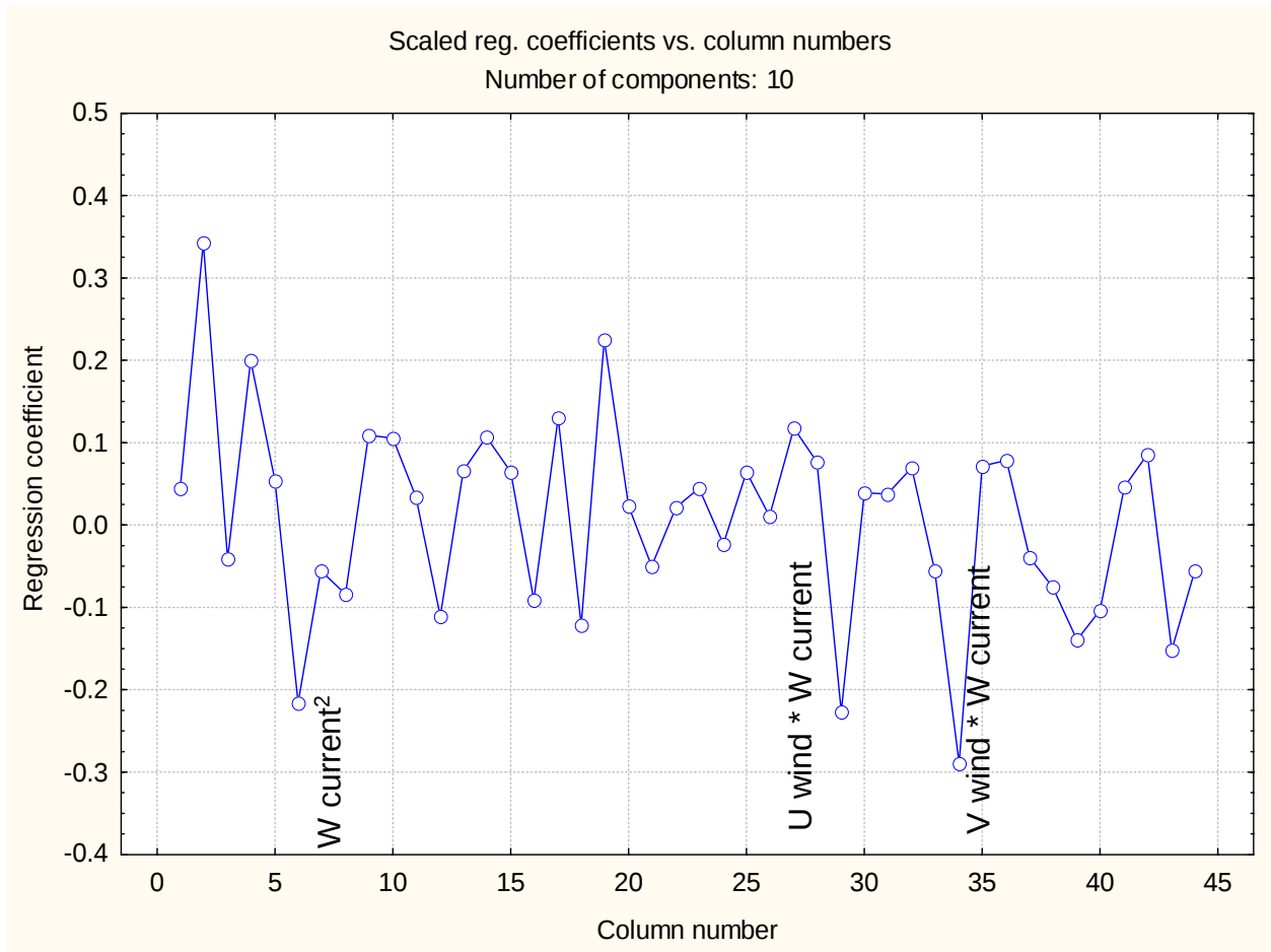
Figure 4.13. Results of the PLS regression showing regression coefficients vs environmental variables for waiting times at station HR 1.
