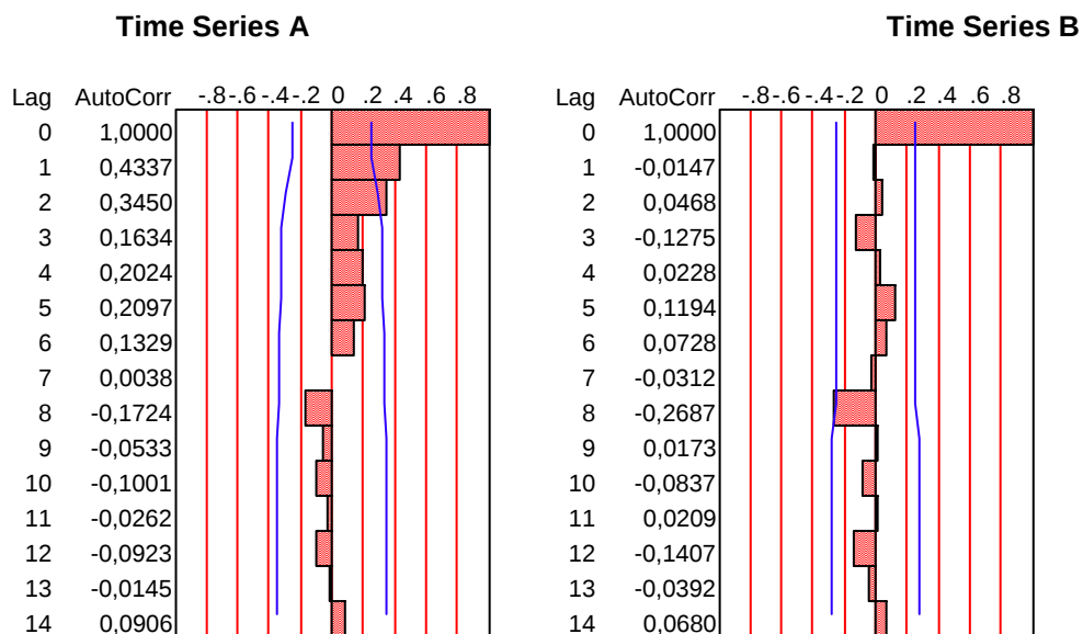
Figure 3.9. Time series of daily click frequencies and the residual series from a station 7 deployment in 2005. The autocorrelation graph is shown below, indicating lag 1 and lag 2 autocorrelation (left graph) for the transformed frequencies and no autocorrelation in the residuals (right graph).
