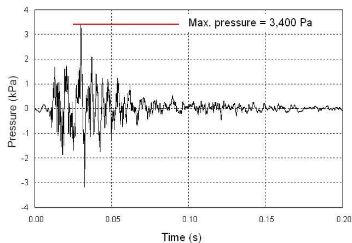
Figure 3.14. Waveform of a impact-pile pulse (after ITAP, 2005).
