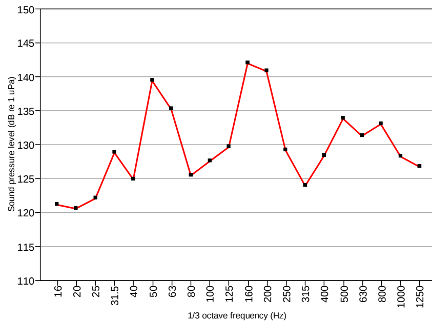
Figure 3.16. Operational source level noise in dB_{Leq} of an offshore wind turbine measured at a 110 m distance and back-calculated to 1 m (from ITAP, 2005).
