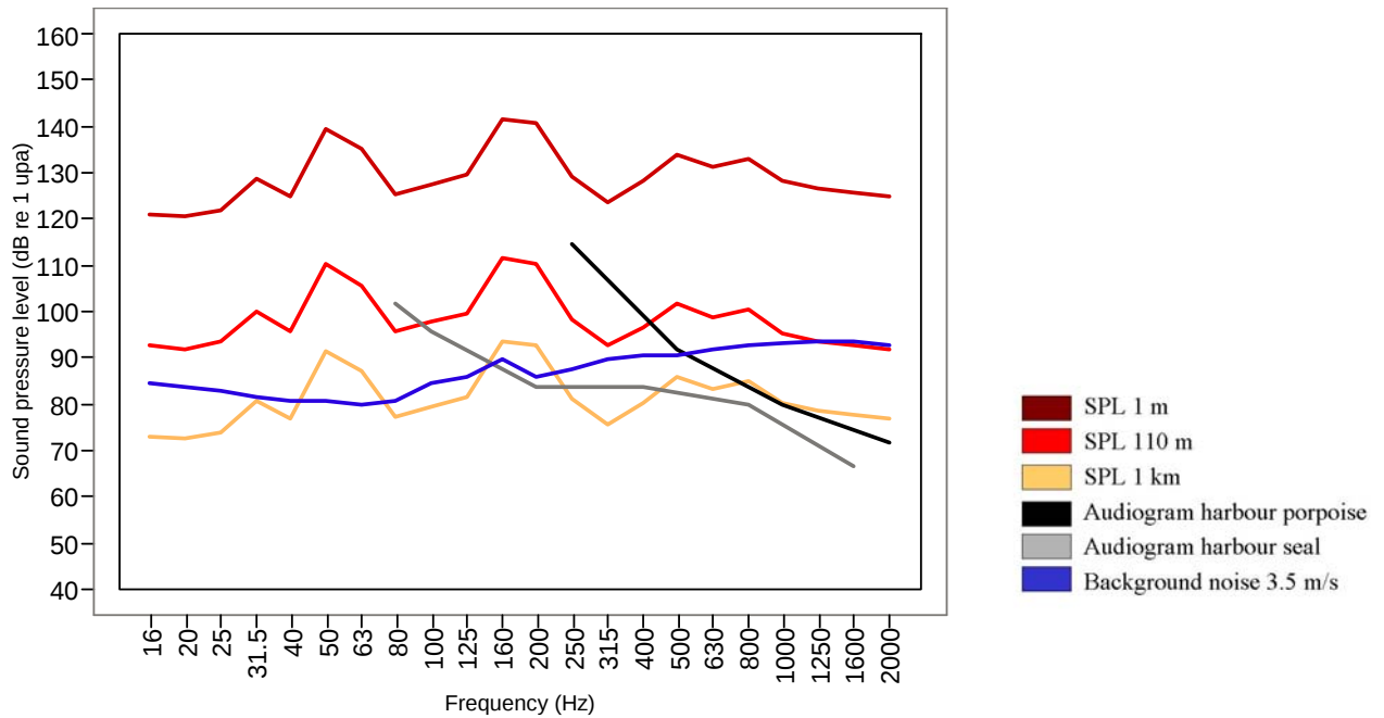
Figure 6.5. Sound pressure levels at an offshore wind farm in operation in at different distances from the source compared to the audiogram of harbour porpoises and harbour seals and background noise (SPL = L_{eq} in 1/3 octave sound pressure levels; 110 m = measurement; 1 m = back-calculated after Thiele, 2002; 1,000 m calculated with 16 \log(r) ; background noise after Betke et al., 2004 and Madsen et al., 2006; audiogram harbour porpoise by Kastelein et al., 2002; harbour seal by Kastak & Schusterman, 1998).
