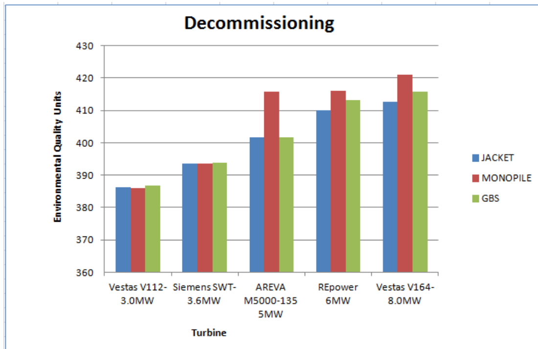
Figure 11: Decommissioning of different turbines with corresponding base structures
