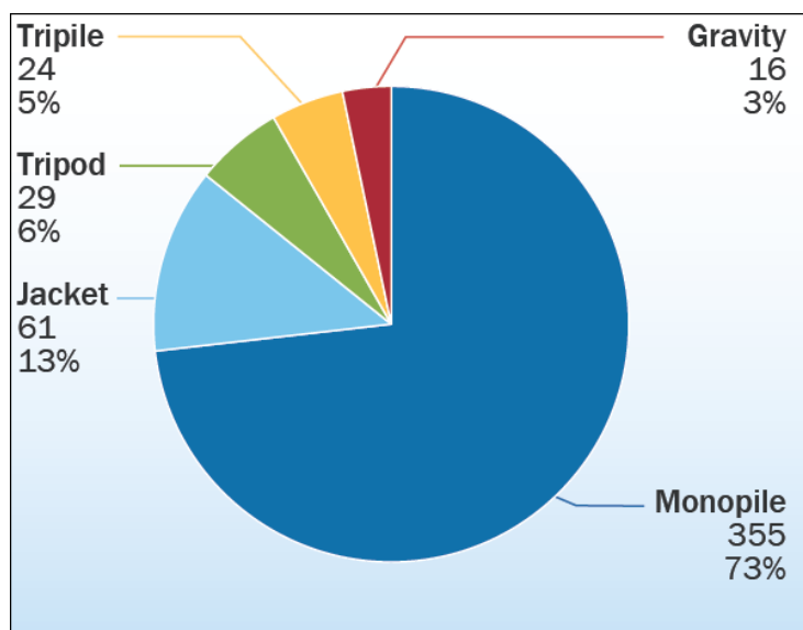
Figure 8: Distribution of foundation types (EWEA 2013)
