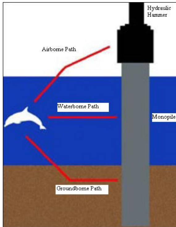
Figure 15: Three different paths for noise travelling away from pile driving (Van den Akker et al., 2012)
