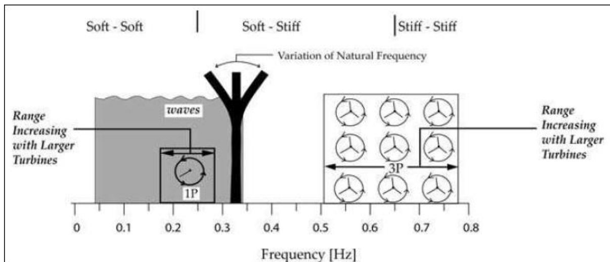
Figure 6: Typical ranges for frequencies of waves, rotors, blade passing and structure (Malhotra, 2011)
