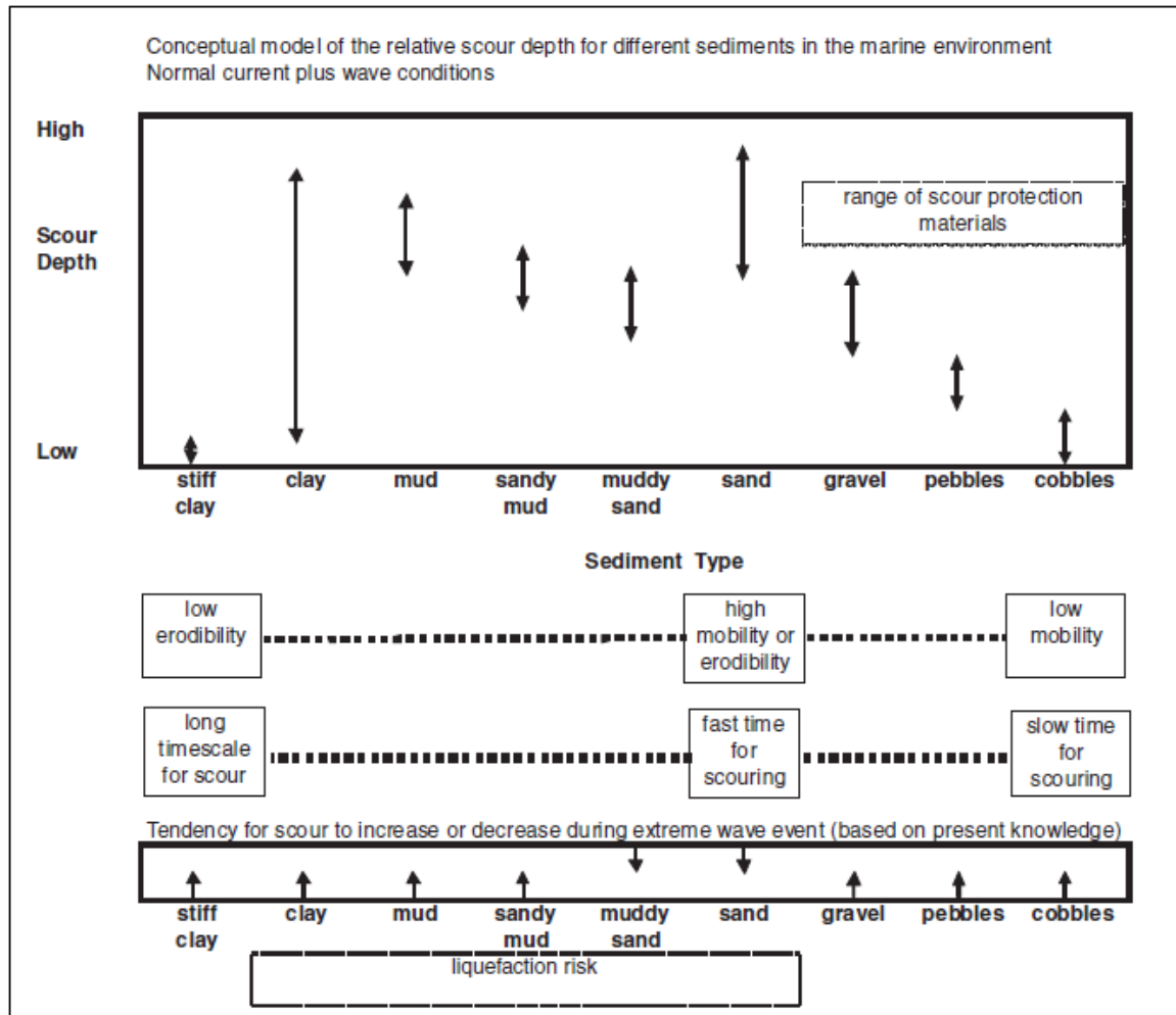
Figure 18: Conceptual model for scour development around marine foundations (Whitehouse et al., 2010)
