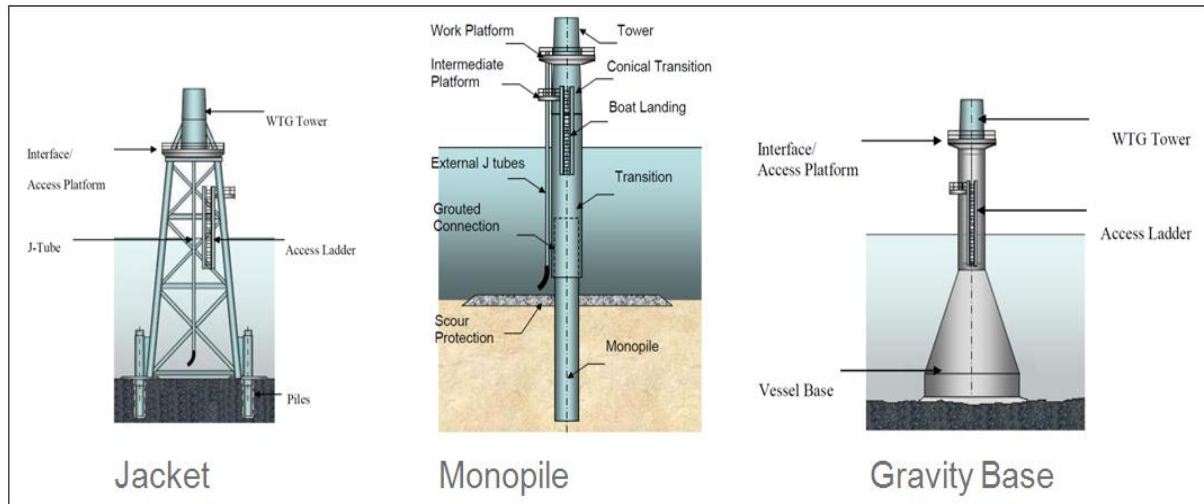
Figure 7: Base foundations used in this investigation (adapted from IMECHE, 2010)
