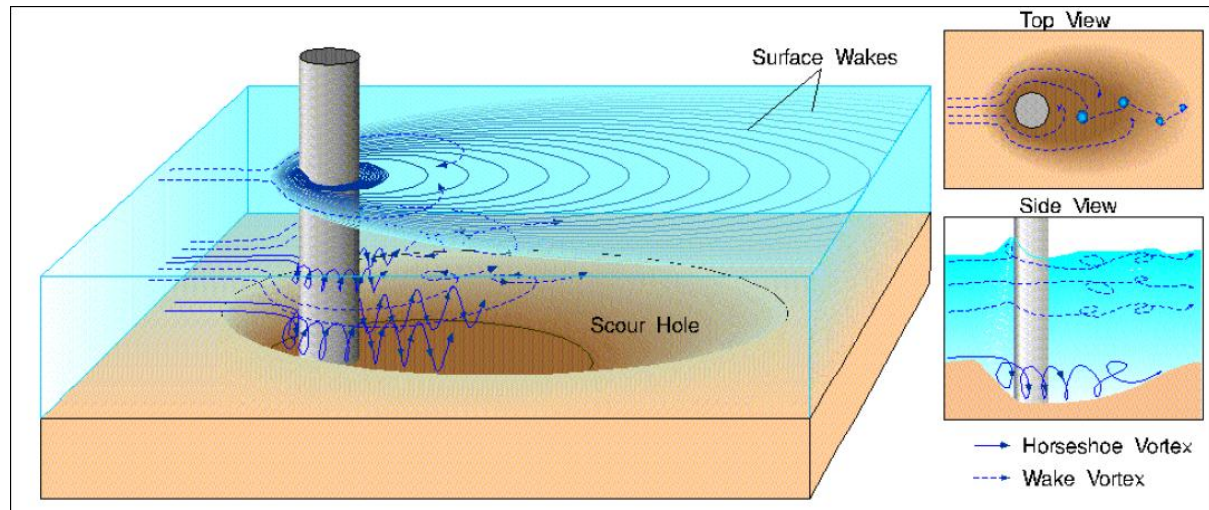
Figure 20: Horseshoe vortex and lee wake (Huizinga et al., 2009)
