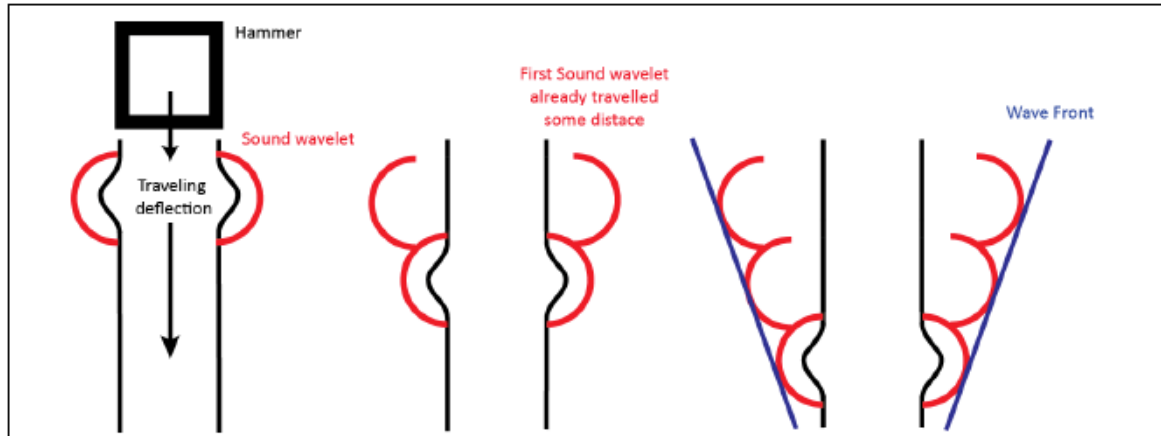
Figure 16: Sound generation during pile driving impact hammer (Saleem, 2011)
