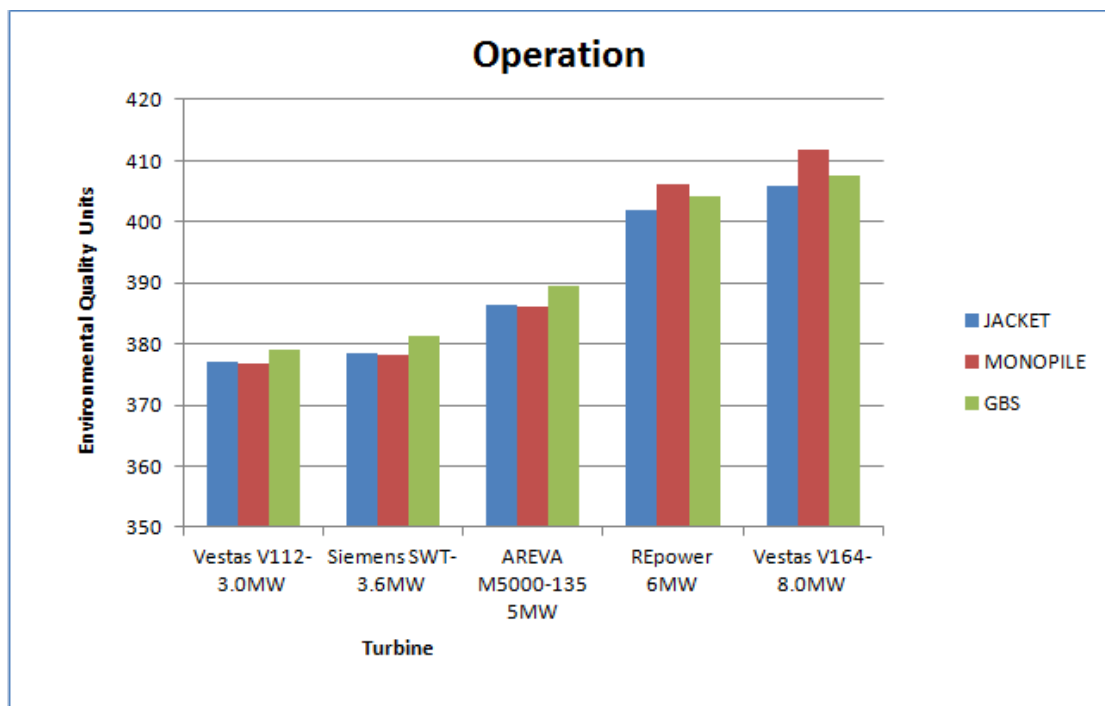
Figure 10: Operation of different turbines with corresponding base structures
