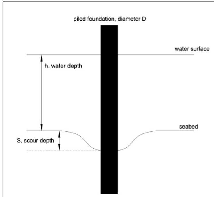
Figure 17: Scour cross section (Whitehouse et al., 2007)
