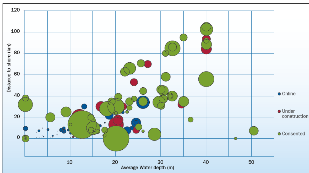
Figure 5: Water depths and distance to shore (EWEA 2013)
