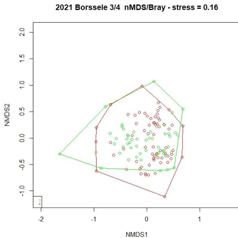
Figure 18. NMDS displaying the differences in species-composition between samples of Borsssele III (green, with oyster tables) and Borsssele IV (red, without oyster tables).
