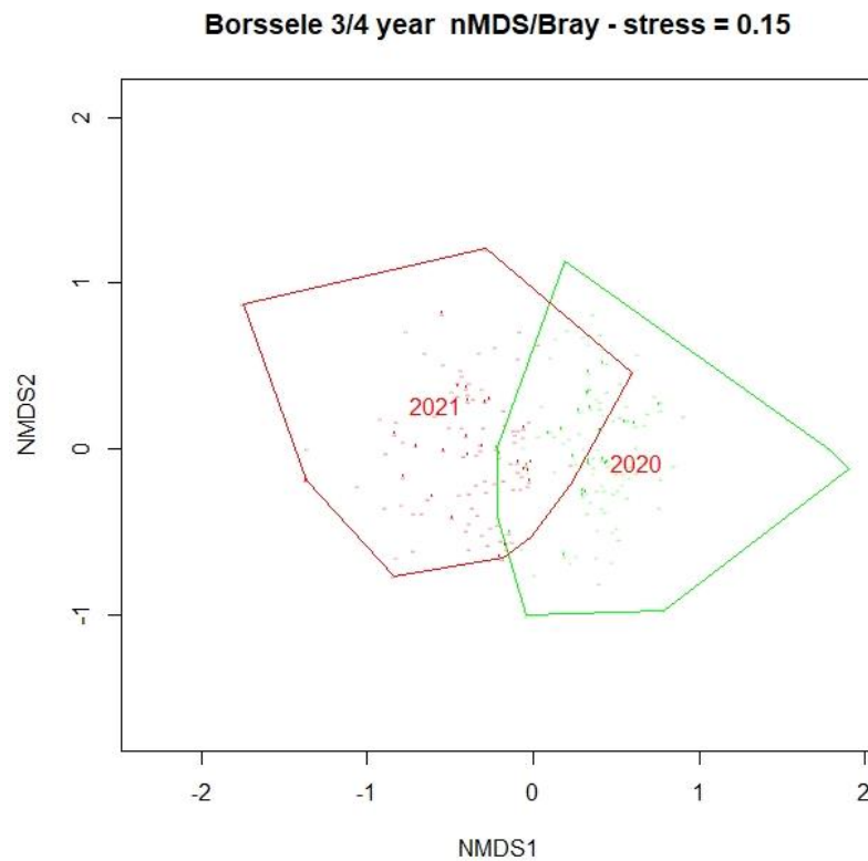
Figure 15. NMDS displaying the differences in species-composition between samples of 2020 and 2021 (all samples except H3 in 2020).
