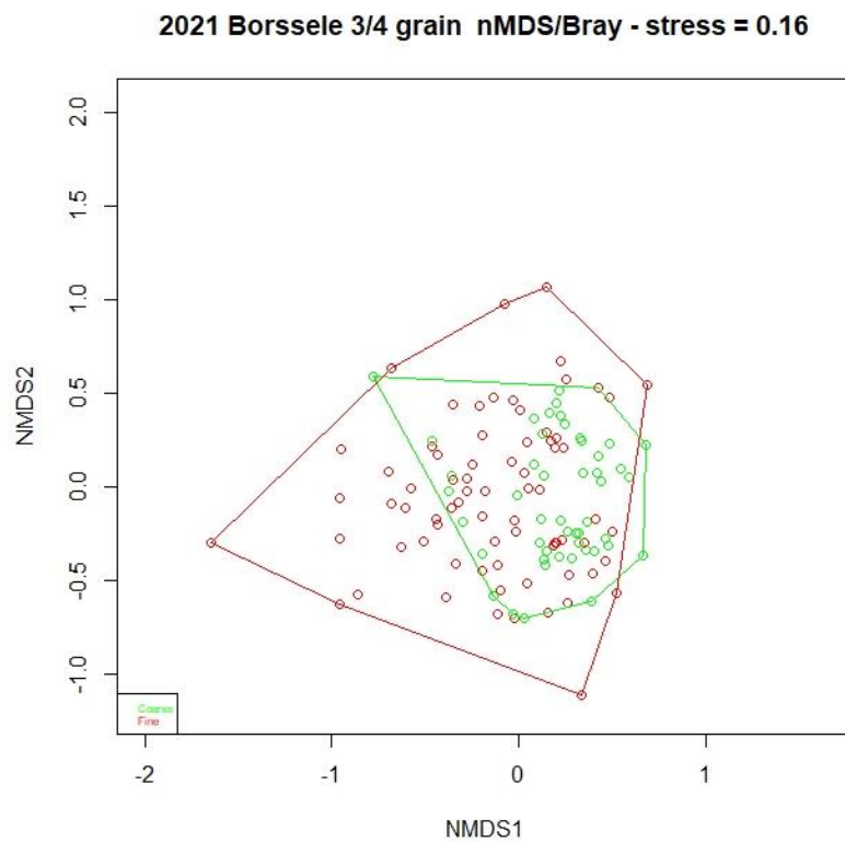
Figure 17. NMDS displaying the differences in species-composition between samples on coarse-grain (green) and fine-grain scour-protection (red).
