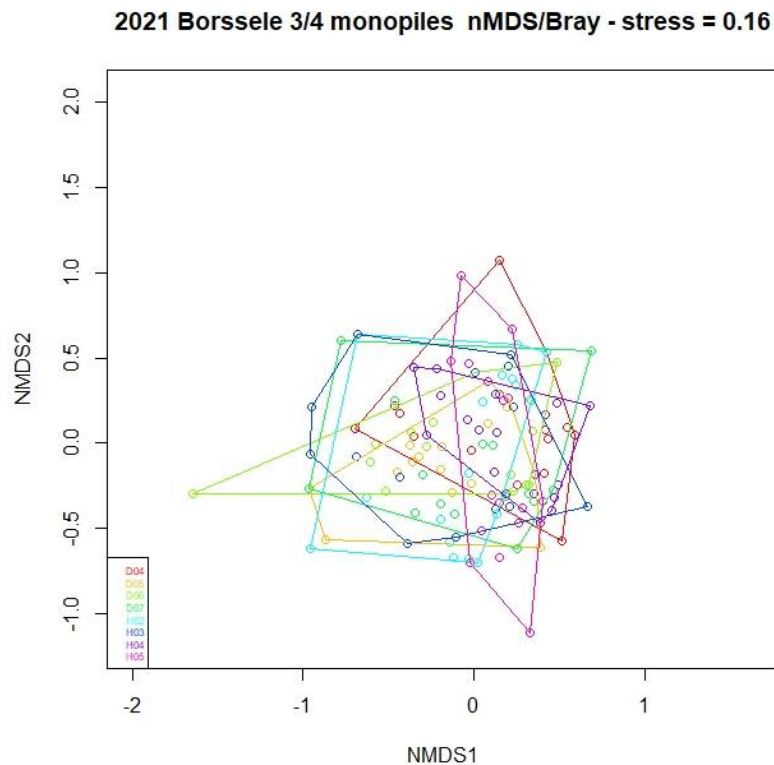
Figure 19. nMDS displaying the differences in species-composition between samples of different monopiles (D04=red, D05=yellow, D06=light green, D07=dark green, H02=light blue, H03=dark blue, H04=purple, H05=pink).
