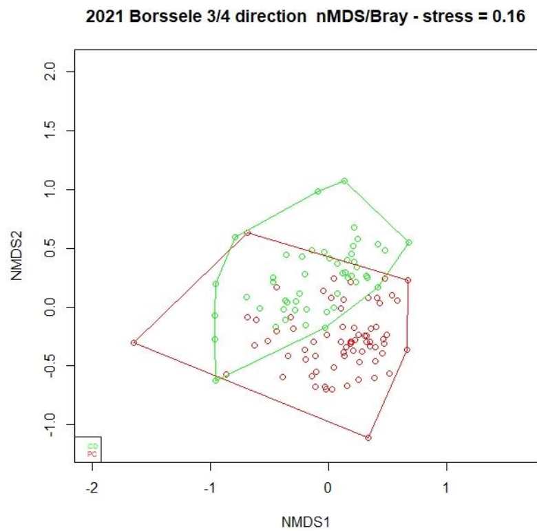
Figure 16. NMDS displaying the differences in species-composition between samples of current-direction (green) and perpendicular-current direction samples (red).
