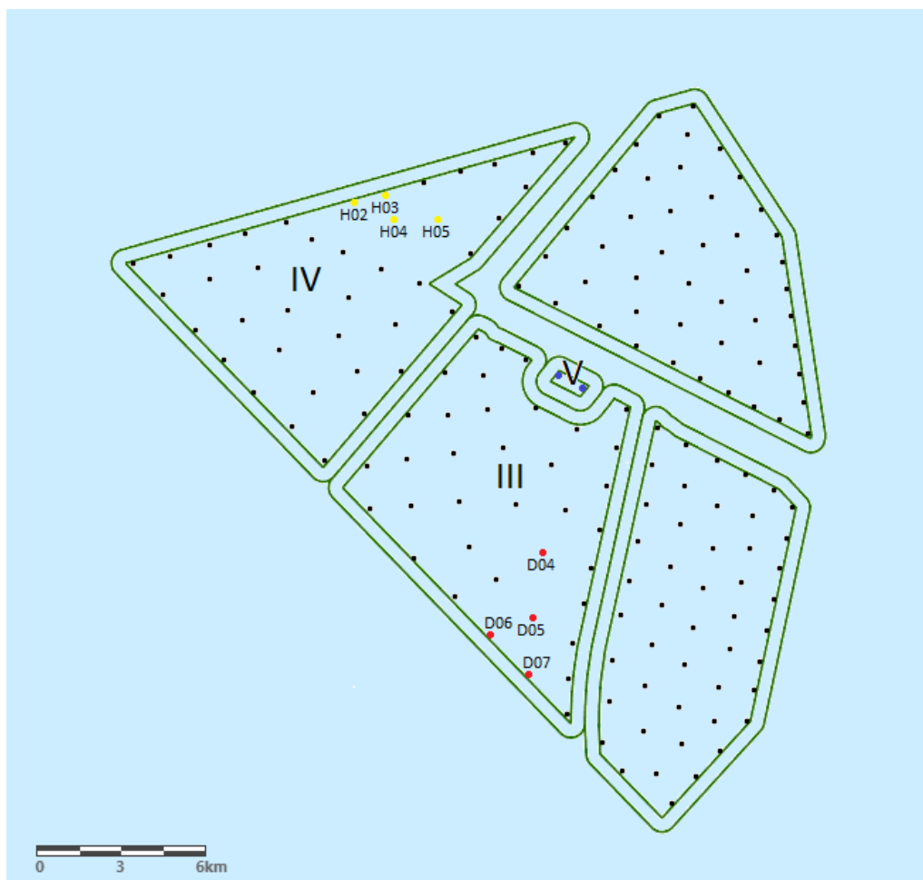
Figure 2-1: Overview of the Borssele offshore wind park. Red dots concern the locations for the oyster installation (from top to bottom B334-D04, B337-D05, B328-D06 and B327-D07), the yellow dots are the reference locations (from left to right: B412-H02, B411-H03, B402-H04 and B401-H05). The blue dots concern locations on Borssele 5.
