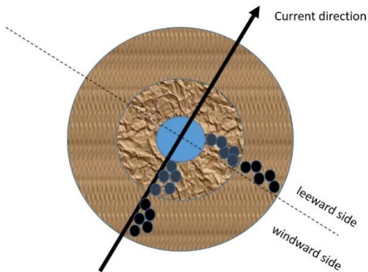
Figure 2-7: the positioning of coarse and filter gradings around the monopiles, and the approximate positioning pictures (black dots in filter grade, gray dots in coarse grade)
