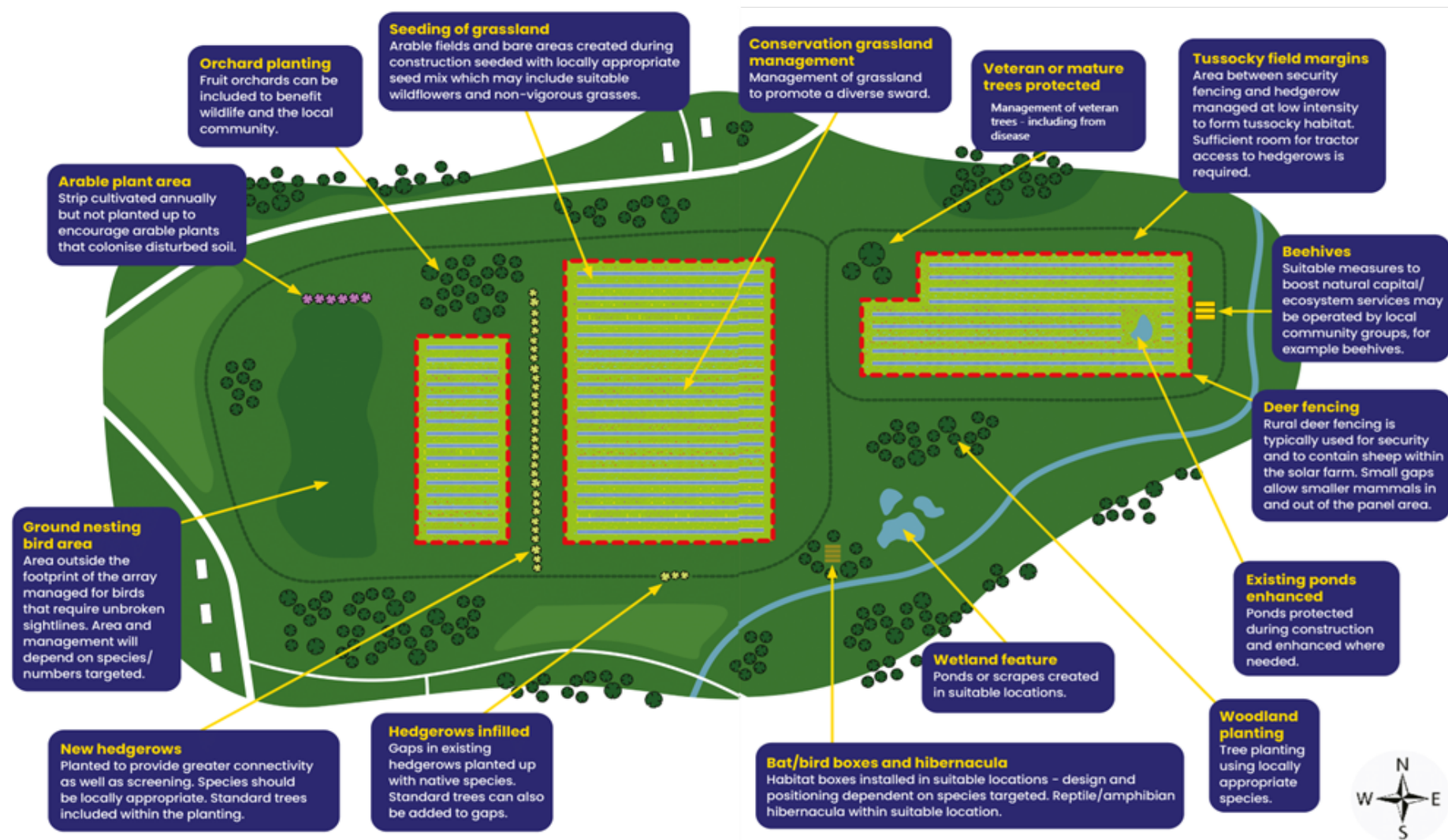
Figure 4 Examples of opportunities for biodiversity enhancement at a hypothetical PV solar farm (Source: Solar Energy UK 2022 pp 24-25).
