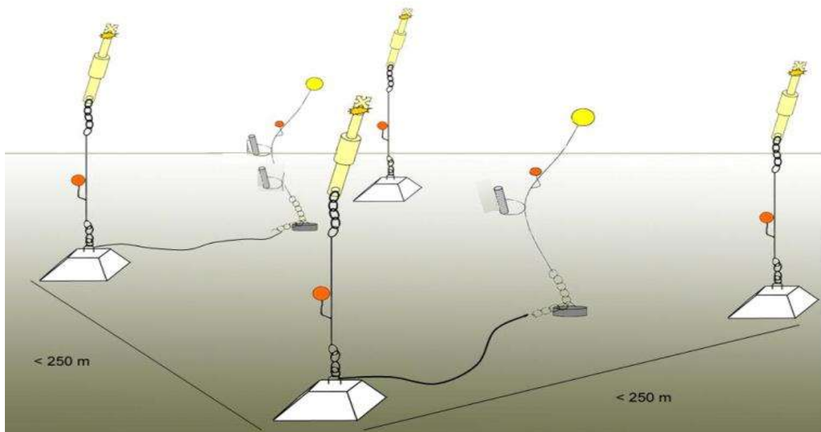
Figure 4.3 CPOD system used by BioConsult SH for CPOD stations with three devices (drawing: Honnef/Gauger).
