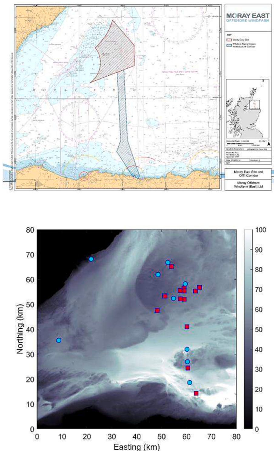
Fig. 1. Map of windfarm location (above) and bathymetric map (below) showing location of the UXO (squares) and recorders (circles) for Moray East (depth scale in metres).
