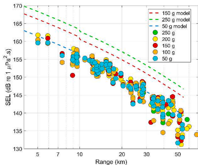
Fig. 10. The broadband SEL values versus range at Moray East for the scare charges, with model predictions.
