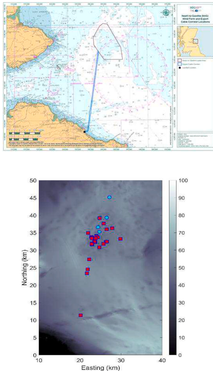
Fig. 2. Map of windfarm location (above) and bathymetric map (below) showing location of the UXO (squares) and recorders (circles) for the NnG site (depth scale in metres).
