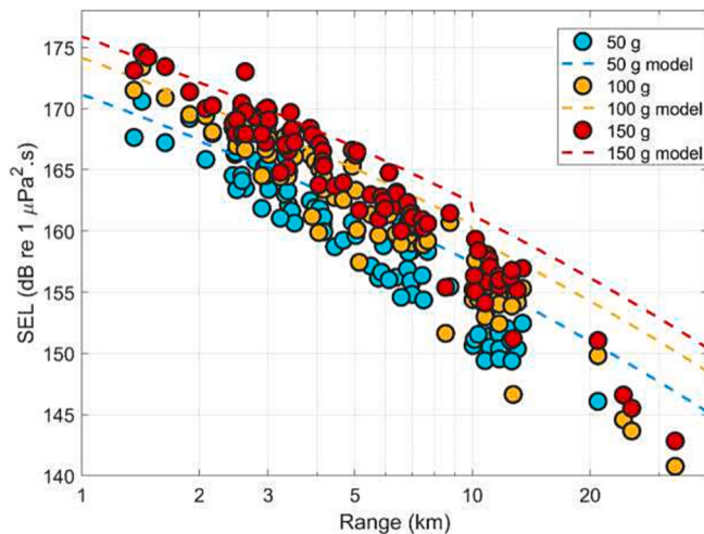
Fig. 8. The broadband SEL values versus range at NnG for the scare charges, with model predictions.
