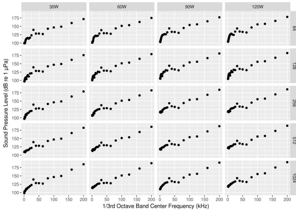
Figure 9: 1/3-octave sound pressure levels (TOLs) of EK60 200 kHz signals by power in Watt (vertical panels) and duration in \mu s (horizontal panels). Integration time: 30 ms; FFT size: 1024 pt.
