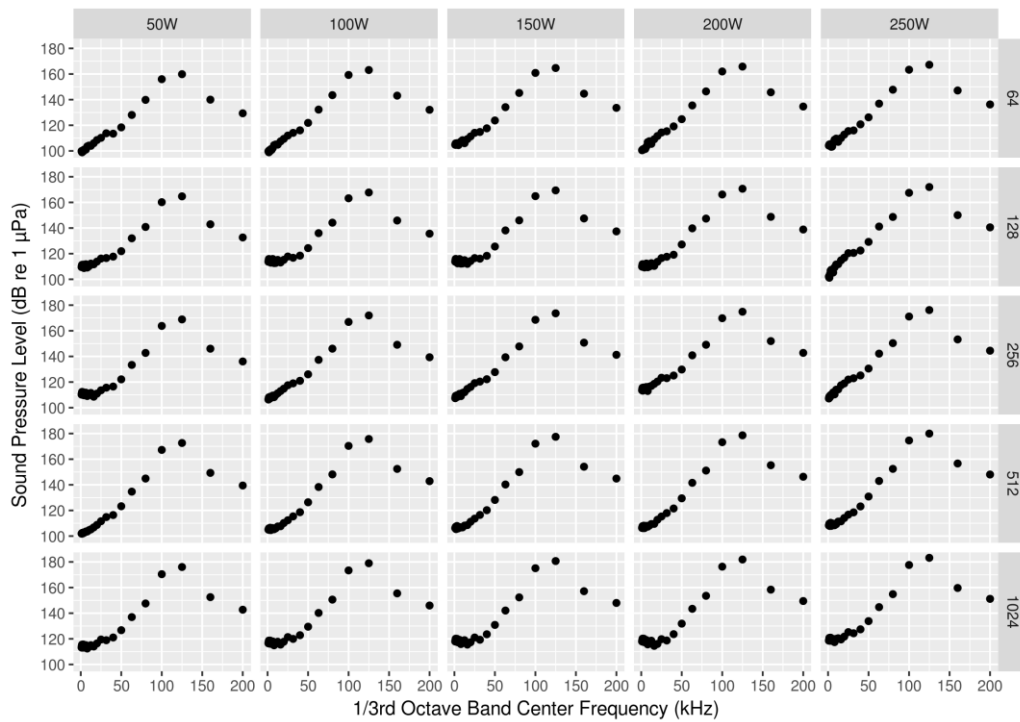
Figure 8: 1/3-octave sound pressure level (TOL) of EK60 120 kHz signals by power in Watt (vertical panels) and duration in \mu s (horizontal panels). Integration time: 30 ms; FFT size: 1024 pt.
