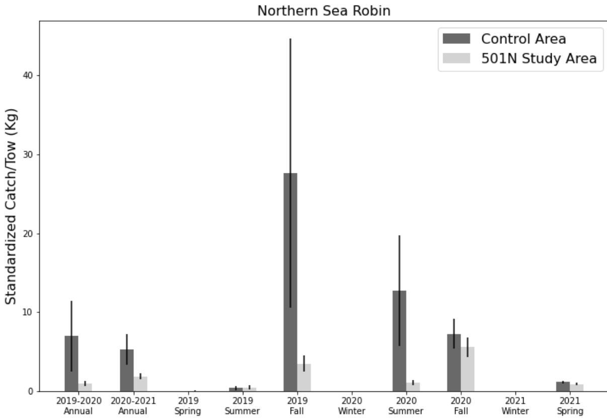
Figure 74: Seasonal catch rates of northern sea robin in the 501N Study Area and Control Area.
