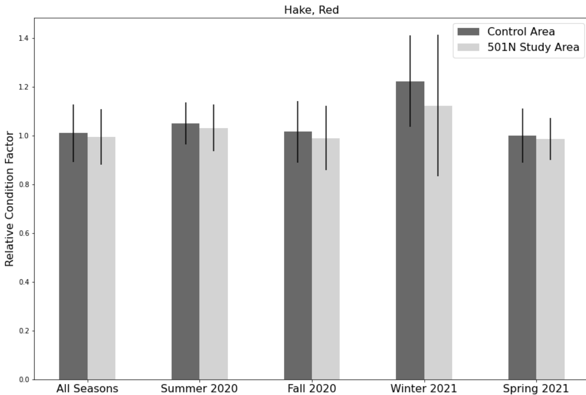
Figure 58: The seasonal condition of red hake (bottom) as derived from the length-weight relationship (top).
