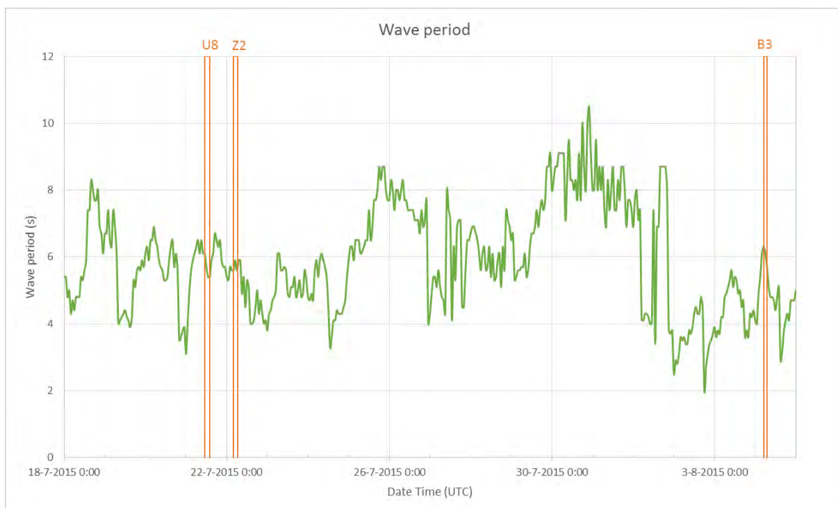
Figure 21: Wave period (measured)
