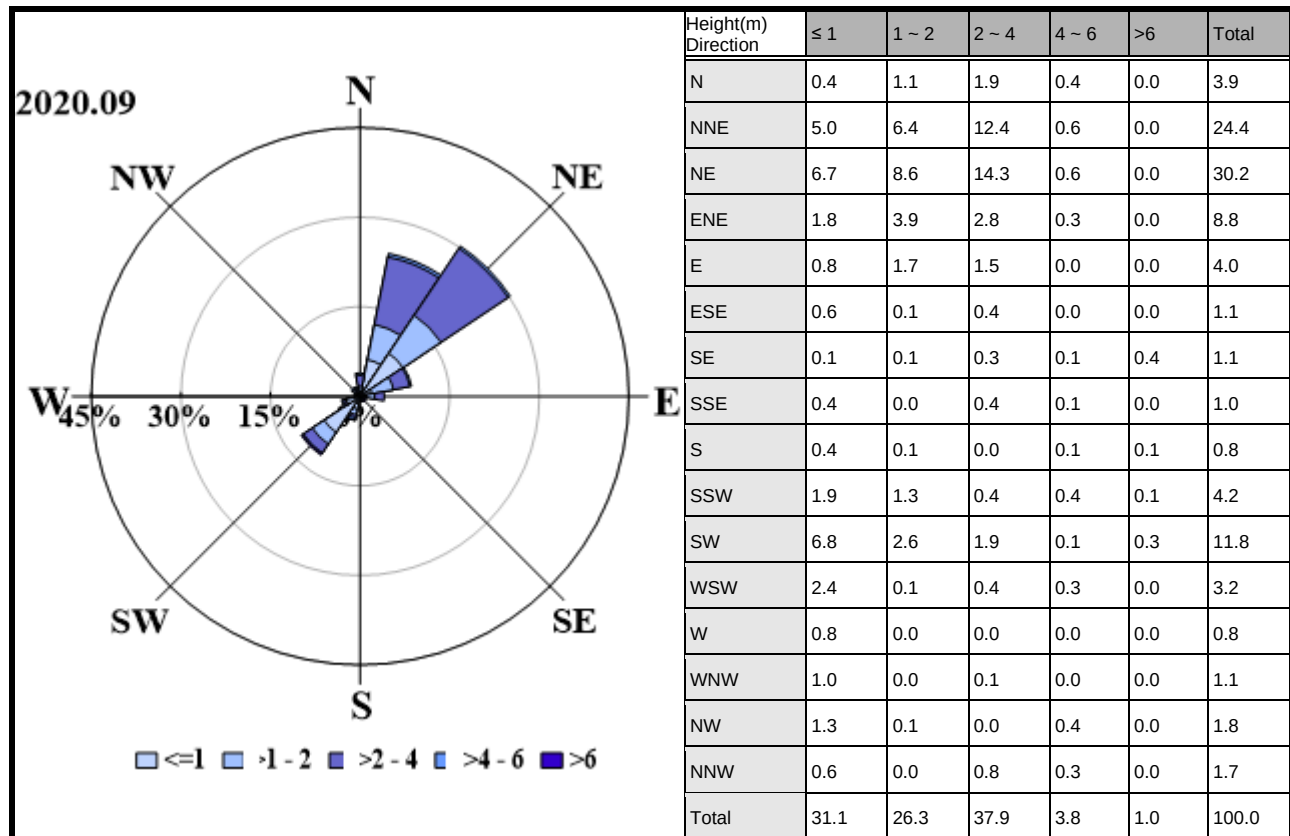
Apx Figure 17: September 2020 significant wave height appearance rate by wave direction (unit: %).
