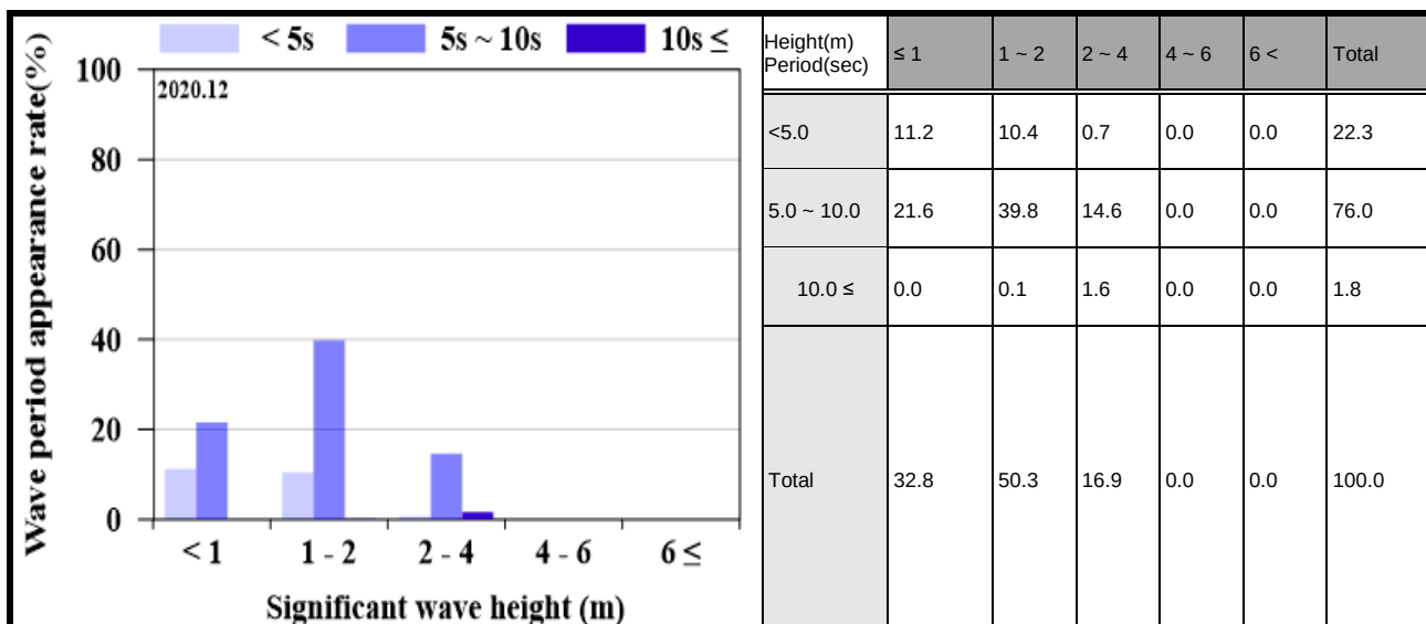
Apx Figure 24: December 2020 significant wave height appearance rate by wave period (unit: %).
