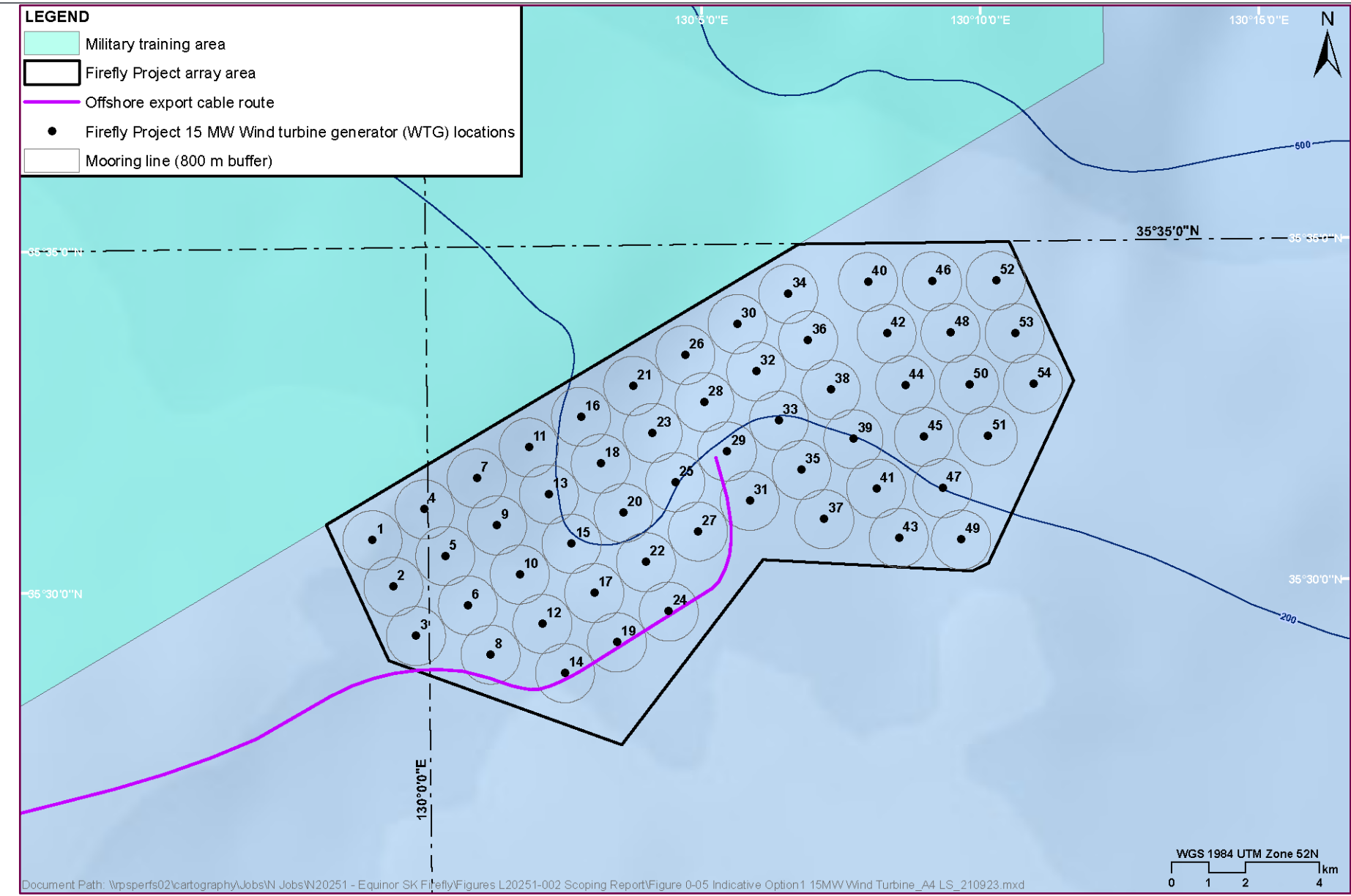
Figure 3-5: Indicative 15 MW Wind Turbine Generator locations.
