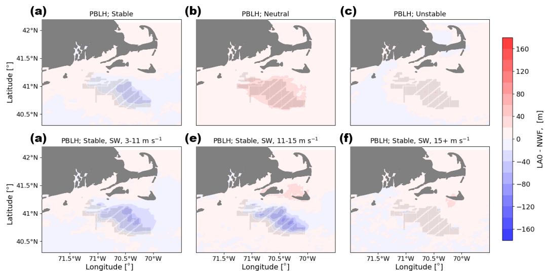
Figure 22. Mean PBLH difference between the LA0 and NWF simulations in (a) stable conditions, (b) neutral conditions, (c) unstable conditions, (d) 3\text{--}11\text{ m s}^{-1} , (e) 11\text{--}15\text{ m s}^{-1} , and (f) 15+\text{ m s}^{-1} . Panels (d), (e), and (f) are only during times with stable conditions and southwest winds. Turbines are marked in gray.
