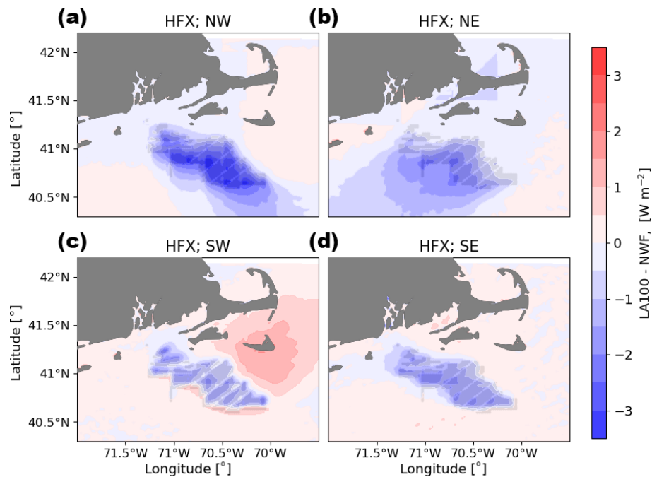
Figure B4. Mean heat flux difference between the LA100 and NWF simulations for (a) NW, (b) NE, (c) SW, and (d) SE wind directions. Turbines are marked in gray.
