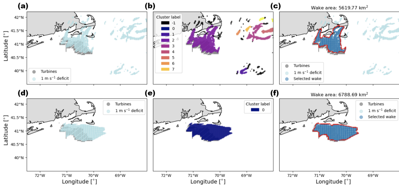
Figure 7. Example of the three steps taken to identify the wind plant wake on 14 December 2019 at 22:00 UTC ( a , b , c ) and on 4 February 2020 at 07:00 UTC ( d , e , f ) in the LA100 simulations. Turbines are marked in gray. ( a , d ) All points identified with a 1 \text{ m s}^{-1} deficit are marked in light blue. ( b , e ) The points with a wind speed deficit are clustered, and a label is assigned to each cluster by the DBSCAN algorithm. The -1 label indicates points classified as noise. ( c , f ) The selected wind plant wake is in darker blue, with its wake boundary in red.
