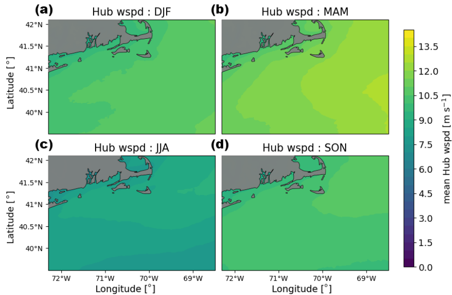
Figure A1. Same as in Fig. 5 but for hub-height wind speed.
