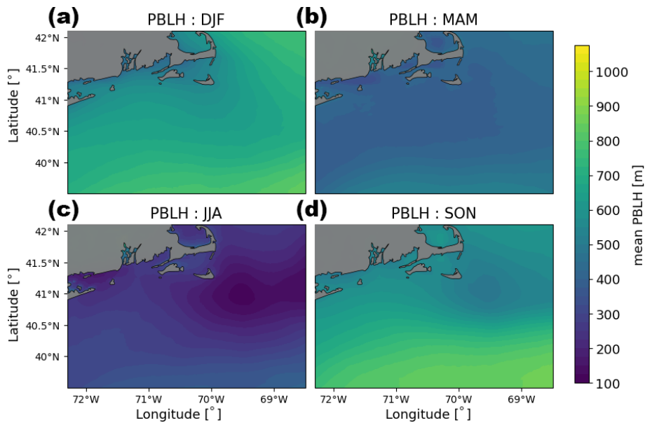
Figure 5. Same as in Fig. 3 but for PBLH.
