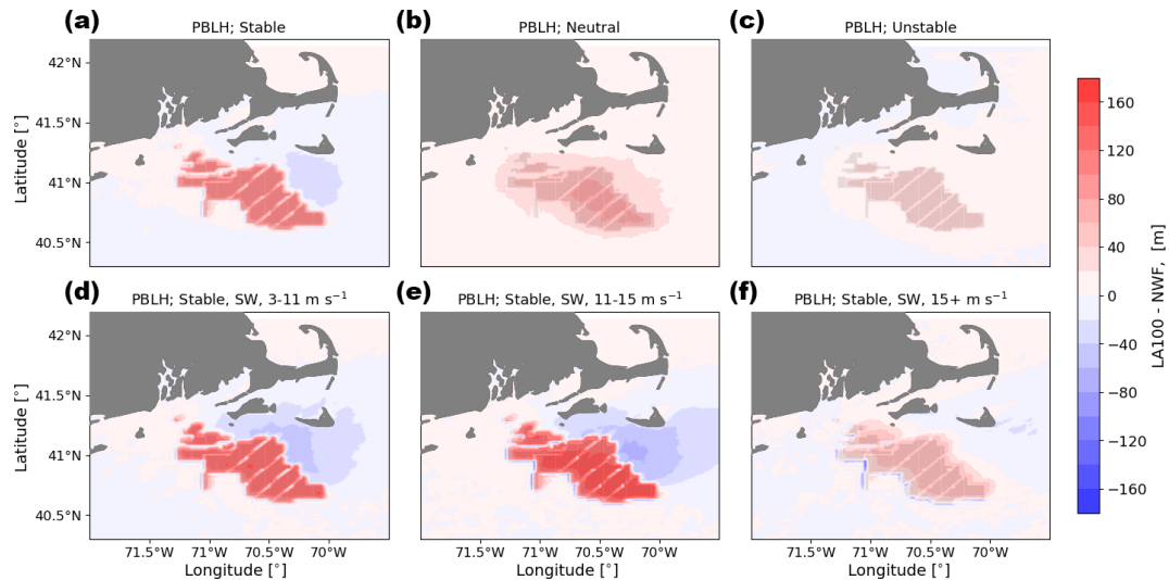
Figure 21. Mean PBLH difference between the LA100 and NWF simulations in (a) stable conditions, (b) neutral conditions, (c) unstable conditions, (d) 3\text{--}11\text{ m s}^{-1} , (e) 11\text{--}15\text{ m s}^{-1} , and (f) 15+\text{ m s}^{-1} . Panels (d), (e), and (f) are only during times with stable conditions and southwest winds. Turbines are marked in gray.
