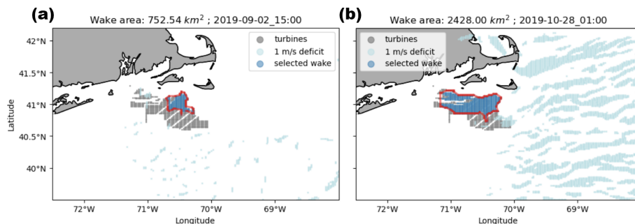
Figure 8. Example of two cases that are flagged by the wake detection algorithm and therefore not considered for further analysis. These plots follow the same convention as panels ( c ) and ( f ) of Fig. 7.
