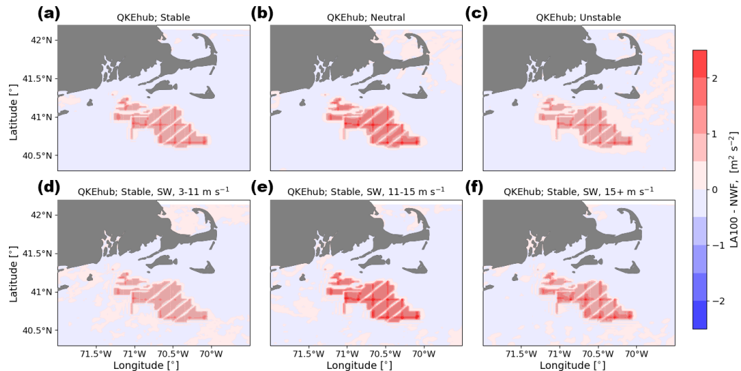
Figure 13. Mean hub-height QKE difference between the LA100 and NWF simulations in (a) stable conditions, (b) neutral conditions, (c) unstable conditions, (d) 3\text{--}11\text{ m s}^{-1} , (e) 11\text{--}15\text{ m s}^{-1} , and (f) 15+\text{ m s}^{-1} . Panels (d), (e), and (f) are only during times with stable conditions and southwest winds. Turbines are marked in gray.
