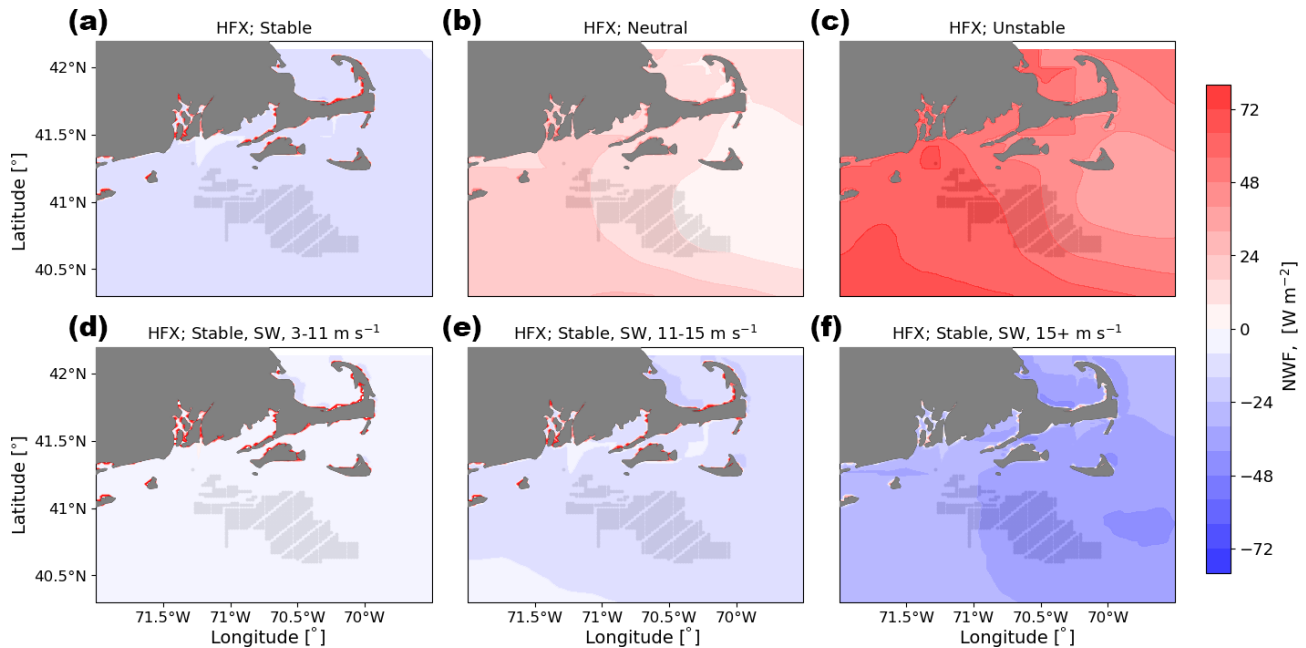
Figure C1. Mean surface heat flux for the NWF simulation in (a) stable conditions, (b) neutral conditions, (c) unstable conditions, (d) 3–11 m s -1 , (e) 11–15 m s -1 , and (f) 15+ m s -1 . Panels (d), (e), and (f) are only during times with stable conditions and southwest winds. Turbines are marked in gray.
