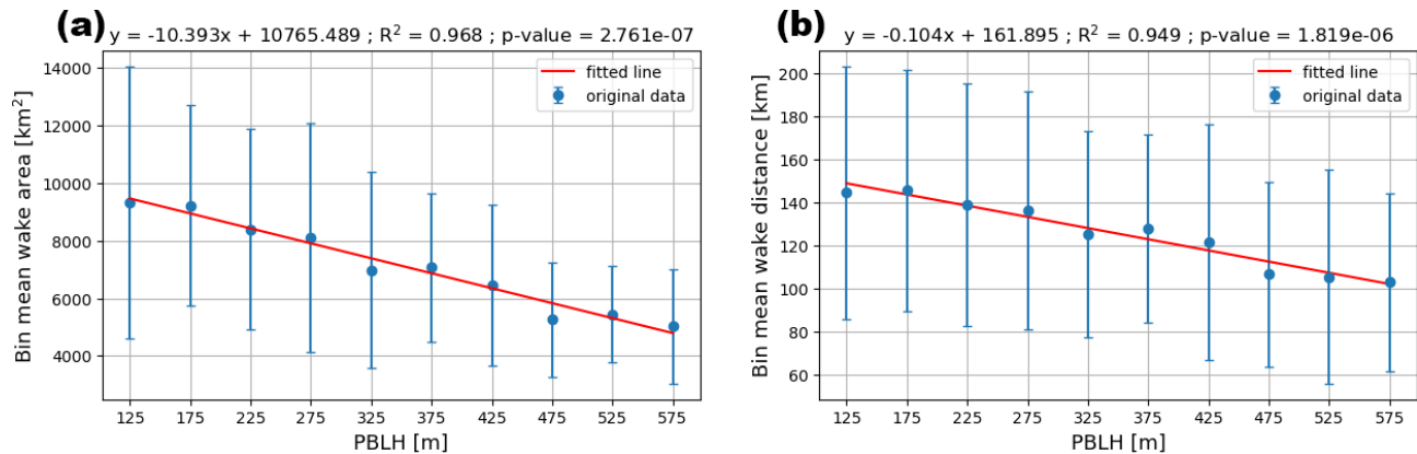
Figure 23. The mean (a) LA100 wake area and (b) LA100 length as a function of the mean lease area PBLH during stable conditions, where the PBLH values are binned every 50 m from 125 to 575 m. The mean PBLH values are calculated as the average PBLH across the wind lease area. For each bin, the blue dots show the mean value, and the blue vertical lines represent the \pm 1 standard deviation error bar. The best-fit line for the bin means is in red. Each panel displays the line of best fit equation, R^2 value, and p value on the top.
