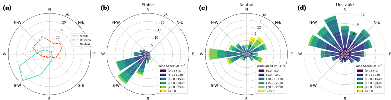
Figure 6. (a) The frequency of each 22.5° wind direction bin for each stability classification. Wind roses for stable, neutral, and unstable conditions are shown in panels (b), (c), and (d), respectively. In all panels, radial distance from the center refers to the percentage of values in each 22.5° bin.
