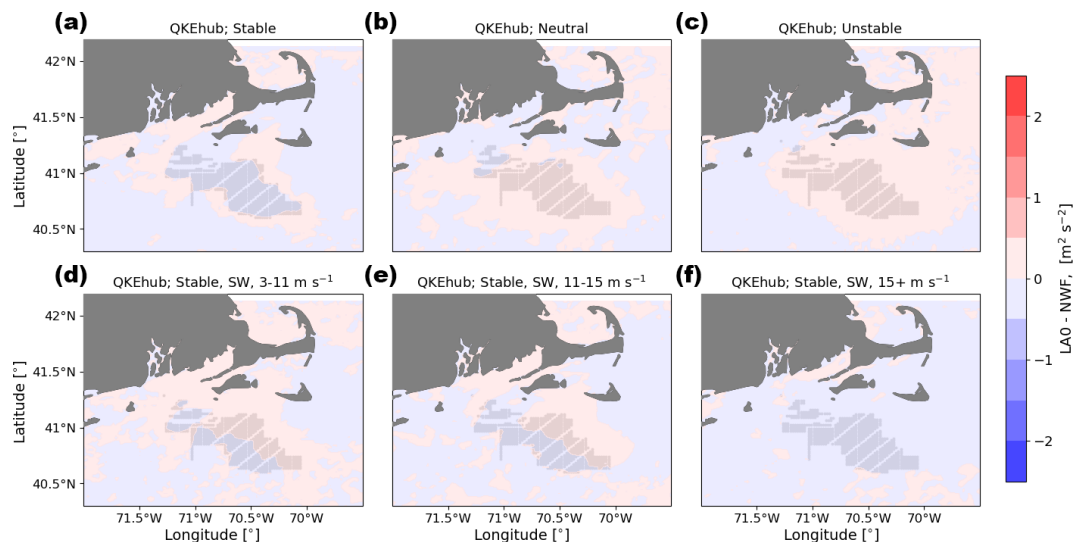
Figure 14. Mean hub-height QKE difference between the LA0 and NWF simulations in (a) stable conditions, (b) neutral conditions, (c) unstable conditions, (d) 3\text{--}11\text{ m s}^{-1} , (e) 11\text{--}15\text{ m s}^{-1} , and (f) 15+\text{ m s}^{-1} . Panels (d), (e), and (f) are only during times with stable conditions and southwest winds. Turbines are marked in gray.
