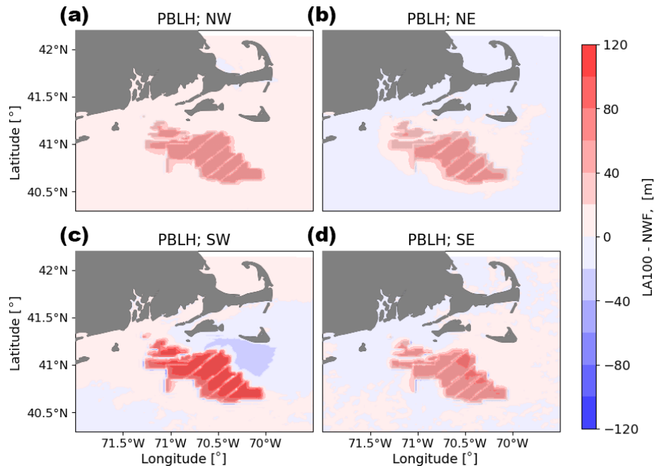
Figure B2. Mean PBLH difference between the LA100 and NWF simulations for (a) NW, (b) NE, (c) SW, and (d) SE wind directions. Turbines are marked in gray.
