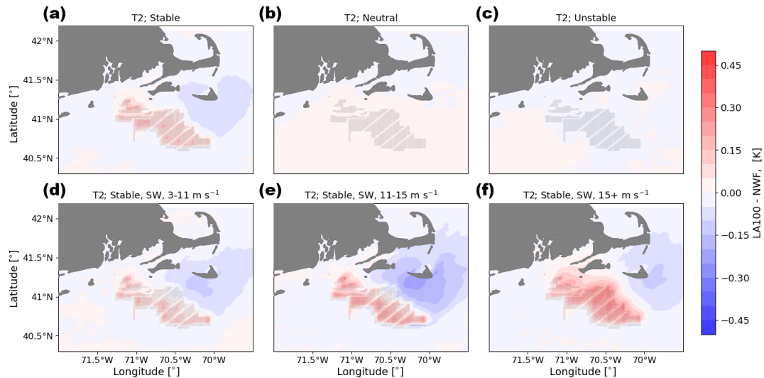
Figure 17. Mean 2 m temperature difference between the LA100 and NWF simulations in (a) stable conditions, (b) neutral conditions, (c) unstable conditions, (d) 3\text{--}11\text{ m s}^{-1} , (e) 11\text{--}15\text{ m s}^{-1} , and (f) 15\text{+ m s}^{-1} . Panels (d), (e), and (f) are only during times with stable conditions and southwest winds. Turbines are marked in gray.
