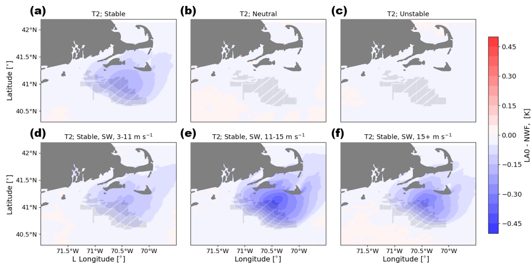
Figure 18. Mean 2 m temperature difference between the LA0 and NWF simulations in (a) stable conditions, (b) neutral conditions, (c) unstable conditions, (d) 3\text{--}11\text{ m s}^{-1} , (e) 11\text{--}15\text{ m s}^{-1} , and (f) 15\text{+ m s}^{-1} . Panels (d), (e), and (f) are only during times with stable conditions and southwest winds. Turbines are marked in gray.
