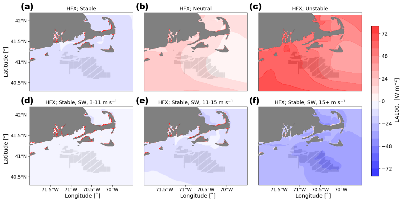
Figure C2. Mean surface heat flux for the LA100 simulation in (a) stable conditions, (b) neutral conditions, (c) unstable conditions, (d) 3–11 m s -1 , (e) 11–15 m s -1 , and (f) 15+ m s -1 . Panels (d), (e), and (f) are only during times with stable conditions and southwest winds. Turbines are marked in gray.
