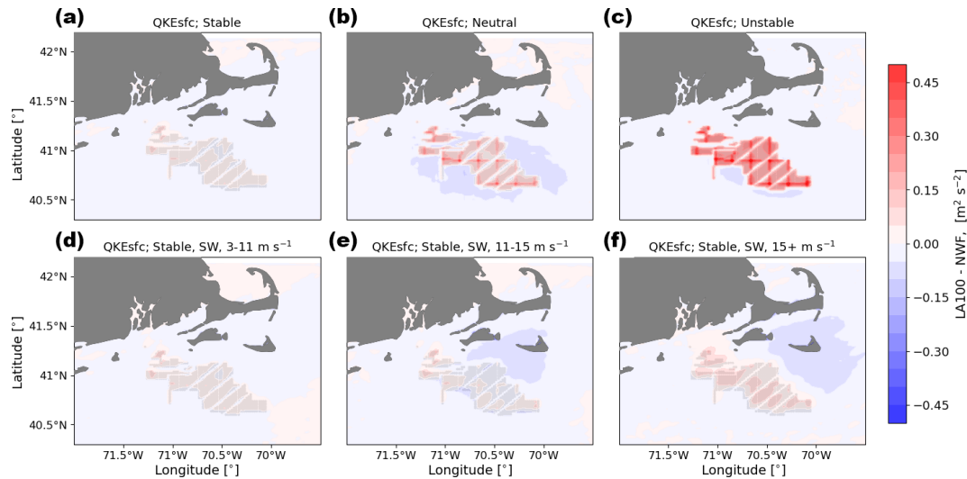
Figure 15. Mean surface QKE difference between the LA100 and NWF simulations in (a) stable conditions, (b) neutral conditions, (c) unstable conditions, (d) 3\text{--}11\text{ m s}^{-1} , (e) 11\text{--}15\text{ m s}^{-1} , and (f) 15+\text{ m s}^{-1} . Panels (d), (e), and (f) are only during times with stable conditions and southwest winds. Turbines are marked in gray.
