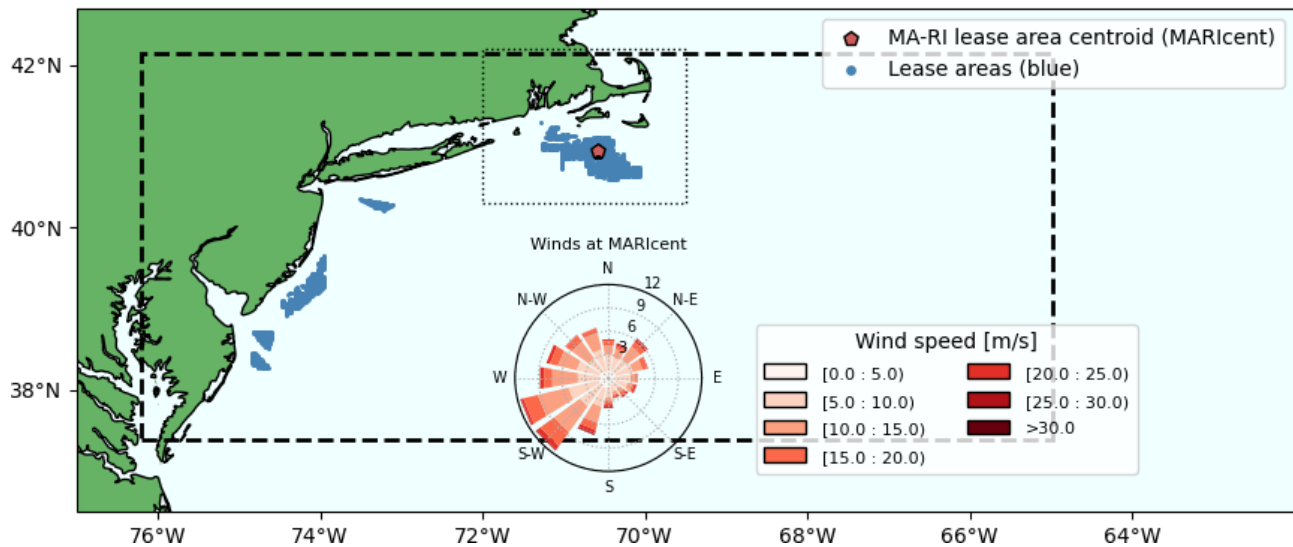
Figure 1. Simulation domain, including turbine locations and a wind rose near the centroid of the Massachusetts–Rhode Island lease area (MARcent). The MARcent location is marked in red. The turbine locations are shaded, and all wind plants included in the lease area simulations are in blue. The boundary of the NOW-WAKES innermost domain is outlined by the dashed black line. The dotted gray line indicates the region of interest for this study. The wind rose shows the wind speed (shading) and direction (angle) at 130 m over the 1 year modeled in NOW-WAKES. The distance from the center of the rose indicates the percentage of values in each bin.
