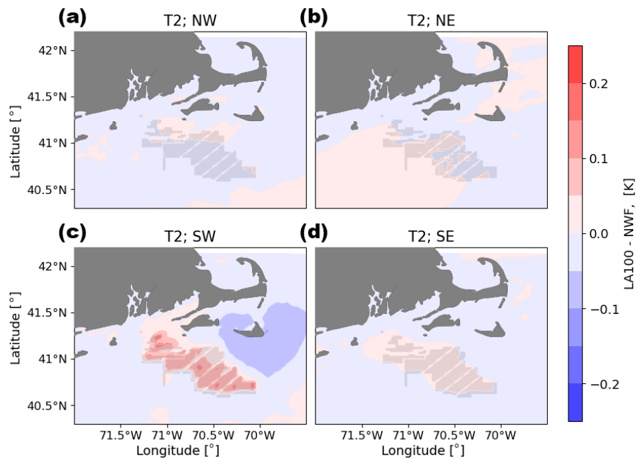
Figure B3. Mean 2 m temperature difference between the LA100 and NWF simulations for (a) NW, (b) NE, (c) SW, and (d) SE wind directions. Turbines are marked in gray.
