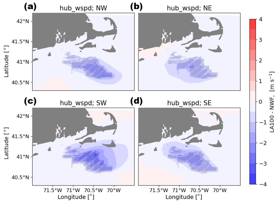
Figure B1. Mean hub-height wind speed difference between the LA100 and NWF simulations for (a) NW, (b) NE, (c) SW, and (d) SE wind directions. Turbines are marked in gray.
