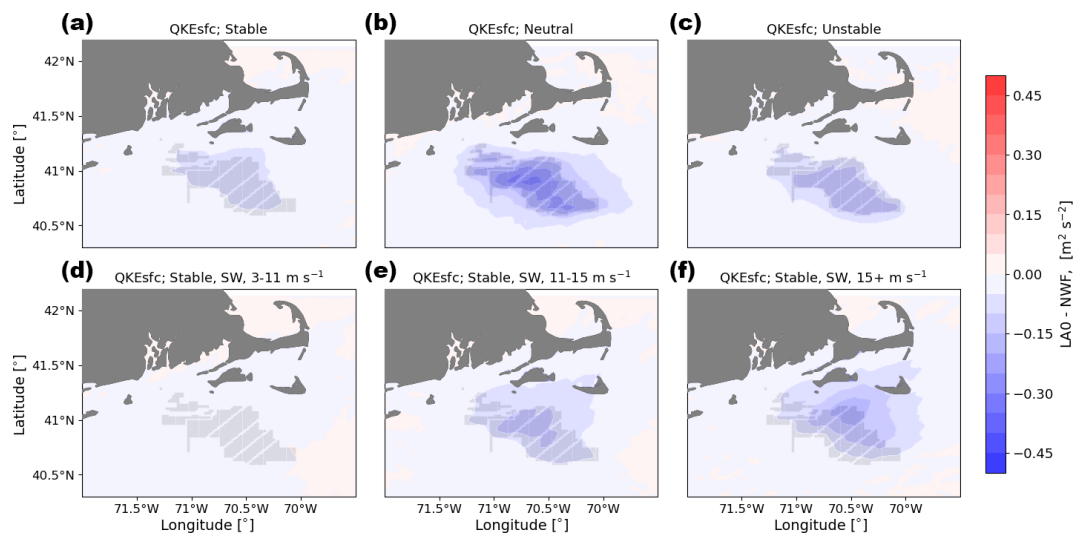
Figure 16. Mean surface QKE difference between the LA0 and NWF simulations in (a) stable conditions, (b) neutral conditions, (c) unstable conditions, (d) 3\text{--}11\text{ m s}^{-1} , (e) 11\text{--}15\text{ m s}^{-1} , and (f) 15+\text{ m s}^{-1} . Panels (d), (e), and (f) are only during times with stable conditions and southwest winds. Turbines are marked in gray.
