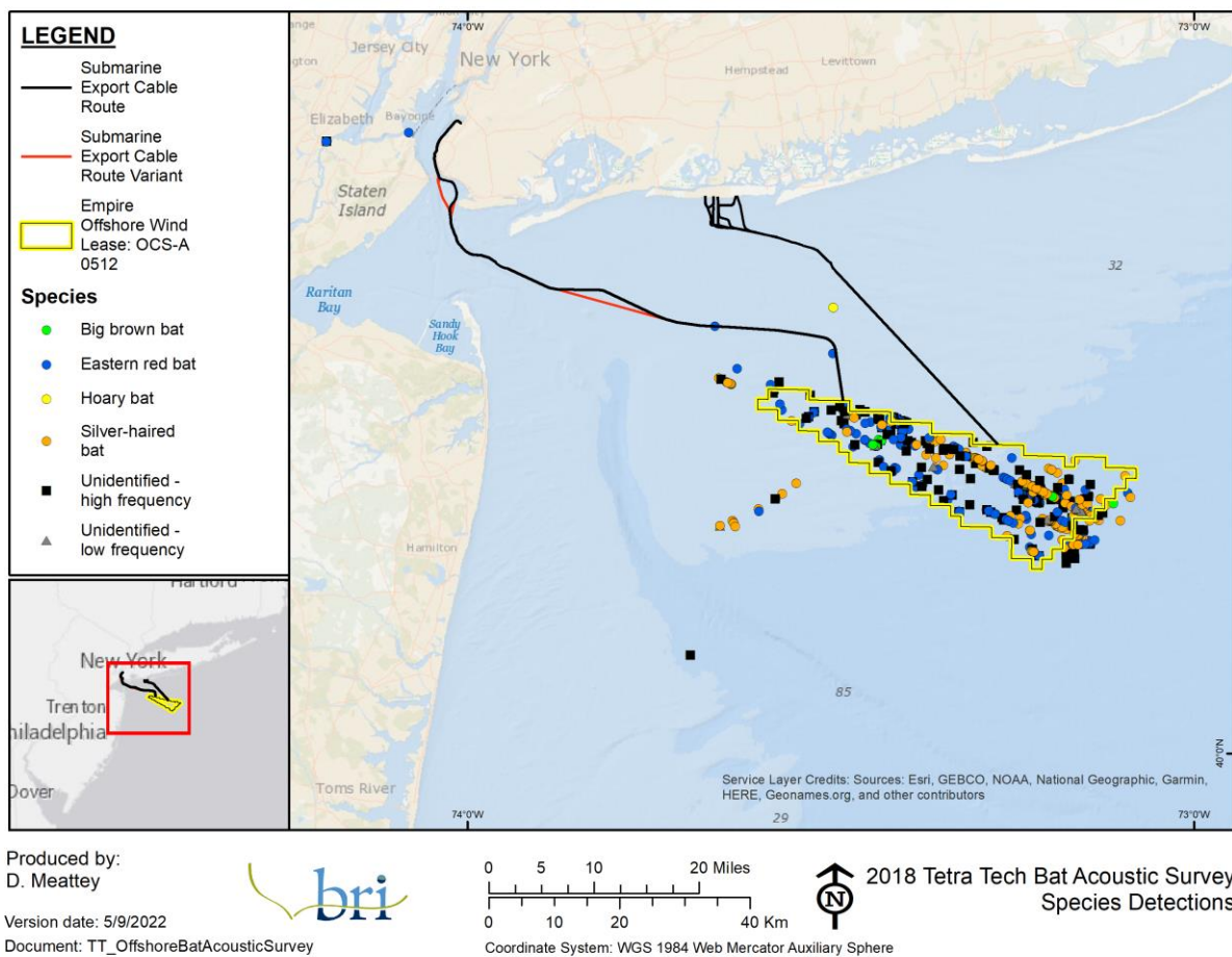
Figure 3-1. Bat occurrences in the Lease Area detected during offshore acoustic surveys conducted by Tetra Tech in 2018 (Tetra Tech 2019).
