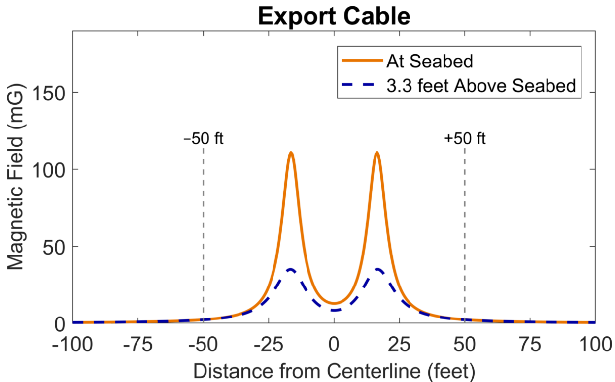
Figure C-1. Calculated magnetic-field levels in seawater above the submarine export cable for a 4-ft (1.2 m) burial depth and average loading.
