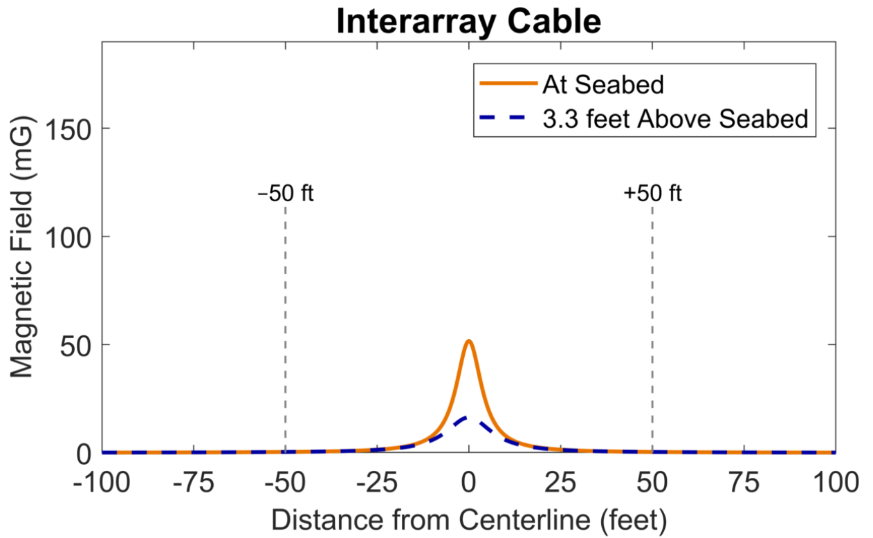
Figure C-2. Calculated magnetic-field levels in seawater above the interarray cable for a 4-ft (1.2 m) burial depth and average loading.
