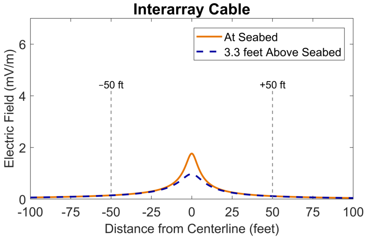
Figure C-4. Calculated electric-field levels in seawater above the interarray cable for a 4-ft (1.2 m) burial depth and average loading.
