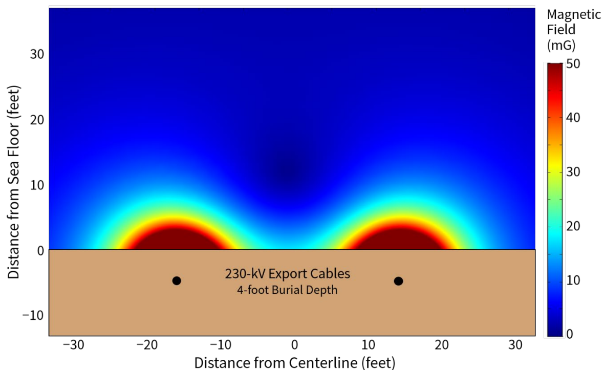
Figure 2. Calculated magnetic-field levels in seawater above the submarine export cable for 4-ft (1.2-m) burial depth and average loading.
