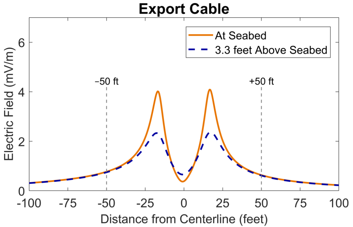
Figure C-3. Calculated electric-field levels in seawater above the submarine export cable for a 4-ft (1.2 m) burial depth and average loading.
