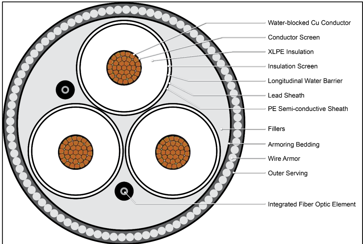
Figure A-1. Representative cross-section of the three-core submarine export cable.
