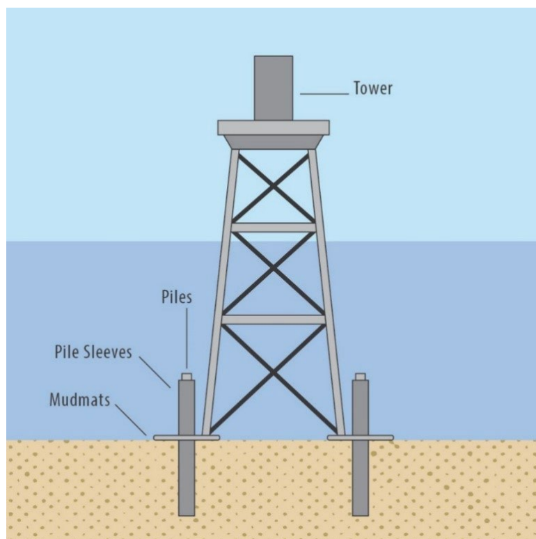
Figure 2-4. Jacket foundation
