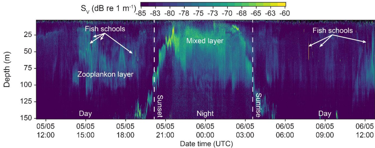
Figure 9 24 h echogram of volume backscattering strength ( S_v ) collected by Sailbuoy Echo 2 on 5-6 May 2023 showing the DVM of the mixed layer.
