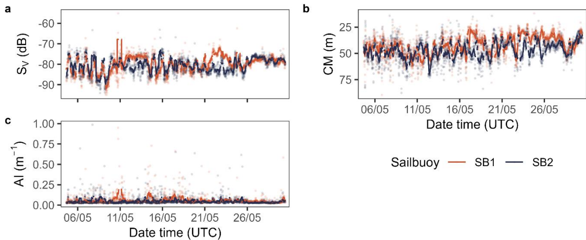
Figure 10 Echo-metrics throughout the entire survey period for each SB (colours), including (a) mean S_v , (b) centre of mass, and (c) aggregation index. The dots show the 15-minute average value, and the lines represent the rolling mean (rolling window of 20 samples).
