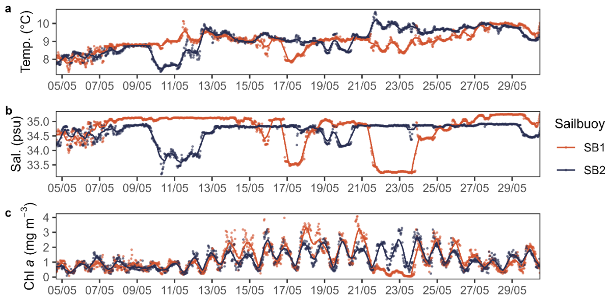
Figure 7 Surface (a) temperature, (b) salinity, and (c) chlorophyll a from SB Echo 1 (red line) and Echo 2 (blue line) during the Hywind Tampen survey. The dots show the raw data, and the lines represent the rolling mean (rolling window of 20 samples).
