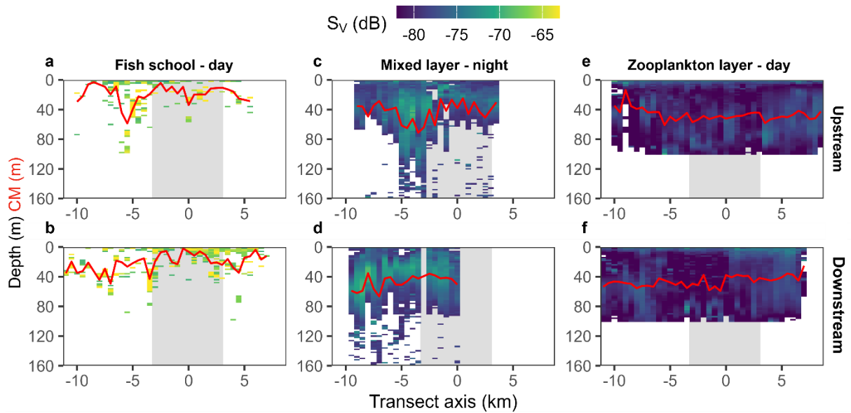
Figure 12 Synthetic echogram of (a, b) fish schools during the daytime, (c, d) mixed layer during nighttime, and (e, f) zooplankton layer during the daytime of the (a, c, e) upstream and (b, d, f) downstream transects along the sampling axes perpendicular to the main SE current direction. The grey area indicates the centre of the transect corresponding to the width of the farm (see Figure 5). The red line indicates the centre of mass (CM) of each group per transect.
