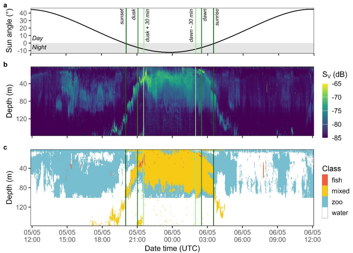
Figure 3 (a) Sun angle in relation to the horizon ( 0^\circ ) for the location of SB Echo 2 on the 5 and 6 May 2023. (b) Volume backscattering strength ( S_V ) echogram and (c) classified echogram. The vertical bars indicate the sunrise and sunset (dark green), dawn and dusk (green), and dawn and dusk \pm 30 min (light green) and were used for acoustic classification.
