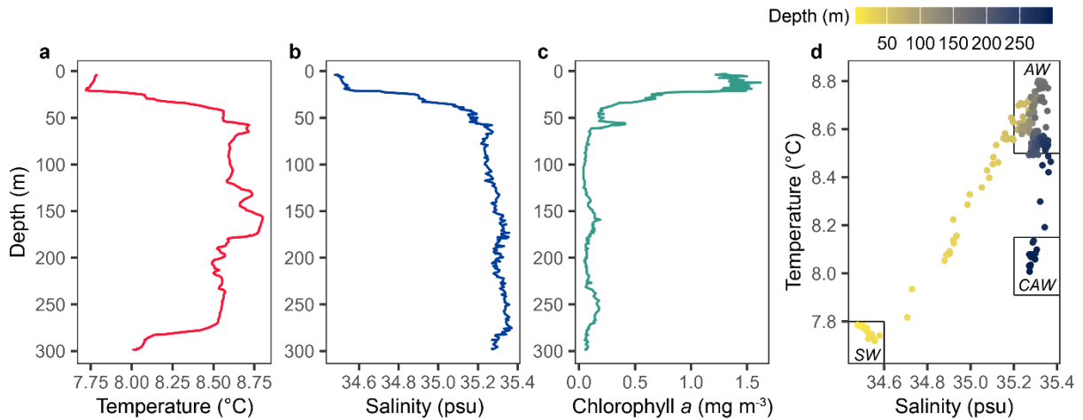
Figure 6 (a) Temperature, (b) salinity, (c) chlorophyll a profile, and (d) temperature-salinity diagram collected in the vicinity of Hywind Tampen on 5 May 2023. SW: Surface water mass; AW: Atlantic water mass; CAW: winter-cooled Atlantic water. Water mass definitions from (Svendsen et al., 1991).
