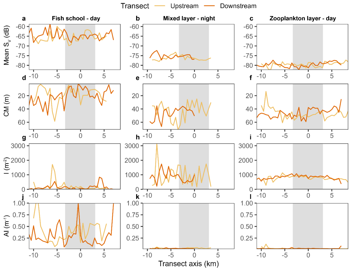
Figure 13 Averaged echo metric per transect type along the sampling axes (see Figure 5) for (a, d, g, j) fish schools, (b, e, h, k) the mixed layer and (c, f, i, l) the zooplankton layer. The echo metrics include (a, b, c) mean S_v , (d, e, f) centre of mass, (g, h, i) inertia, and (j, k, l) aggregation index. The vertical grey shadowed area shows the width of the farm along the direction of the sampling axis. farm
