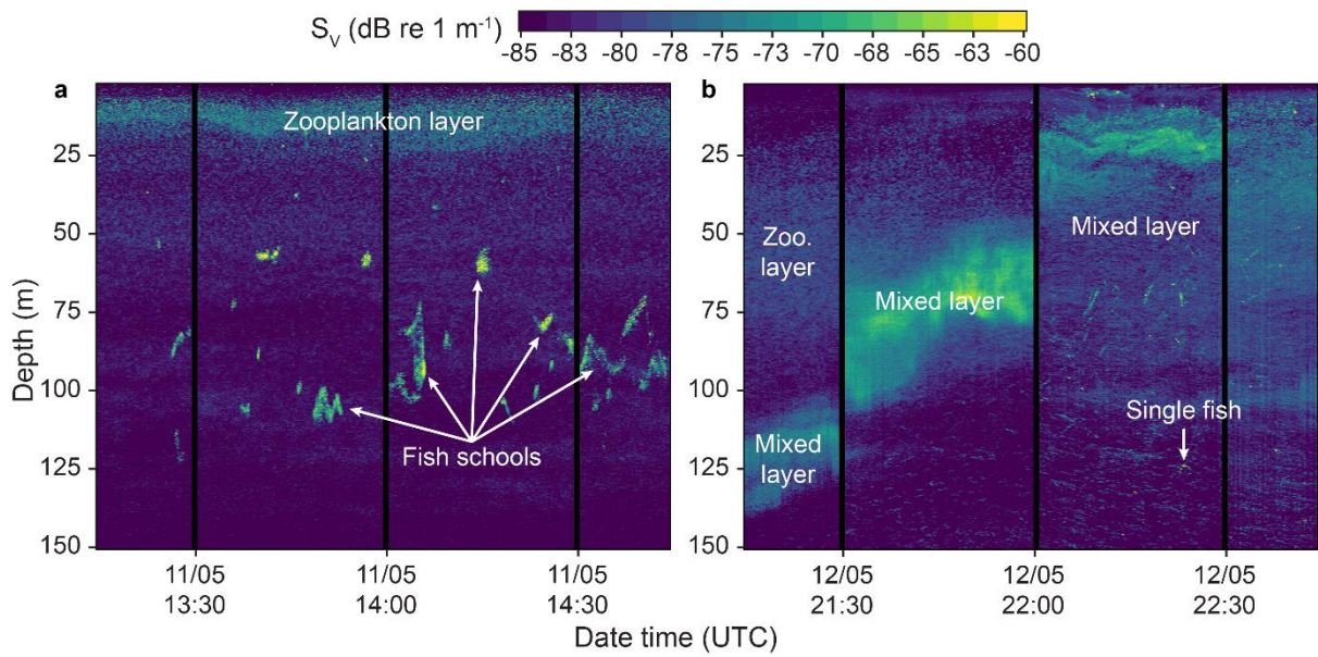
Figure 8 Zoom on echogram of volume backscattering strength ( S_v ) showing (a) a zooplankton layer and fish schools during daytime and (b) the ascent of a mixed scattering layer and single fish at dusk.
