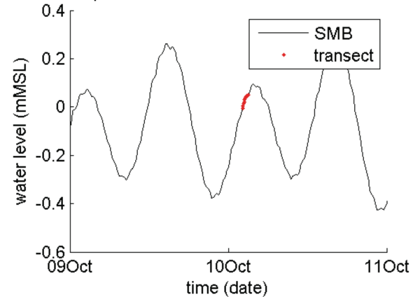
period of transect 22 relative to tide
