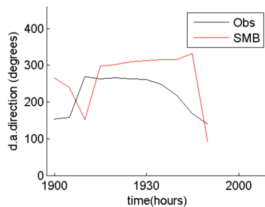
VMADCP transect 14 vs model :RMS= 86.90degrees
