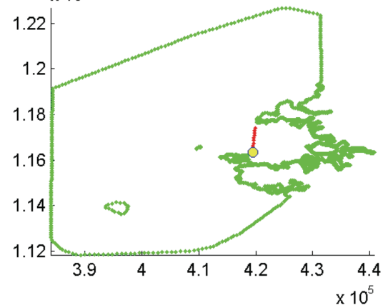
period of transect 22 relative to tide
