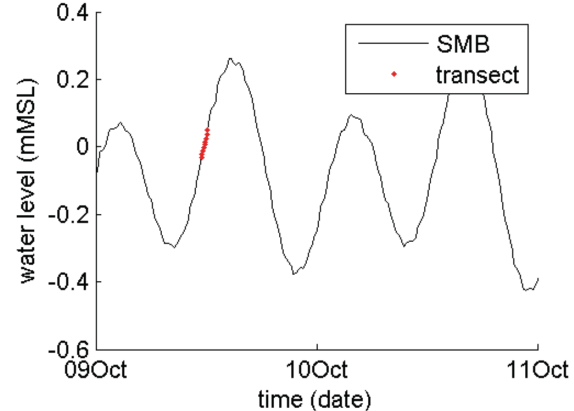
period of transect 5 relative to tide
