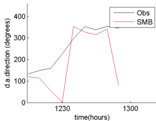
VMADCP transect 6 vs model :RMS= 123.82degrees
