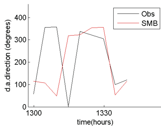
VMADCP transect 7 vs model :RMS= 172.32degrees
