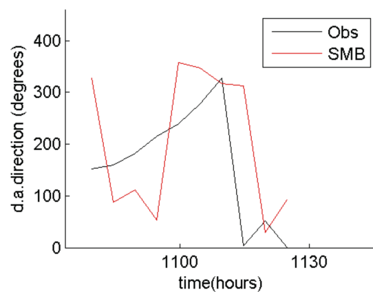
VMADCP transect 4 vs model :RMS= 138.09degrees
