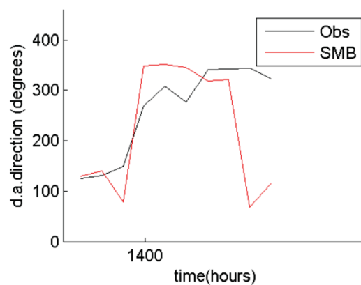
VMADCP transect 8 vs model :RMS= 117.39degrees
