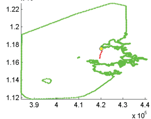
period of transect 3 relative to tide
