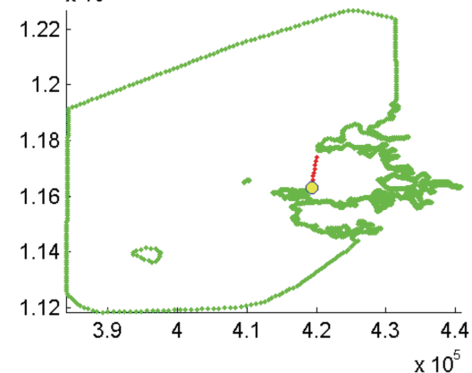
period of transect 6 relative to tide
