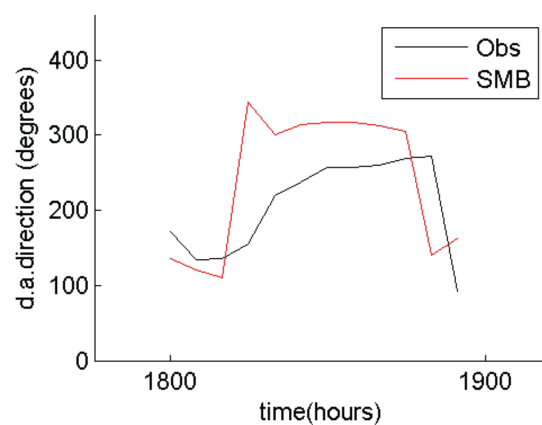
VMADCP transect 13 vs model :RMS= 83.60degrees
