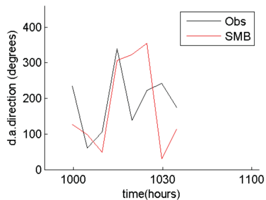
VMADCP transect 3 vs model :RMS= 121.14degrees
