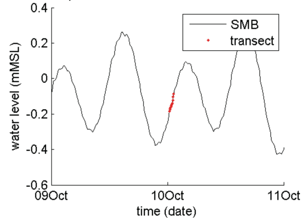
period of transect 20 relative to tide
