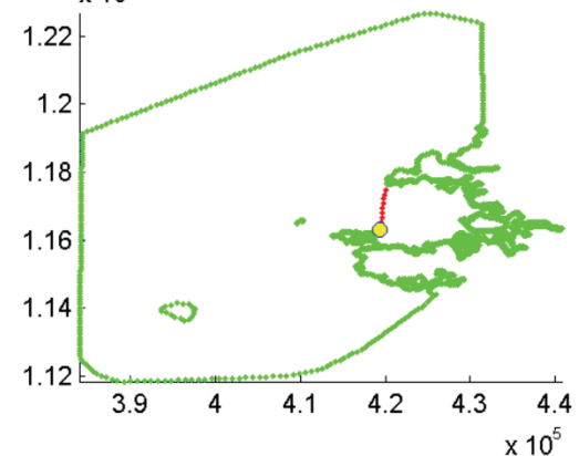
period of transect 8 relative to tide
