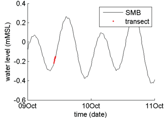
period of transect 3 relative to tide
