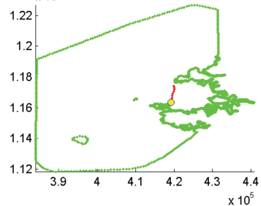
period of transect 2 relative to tide
