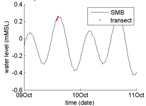
period of transect 8 relative to tide
