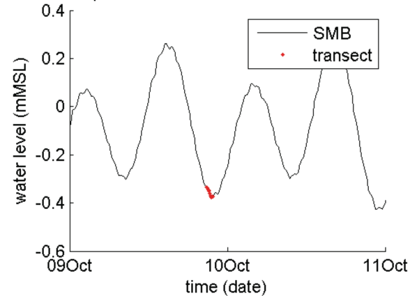
period of transect 16 relative to tide
