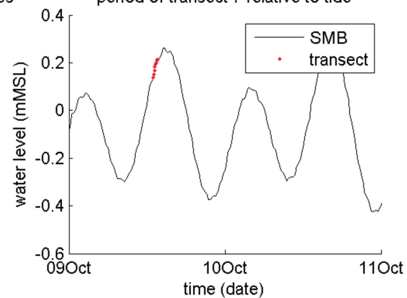
period of transect 7 relative to tide
