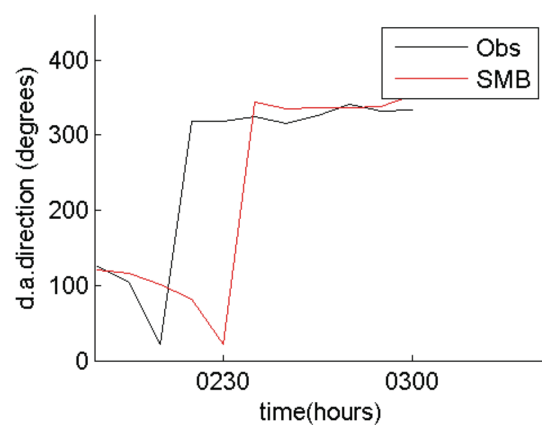
VMADCP transect 22 vs model :RMS= 117.40degrees
