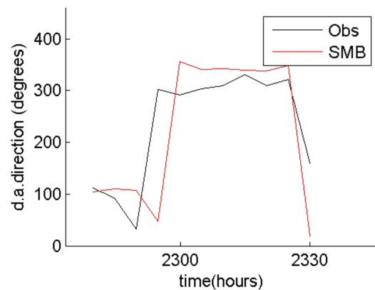
VMADCP transect 18 vs model :RMS= 94.60degrees
