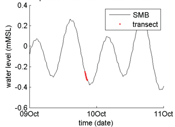
period of transect 15 relative to tide
