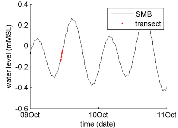
period of transect 4 relative to tide
