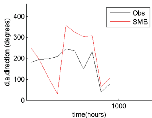
VMADCP transect 2 vs model :RMS= 98.55degrees
