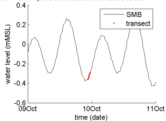
period of transect 18 relative to tide
