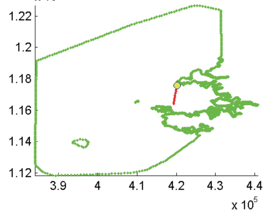
period of transect 13 relative to tide
