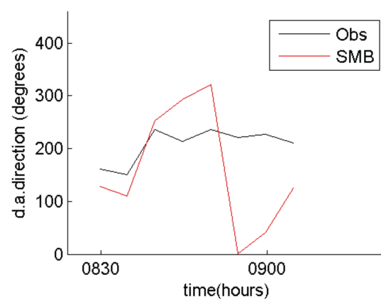
VMADCP transect 1 vs model :RMS= 115.69degrees
