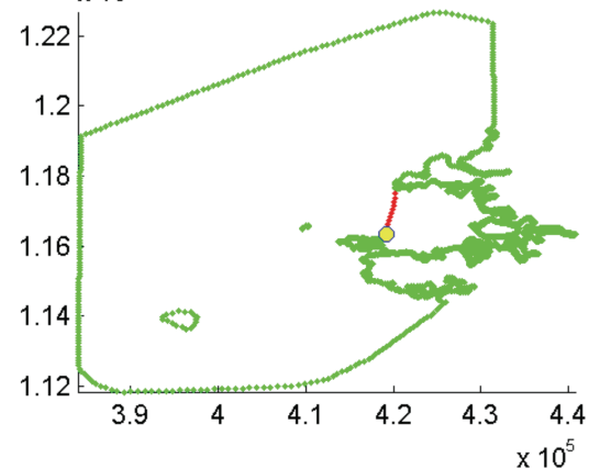
period of transect 10 relative to tide
