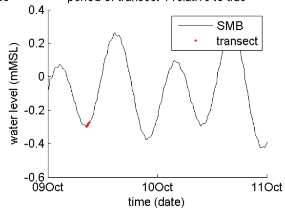
period of transect 1 relative to tide
