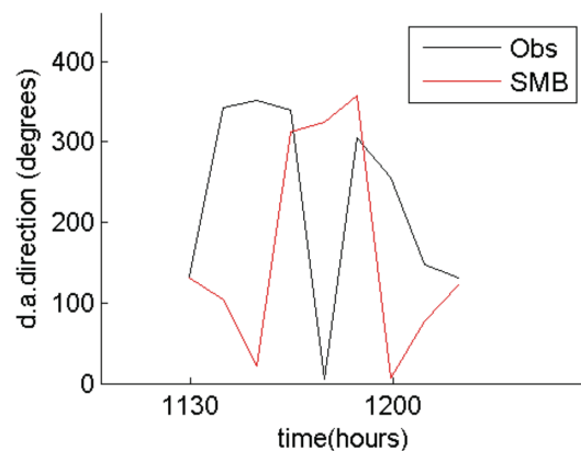
VMADCP transect 5 vs model :RMS= 193.67degrees
