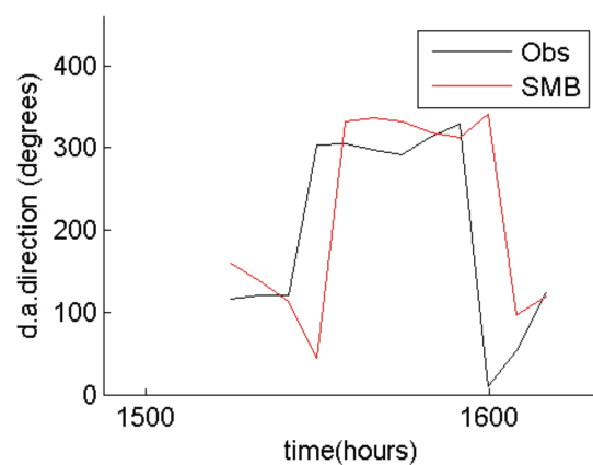
VMADCP transect 10 vs model :RMS= 124.34degrees
