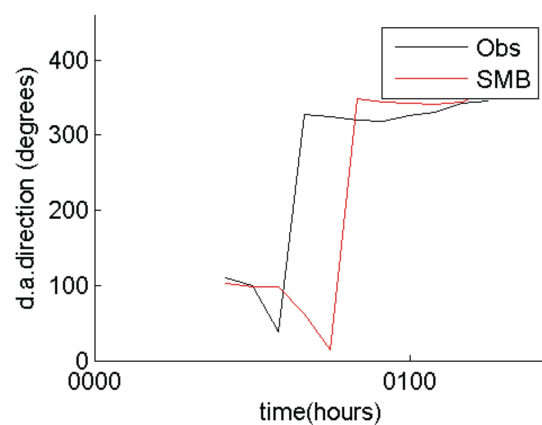
VMADCP transect 20 vs model :RMS= 125.00degrees
