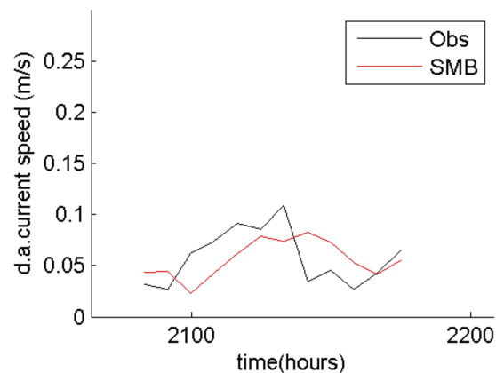
VMADCP transect 16 vs model :RMS= 97.33degrees
