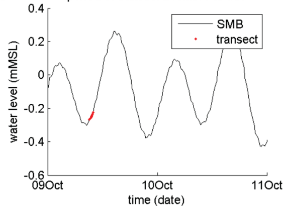
period of transect 2 relative to tide
