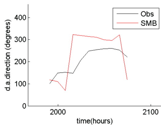
VMADCP transect 15 vs model :RMS= 84.16degrees
