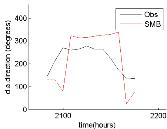
VMADCP transect 16 vs model :RMS= 97.33degrees
