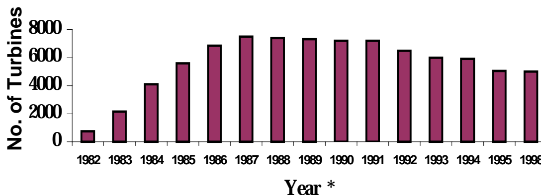
Figure 4.1 Wind Turbine Development at Altamont Pass
