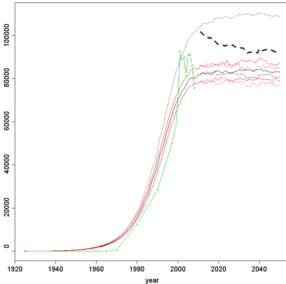
Figure 5.1.6 Counted (green circles and line) and modelled population trend for lesser black-backed gull in number of pairs (black line=median; red lines=25 and 75 percentile; black broken line= floater pairs 30%) (source www.sovon.nl ). With the effect of worst-case increased mortality, number of yearly collisions based on a scenario that the population reach a 0-growth status (resulting in a number of potential victims of 1,750 female birds, implying a scenario of more than 20 new wind farms in offshore waters).
