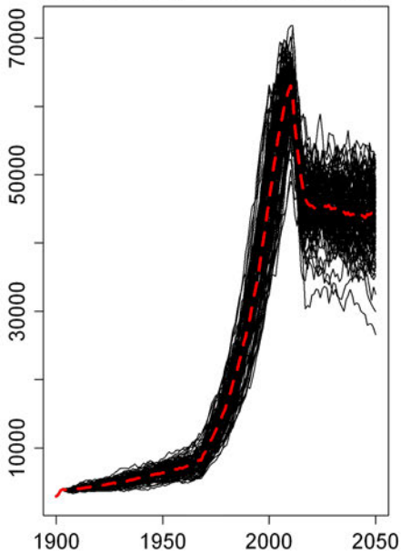
All realizations (r=100) for breeding pairs
