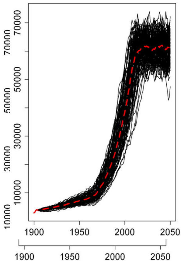
All realizations (r=100) for breeding pairs
