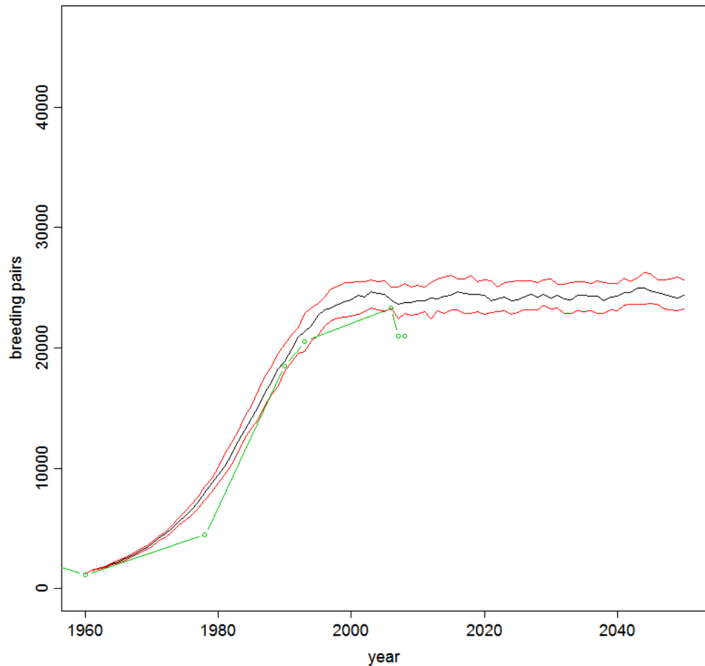
Figure 5.1.1 Counted (green circles and line) and modelled (black line=median; red lines=25 and 75 percentile) population trend for cormorant.
