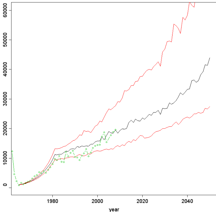
Figure 5.1.7 Counted (green circles and line) and modelled (black line=median; red lines=25 and 75 percentile) population trend for Sandwich tern with no floaters.
