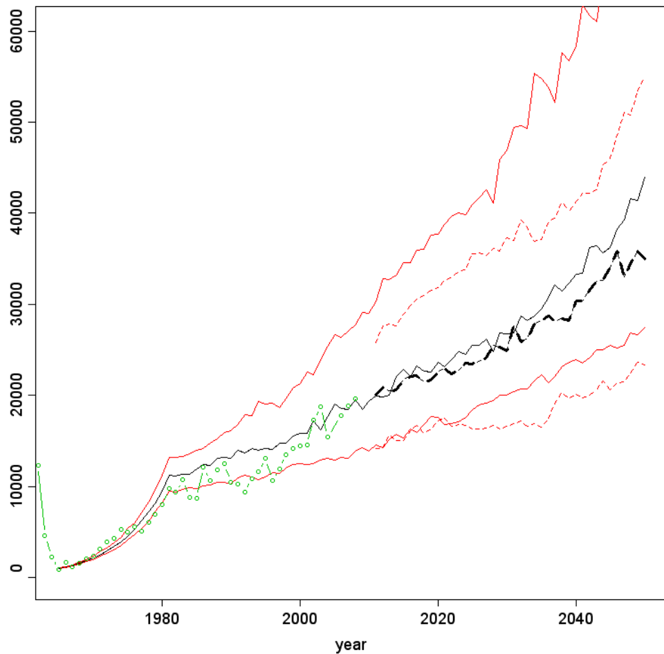
Figure 5.1.8 Counted (green circles and line) and modelled (black line=median; red lines=25 and 75 percentile) population trend for Sandwich tern with no floaters. With the effect of worst-case increased mortality, number of yearly collisions based on band model calculation ( n victims = 150) for a scenario with 11 wind farms (like OWEZ) in offshore waters.
