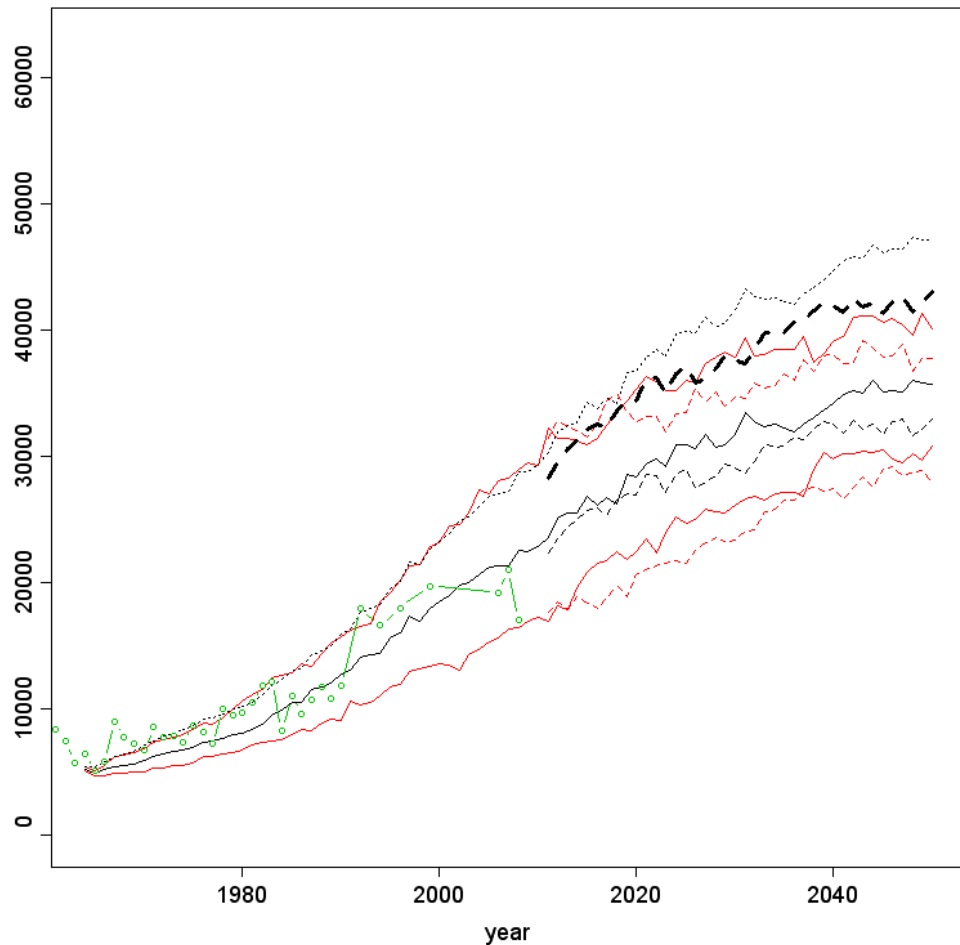
Figure 5.1.10 Counted (green circles and line) and modelled (black line=median; red lines=25 and 75 percentile) population trend for Sandwich tern with 30% floaters. With the effect of worst case increased mortality, number of yearly collisions based on band model calculation ( n victims = 73) for a scenario with 11 wind farms like OWEZ in offshore waters.
