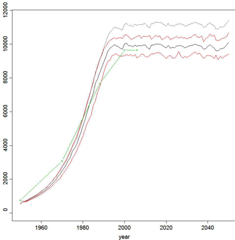
Figure 5.1.13 Counted (green circles and line) and modelled (black line=median; red lines=25 and 75 percentile) population trend for great skua, with an assumed 10% floater population (dotted line).
