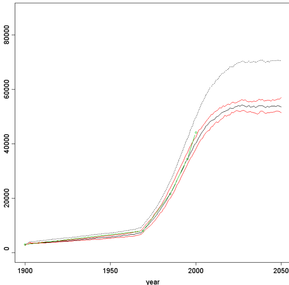
Figure 5.1.11 Counted (green circles and line) and modelled population trend for gannet on Bass Rock (black line=median; red lines=25 and 75 percentile; black broken line= floater pairs 30%).
