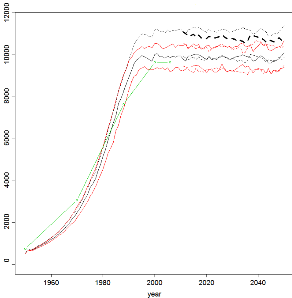
Figure 5.1.14 Counted (green circles and line) and modelled (black line=median; red lines=25 and 75 percentile) population trend for great skua, with an assumed 10% floater population (dotted line). Also depicted is the lines with the effect of worst case increased mortality due to yearly collisions based on band model calculation ( n victims = 40) for a scenario with 11 wind farms like OWEZ in offshore waters.
