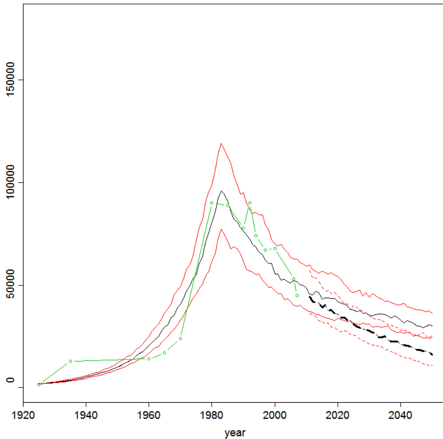
Figure 5.1.3 Counted (green circles and line) and modelled (black line=median; red lines=25 and 75 percentile) population trend for herring gull. With the effect of worst-case increased mortality, number of yearly collisions based on band model calculation ( n female victims = 700), of a scenario with 11 offshore wind farms.
