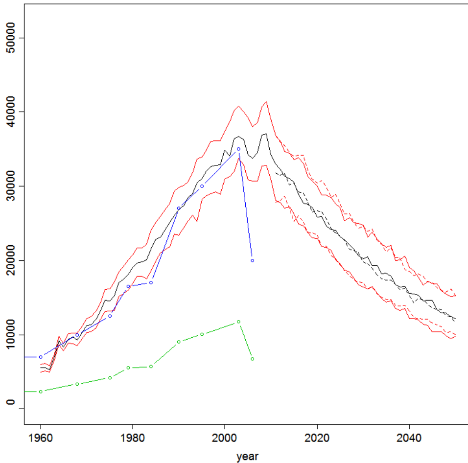
Figure 5.1.20 Counted breeding (green circles and line) and total (blue circles and line), and modelled (black line=median; red lines=25 and 75 percentile) population trend for Bewick's swan. With the effect of worst case increased mortality, number of yearly collisions based on band model calculation (n victims = 10) for a scenario with 11 wind farms like OWEZ in offshore waters.
