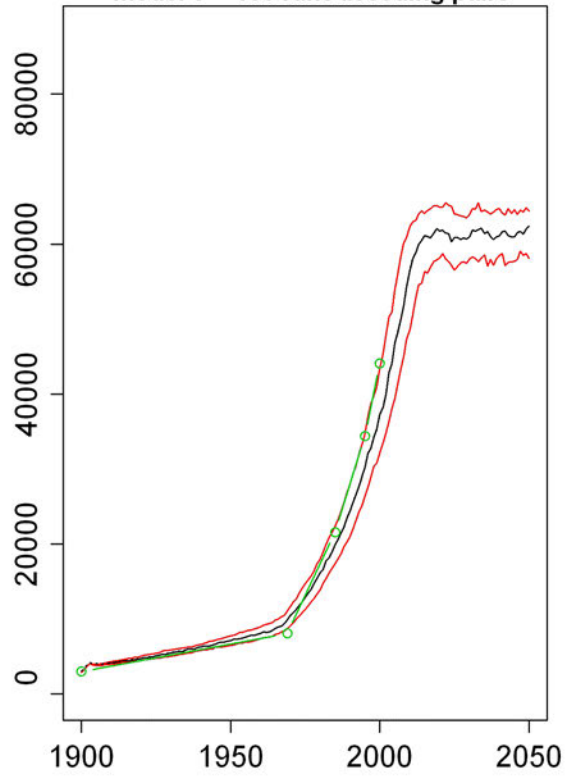
Gannet Morus bassanus - Bass Rock model 3 - 100 runs breeding pairs
