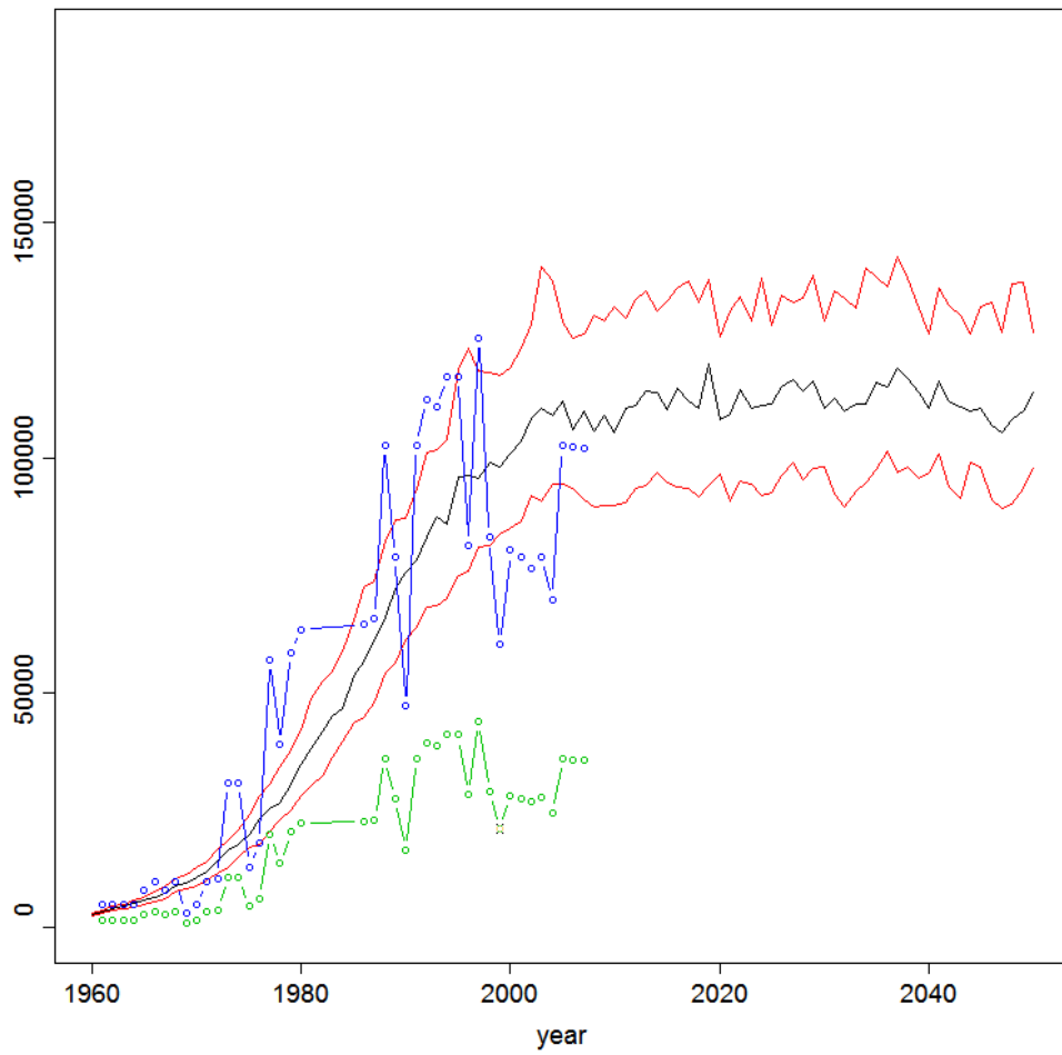
Figure 5.1.21 Counted total (blue circles and line) and modelled (black line=median; red lines=25 and 75 percentile) total population trend for brent geese. Fraction of breeding birds depicted with green circles and line.
