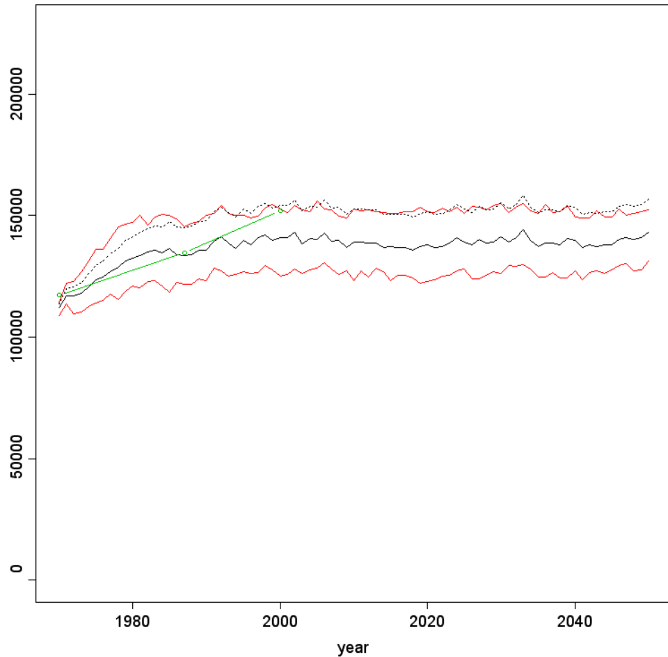
Figure 5.1.18 Counted (green circles and line) and modelled (black line=median; red lines=25 and 75 percentile) population trend for razorbill on the east coast of Scotland, with an assumed 10% floater population (fine dotted line).
