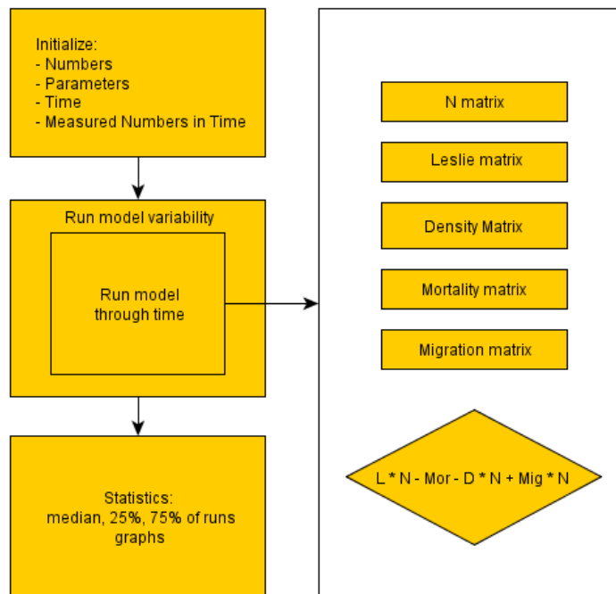
Figure 3.1.5 Flowchart of modelling process.
