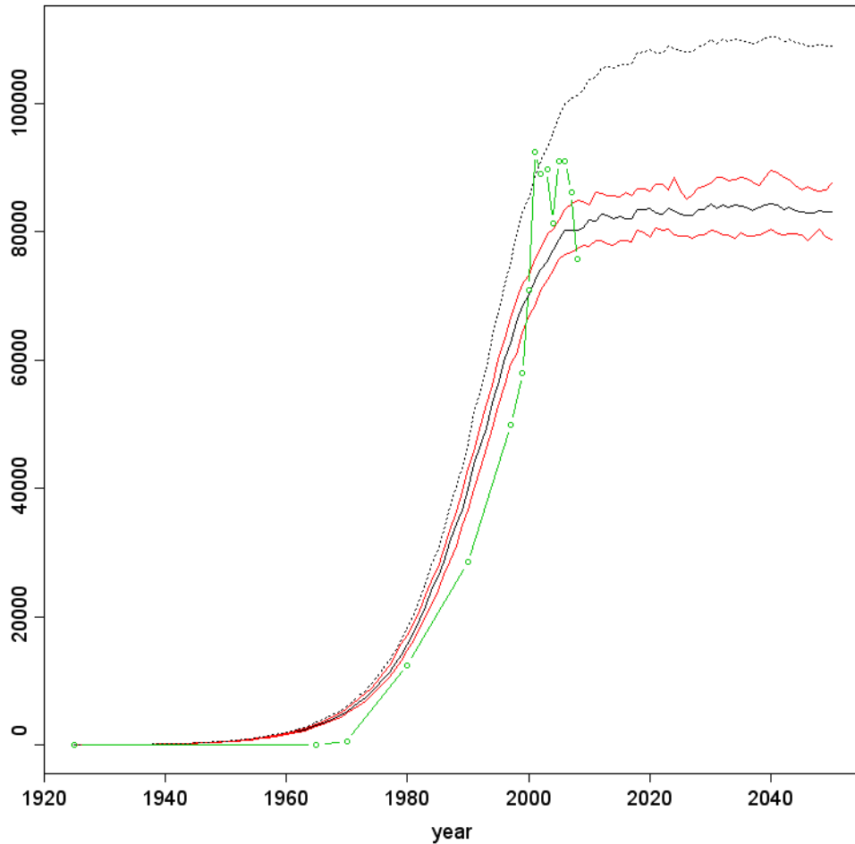
Figure 5.1.4 Counted (green circles and line) and modelled population trend for lesser black-backed gull in number of pairs (black line=median; red lines=25 and 75 percentile; black broken line= floater pairs 30%) (source www.sovon.nl ).
