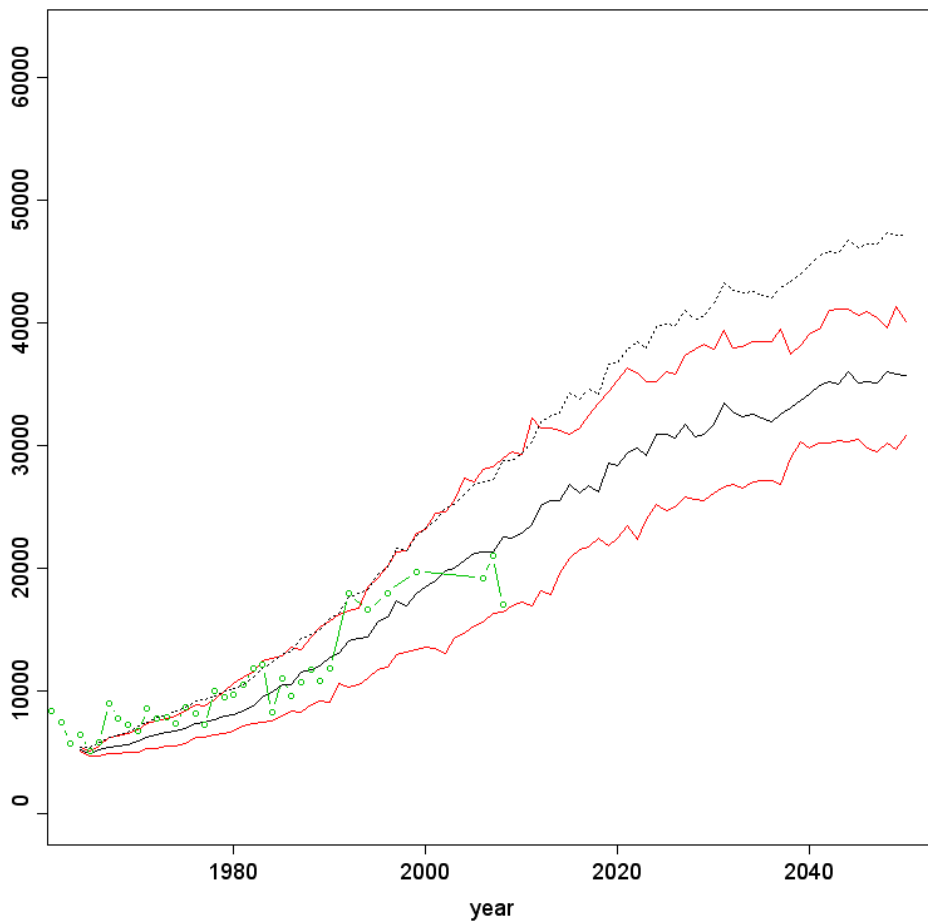
Figure 5.1.9 Counted (green circles and line) and modelled population trend for common tern (black line=median; red lines=25 and 75 percentile; black broken line= floater pairs 30%).
