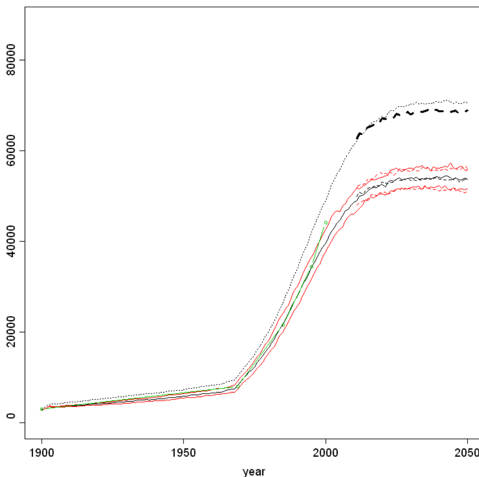
Figure 5.1.12 Counted (green circles and line) and modelled population trend for the gannet in number of pairs (black line=median; red lines=25 and 75 percentile; black broken line= floater pairs 30%). With the effect of worst case increased mortality, number of yearly collisions based on band model calculation ( n victims = 200) for a scenario with 11 wind farms like OWEZ in offshore waters.
