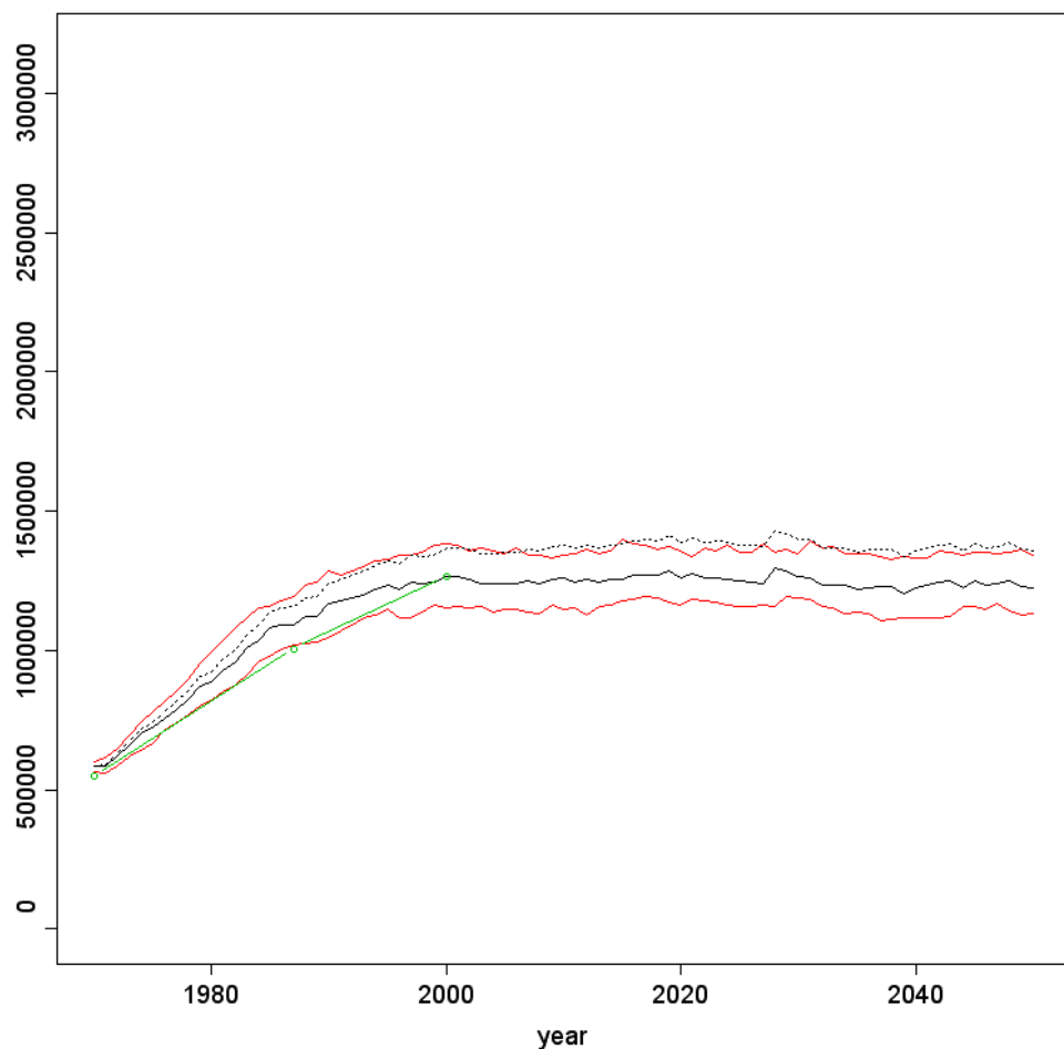
Figure 5.1.17 Counted (green circles and line) and modelled (black line=median; red lines=25 and 75 percentile) population trend for guillemot in Scotland, with an assumed 10% floater population (fine dotted line).
