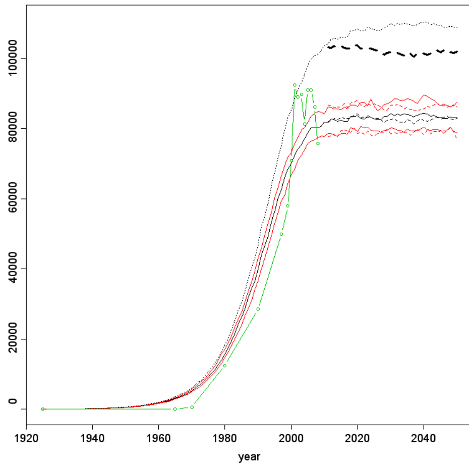
Figure 5.1.5 Counted (green circles and line) and modelled population trend for lesser black-backed gull in number of pairs (black line=median; red lines=25 and 75 percentile; black broken line= floater pairs 30%) (source www.sovon.nl ). With the effect of worst-case increased mortality, number of yearly collisions based on band model calculation ( n victims = 875) for a scenario with 11 wind farms in offshore waters.
