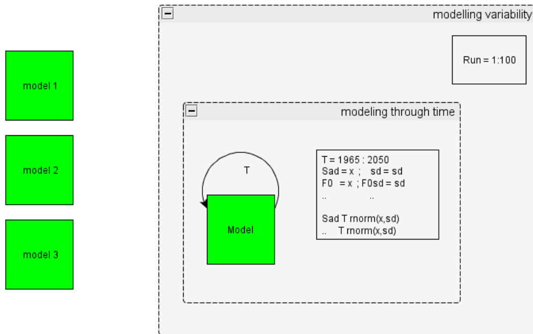
Figure 3.1.4 Framework modelling variability.
