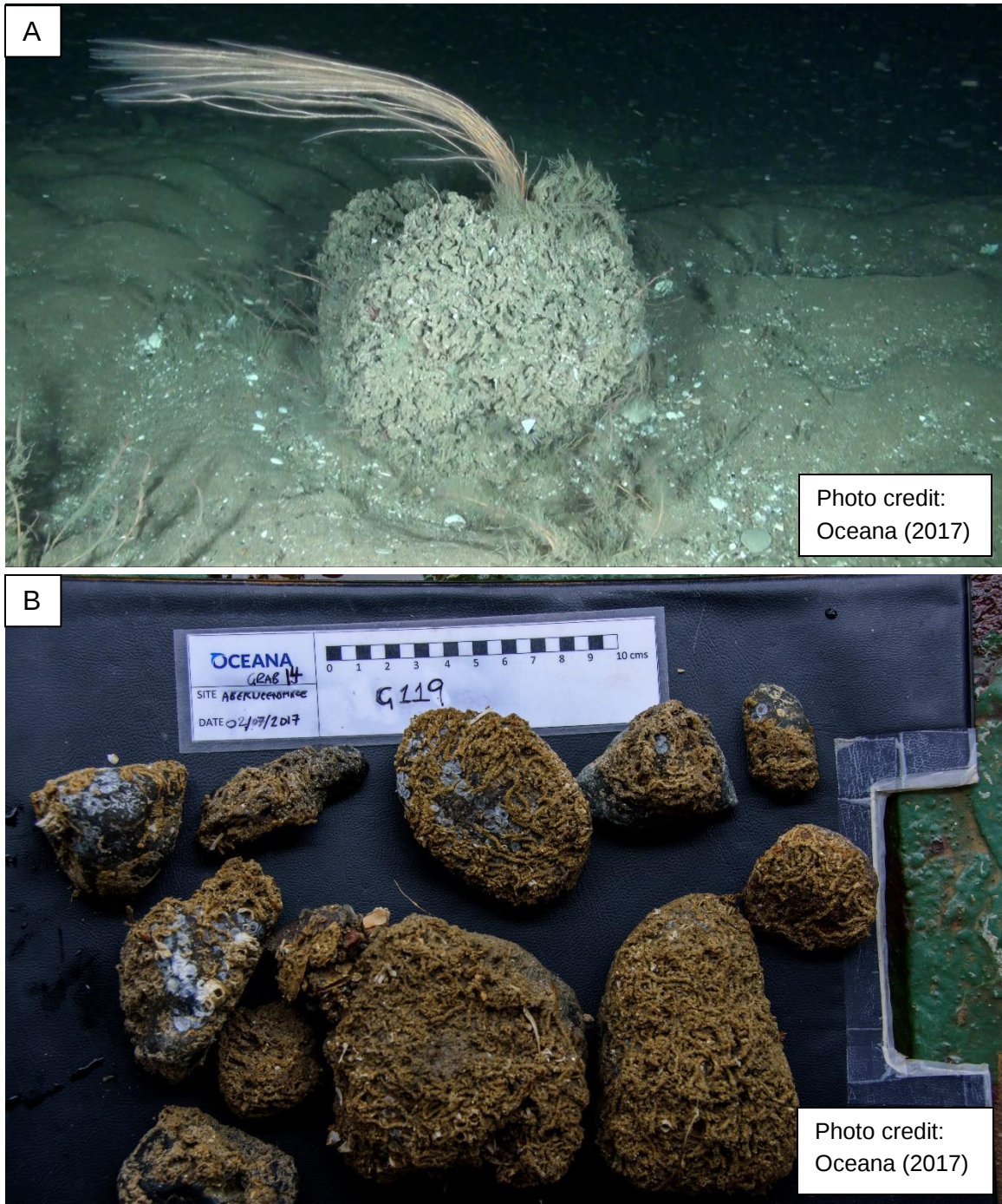
Plate 1: A) Screengrab from the ROV footage collected as part of the Oceana research cruise showing a discrete aggregation of Sabellaria spinulosa amidst an otherwise relatively featureless fine sedimentary habitat. B) Photograph of cobbles sampled during the Oceana cruise with encrusting S. spinulosa tubes.
