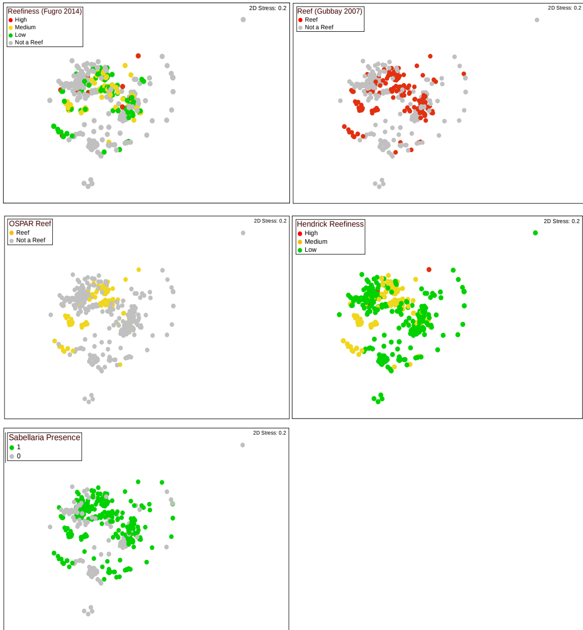
Figure 2:. A two-dimensional nMDS ordination based on the untransformed SACFOR abundance data (Table 6) extracted from video tow segments on the east coast of Scotland between 2011 and 2016. Sabellaria spinulosa abundance has been removed as well as any afaunal and outlying samples. The MDS plots are overlaid with the Sabellaria spinulosa reefiness classes as summarised in Table 8 and presented in full in Electronic Appendix 1 .
