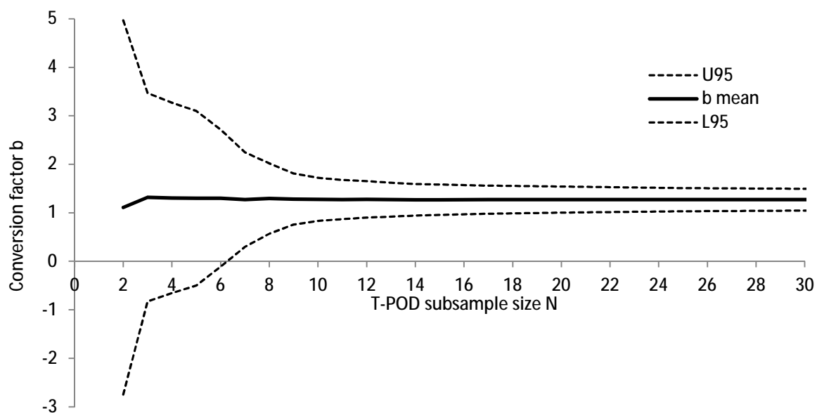
Fig. 8-6: Dependence of the 95% confidence envelope of conversion factor b on subsample size N_{sample} (envelopes are based on 1,000 permutations of N_{sample} data randomly drawn from the baseline dataset with N_{total} = 400 pairs of T-POD and C-POD data).
