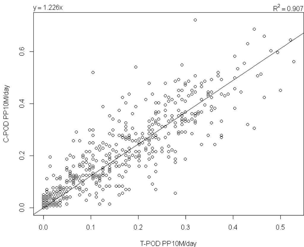
Fig. 8-2: Simple linear regression of C-POD data on T-POD data (PP10M/day) for the whole dataset (11 subsets regarding different T-POD/C-POD combinations; N = 527 ).
