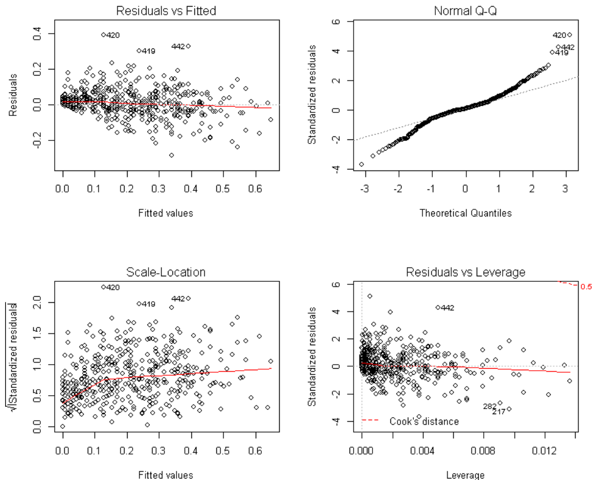
Fig. 8-3: Residuals plots for a simple linear model (LM) with all data (11 subsets regarding different T-POD/C-POD combinations; N = 527 ).
