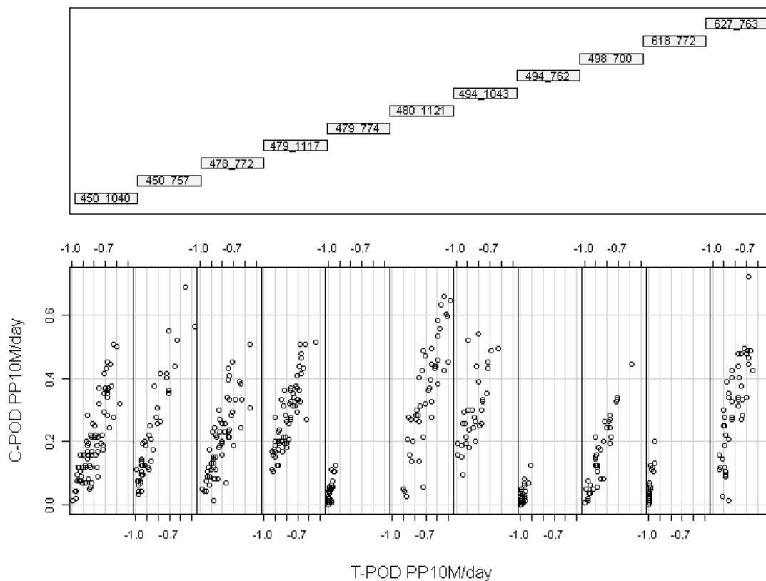
Fig. 8-4: Dot plots for 11 data subsets, each representing a T-POD/C-POD combination; for combinations “618_772”, “479_774”, and “494_762” the detection rates were always low, rendering these subsets unsuitable for assessment of a T-POD/C-POD conversion factor.
