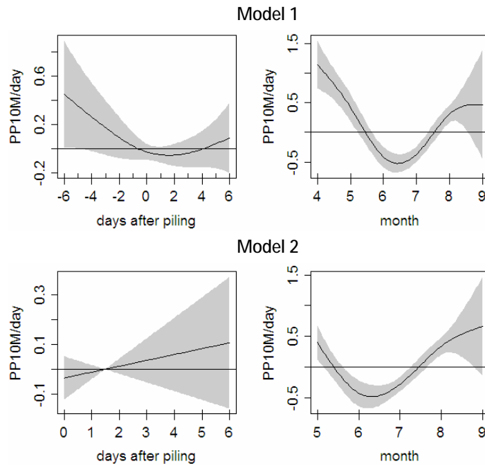
Fig. 8-12: GAM plots (2008 data with hypothetical pile-drivings) according to control model 1 and 2 (see Section 2.4.7, p. 36) for distance class 2 (stations T8 and T13), visualising the control model outcome with hypothetical pile-drivings ('days after piling') and the effect of Month on daily harbour porpoise detection rates PP10M/day (see Fig. 3-23 for further information).
