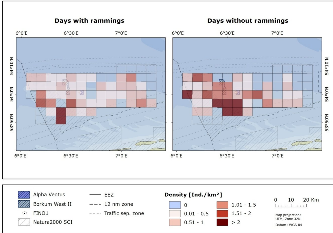
Fig. 3-8: Densities from June to August 2008 and 2009 at days with and without pile-driving.
