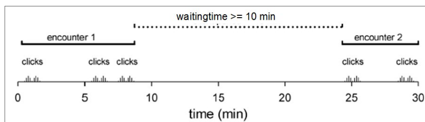
Fig. 2-22: Relationship between Encounter and Waiting time.
