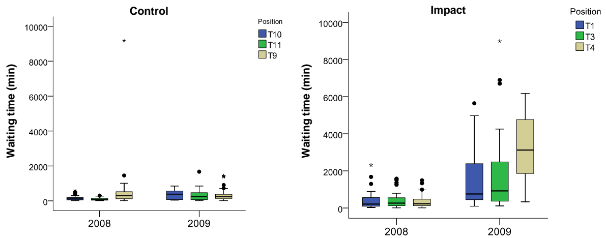
Fig. 3-30: Boxplots of the differences of the 1 st Waiting times between 2008 (Before) and 2009 (After), both for Control and Impact; these data were used for calculation of the BACI effect in Tab. 3-14.
