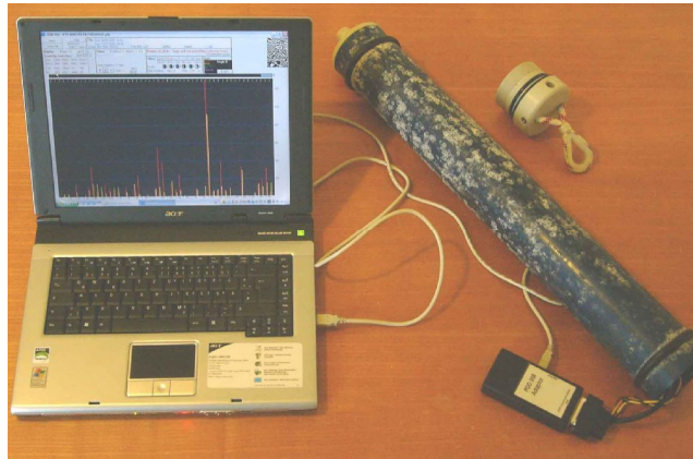
Fig. 2-18: T-POD (version 4) connected with a notebook; this configuration was used during Phase I and Phase II of the project.
