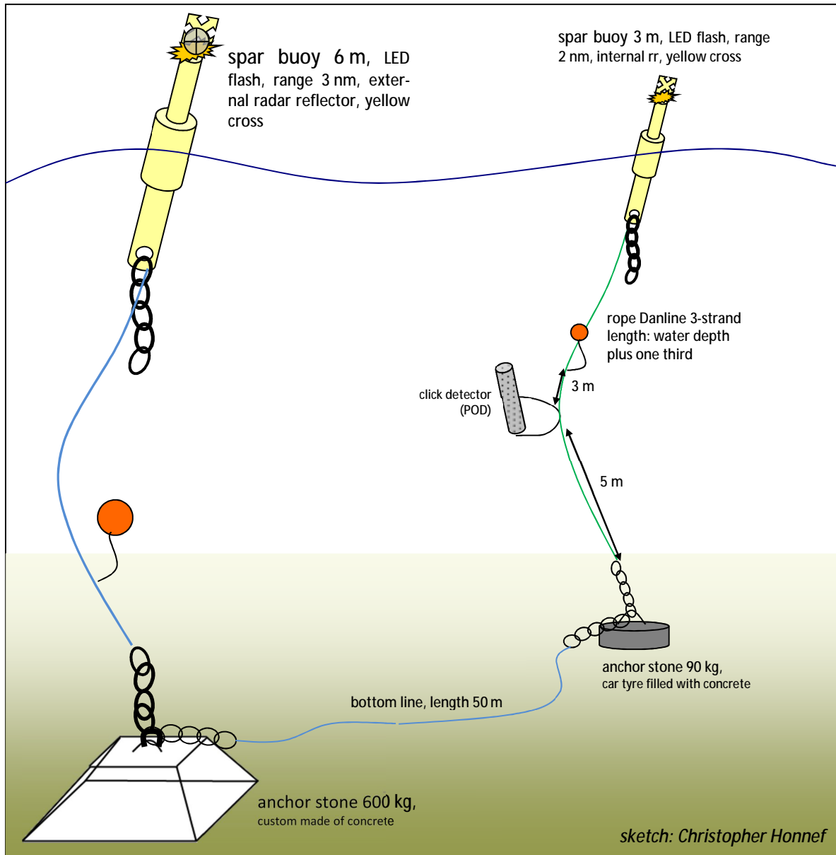
Fig. 2-20: POD system used by BioConsult SH for the alpha ventus project.
