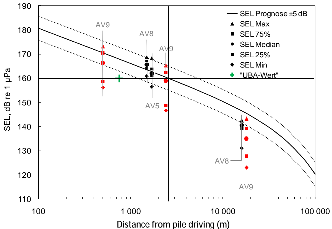
Fig. 2-5: Measured SEL at alpha ventus foundations AV5, AV8, and AV9, as well as predicted curves (after Betke & Matuschek 2011). At AV9 pile driving was conducted with and without noise mitigation system, causing higher SEL variability.
