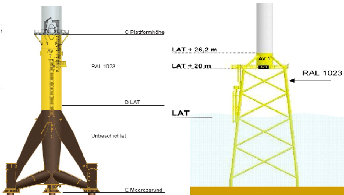
Fig. 2-3: Tripod foundations of Multibrid wind turbines (left) and Jacket foundation of Repower wind turbines (right).
