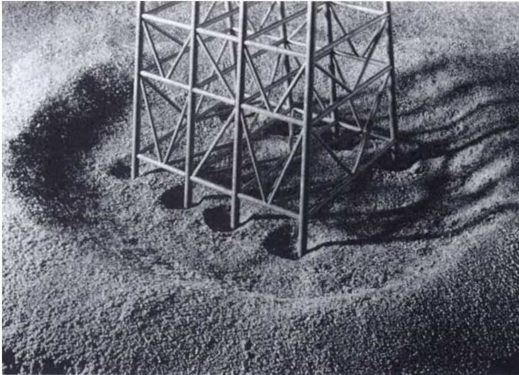
Figure 5.14 – Representation of global and local scour development around a jacket structure
