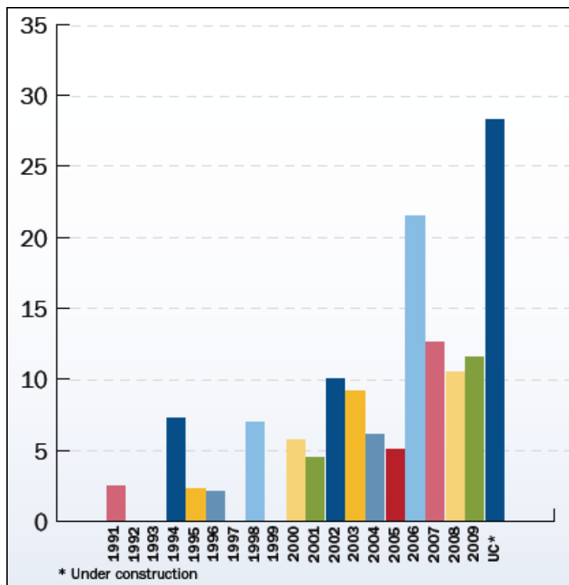
Figure 5.34 – Average European wind farm distance to shore in km, 1991-2009
