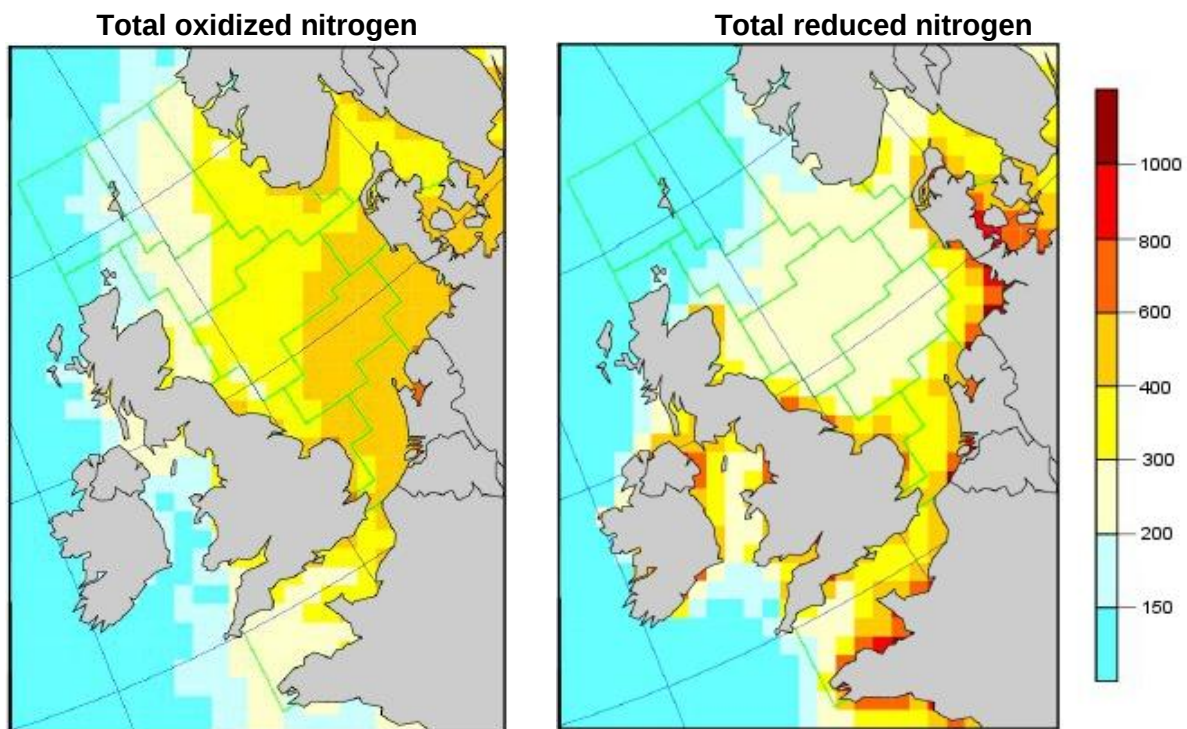
Figure A3e.2 – Estimated atmospheric deposition of nitrogen to the greater North Sea (OSPAR Region II), 2004 ( \text{mg}/\text{m}^2/\text{p.a.} )
