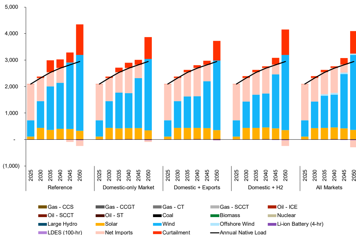
Figure 30. Prince Edward Island Generation (GWh) Across All Scenarios
