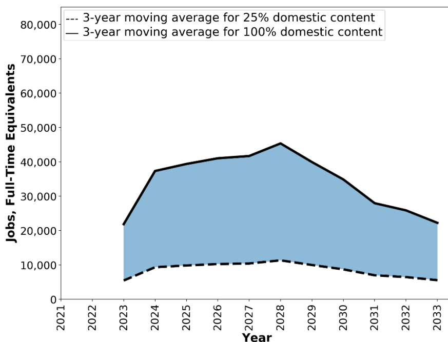
Figure B1. Moderate supply chain constraint scenario – number of jobs (full-time equivalents [FTEs]) for all fixed-bottom component demand based on scaling domestic content for the entire supply chain
