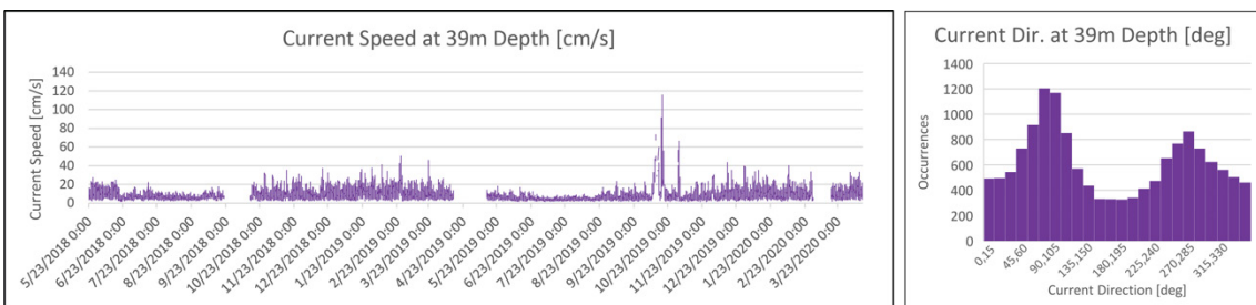
Figure 2-2: Current speed time series and associated current direction histogram spanning the data observation period for buoy SAP-1.
